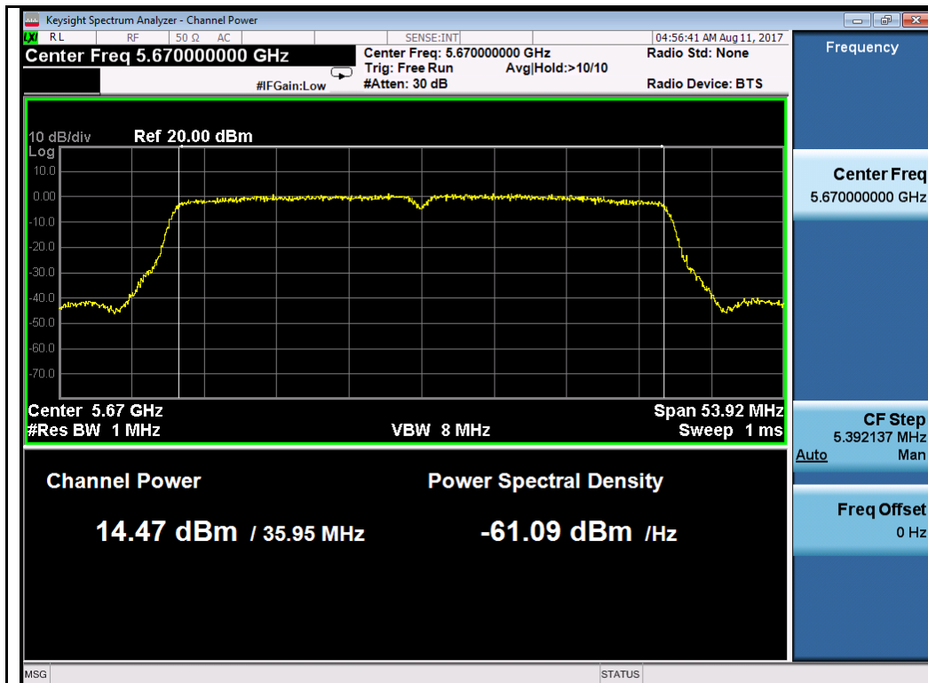
802.11n-HT40 5670M
