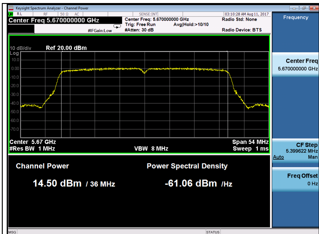
802.11n-HT40 5670M
