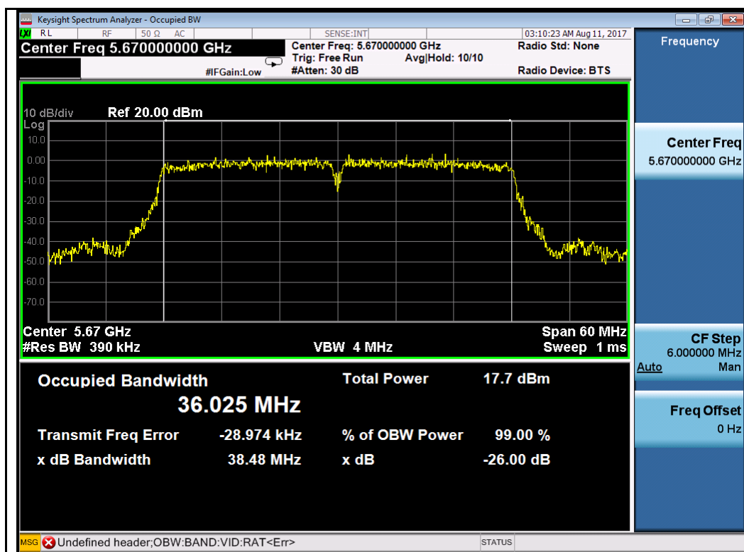
802.11n-HT40-5670MHz
