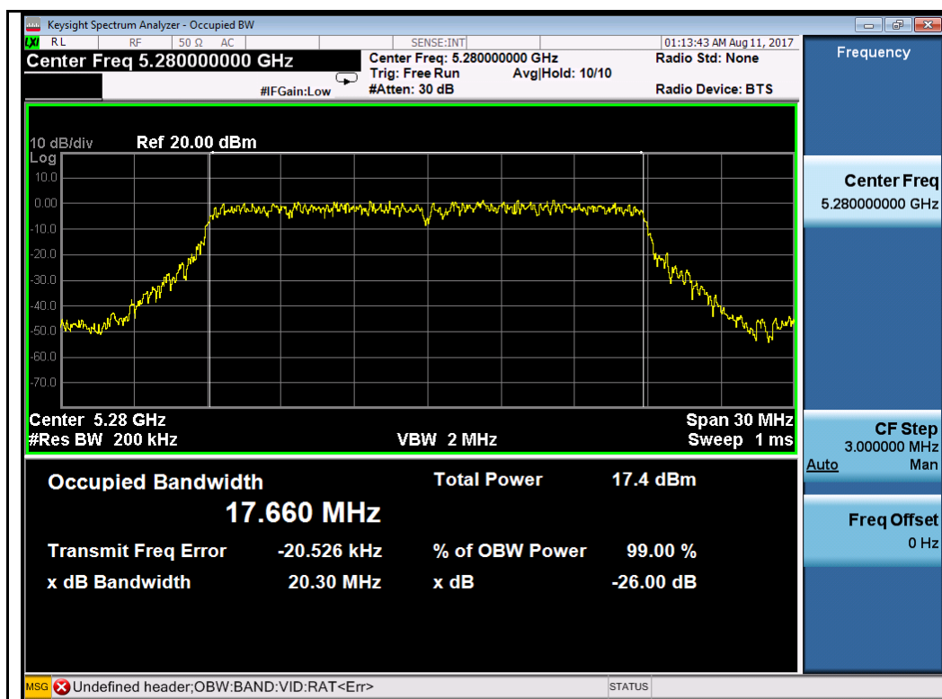
802.11n-HT20-5280MHz
