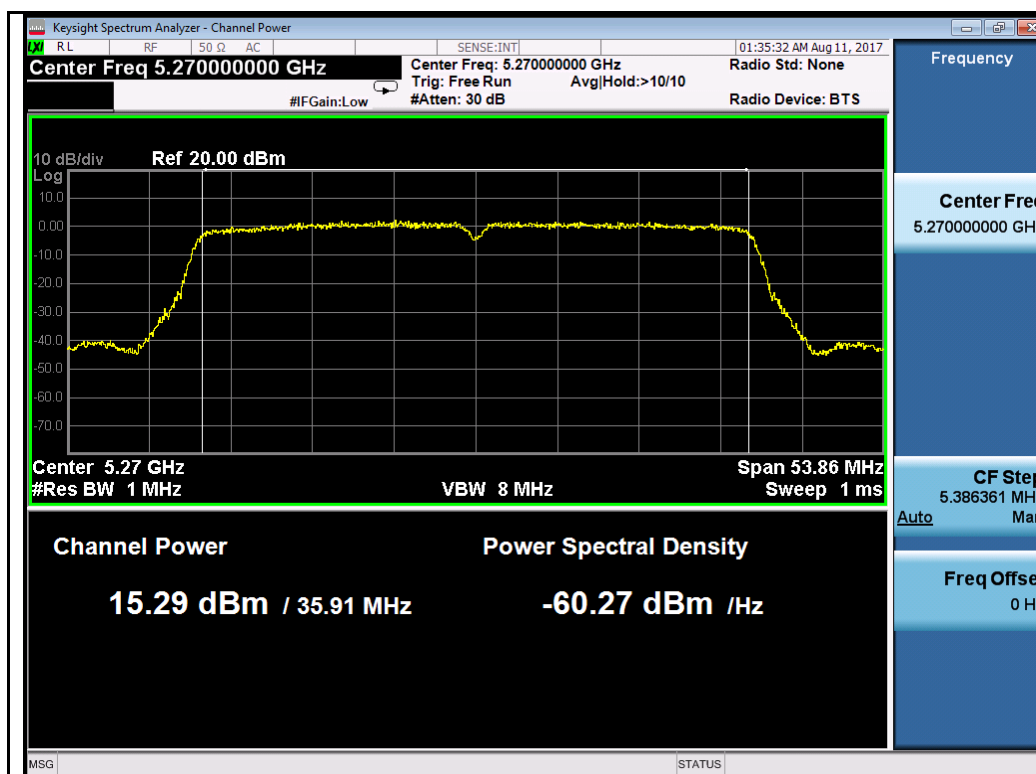
802.11n-HT40 5270M
