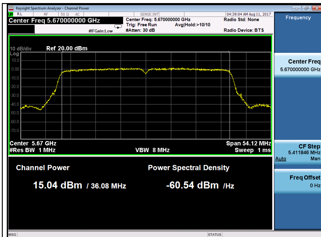
802.11n-HT40 5670M
