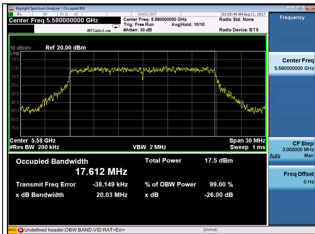
802.11n-HT20-5580MHz
