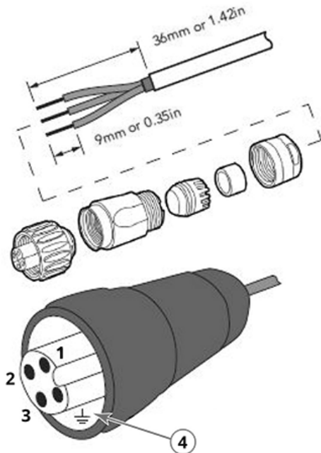
FIGURE 10 Assembling the AC power connector
