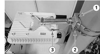
FIGURE 13 Attaching the security cable
