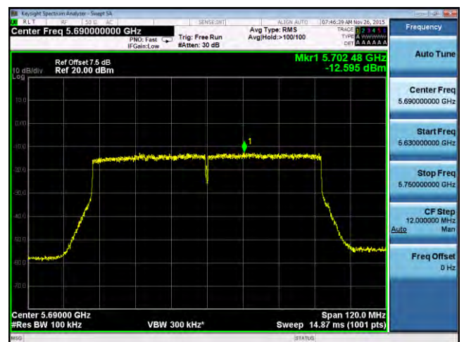
PSD-802.11ac-CROSS-5690M-chain4
