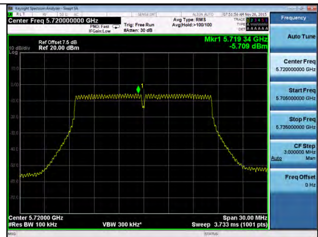
PSD-802.11a-CROSS-5720M-chain2
