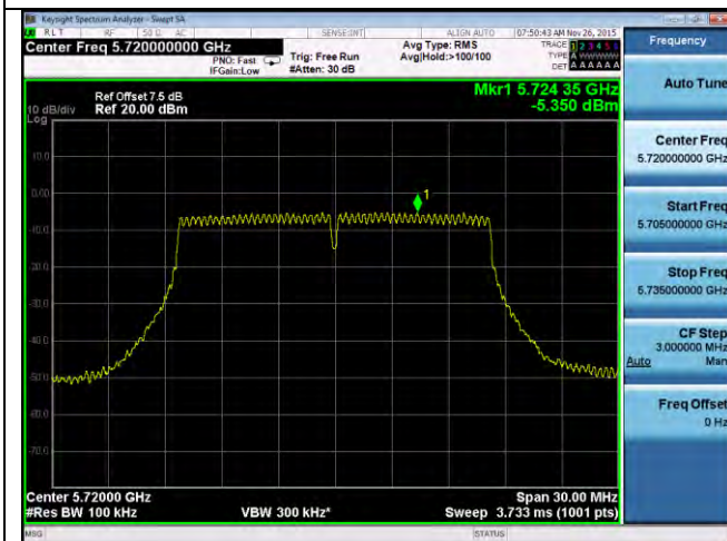
PSD-802.11a-CROSS-5720M-chain1
