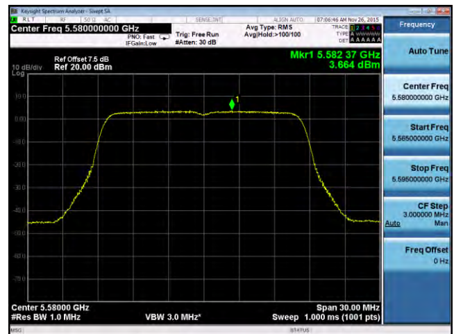
PSD-802.11a-5580M-chain2
