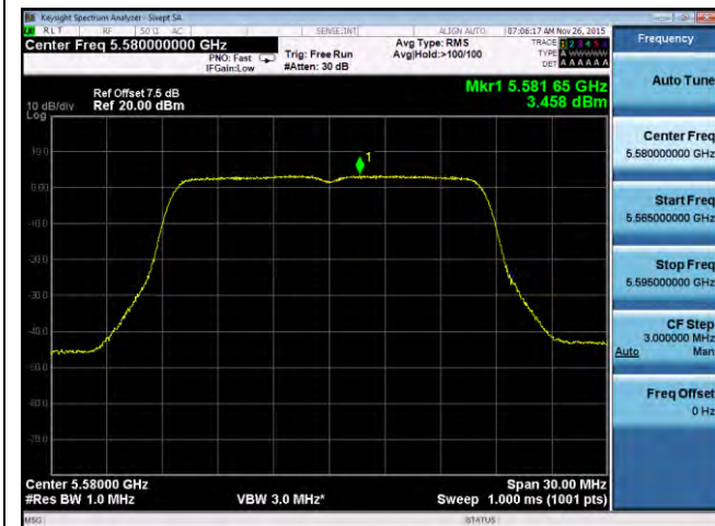
PSD-802.11a-5580M-chain1
