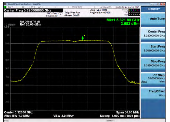
PSD-802.11a-5320M-chain4
