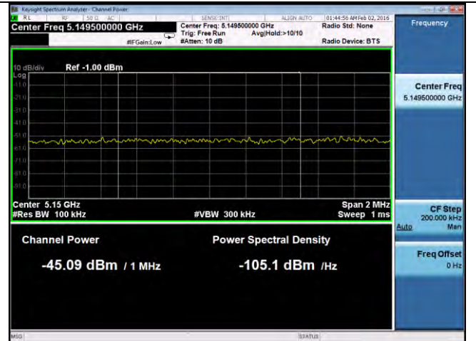
Band Edge-802.11a-5180M-chain2
