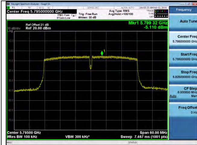
PSD-802.11n-40M-5795M-chain3
