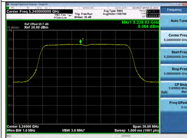
PSD-802.11n-20M-5240M-chain1
