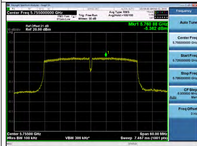
PSD-802.11n-40M-5755M-chain3
