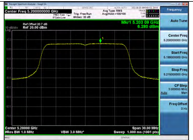
PSD-802.11a-5200M-chain4
