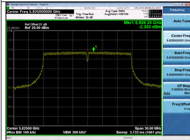
PSD-802.11n-20M-5825M-chain1
