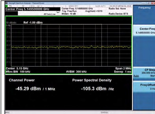
Band Edge-802.11a-5180M-chain1
