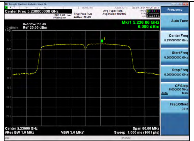
PSD-802.11n-40M-5230M-chain4
