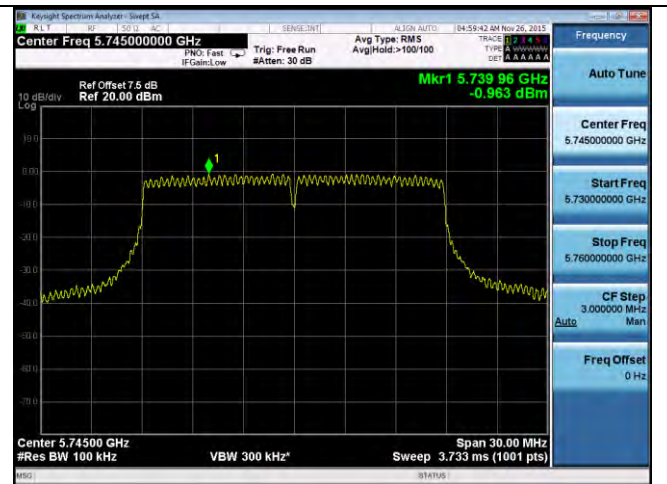
PSD-802.11n-20M-5745M-chain2
