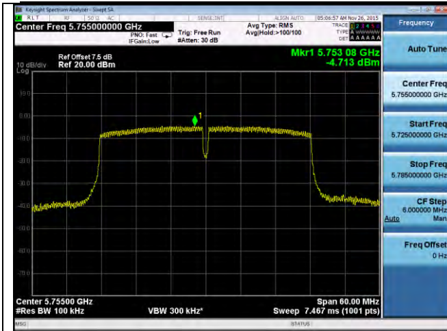
PSD-802.11n-40M-5755M-chain1
