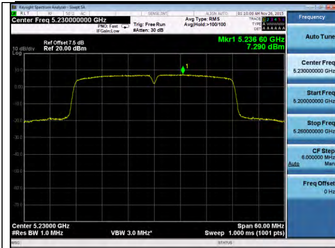
PSD-802.11n-40M-5230M-chain3
