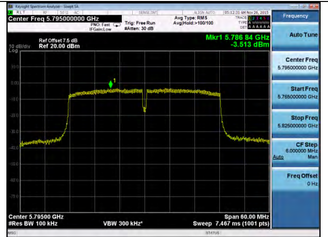
PSD-802.11n-40M-5795M-chain4
