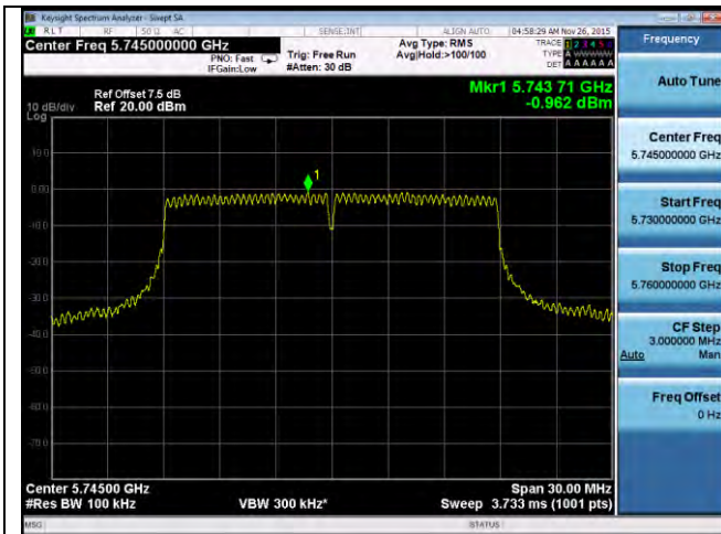
PSD-802.11n-20M-5745M-chain1
