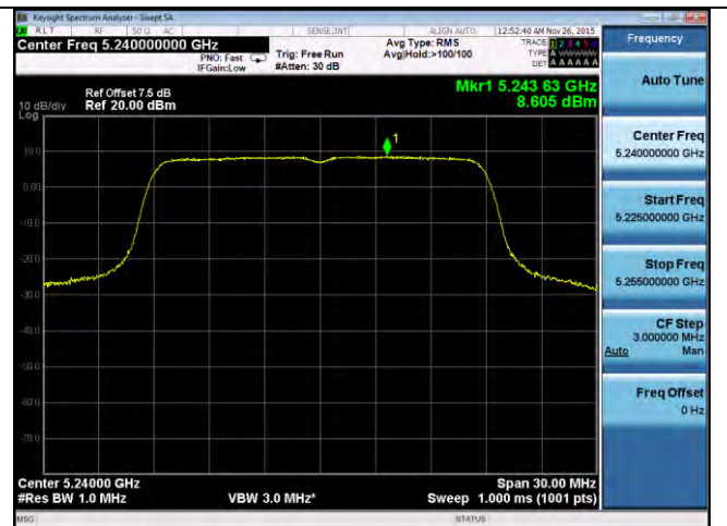
PSD-802.11n-20M-5240M-chain2
