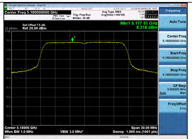
PSD-802.11a-5180M-chain4
