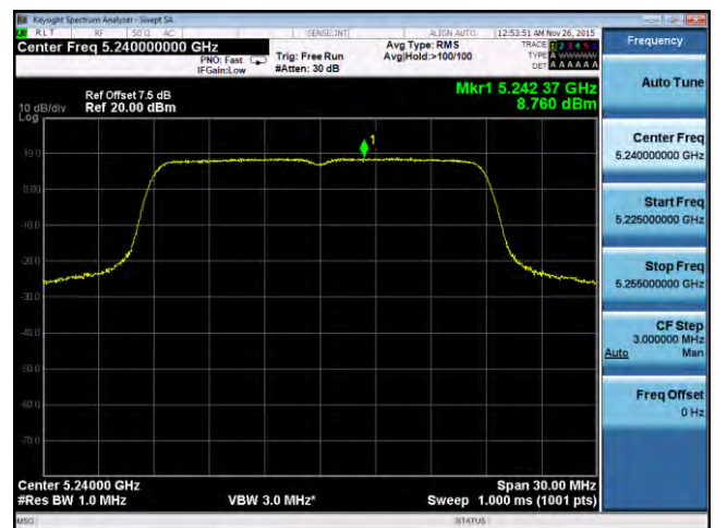
PSD-802.11n-20M-5240M-chain4
