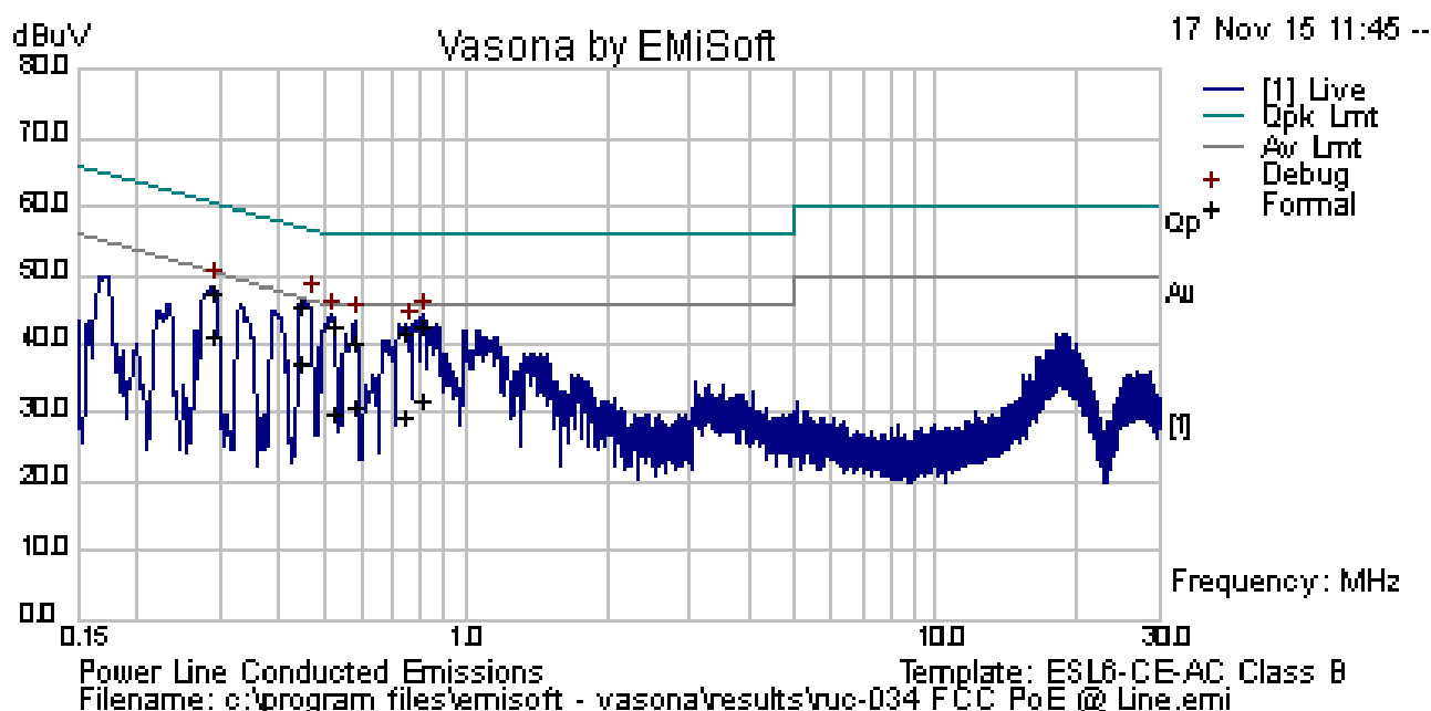
Live Line Plot at 120Vac, 60Hz
