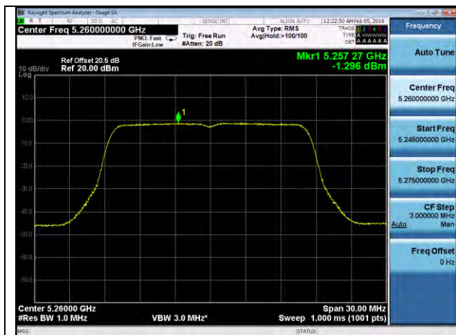
PSD-802.11a-5260M-chain1
