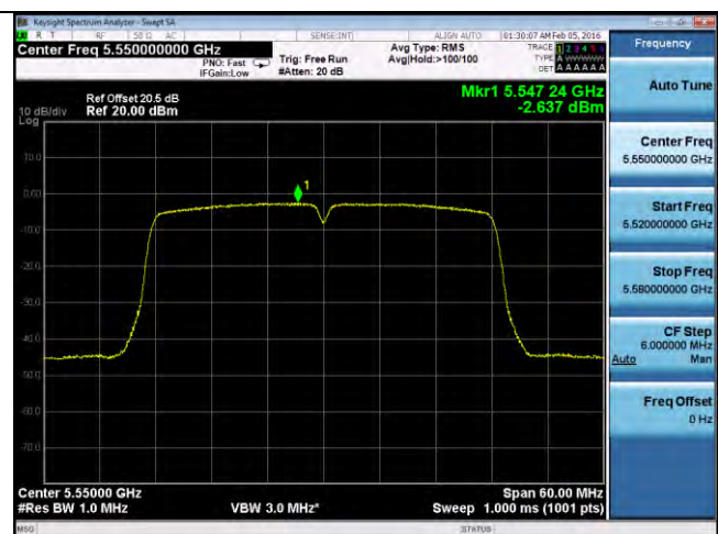
PSD-802.11n-40M-5550M-chain4
