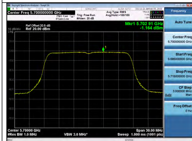
PSD-802.11a-5700M-chain1
