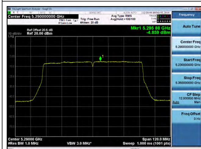
PSD-802.11ac-80M-5290M-chain3
