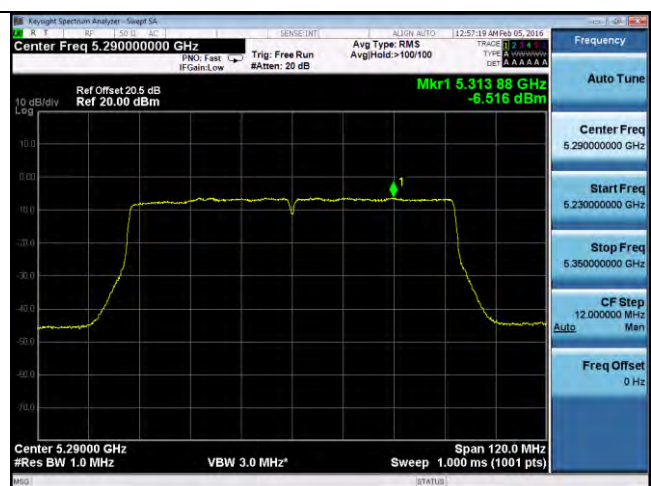
PSD-802.11ac-80M-5290M-chain2
