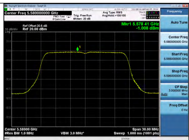
PSD-802.11a-5580M-chain4
