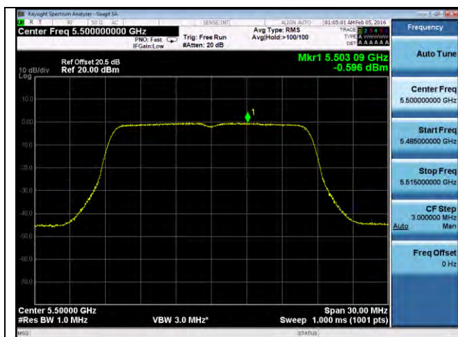
PSD-802.11a-5500M-chain1
