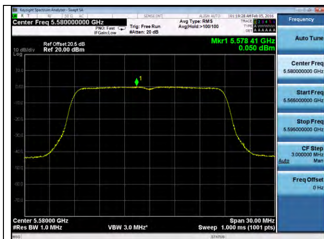
PSD-802.11n-20M-5580M-chain3
