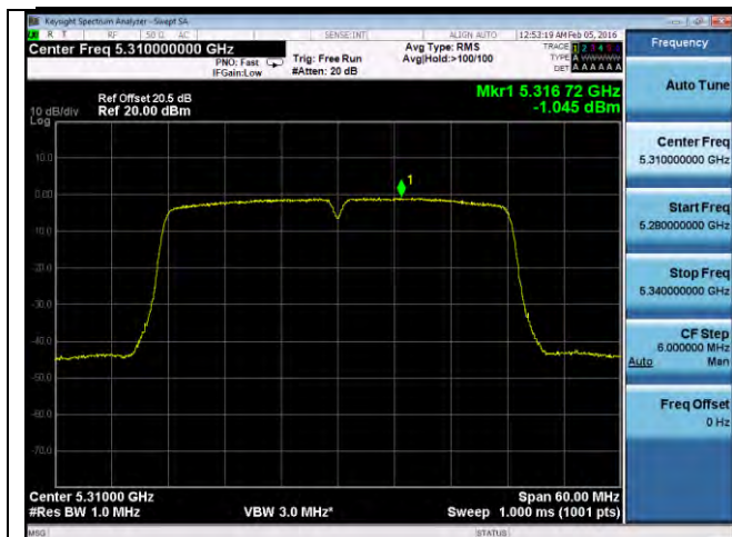
PSD-802.11n-40M-5310M-chain3
