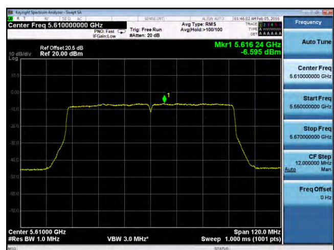
PSD-802.11ac-80M-5610M-chain2
