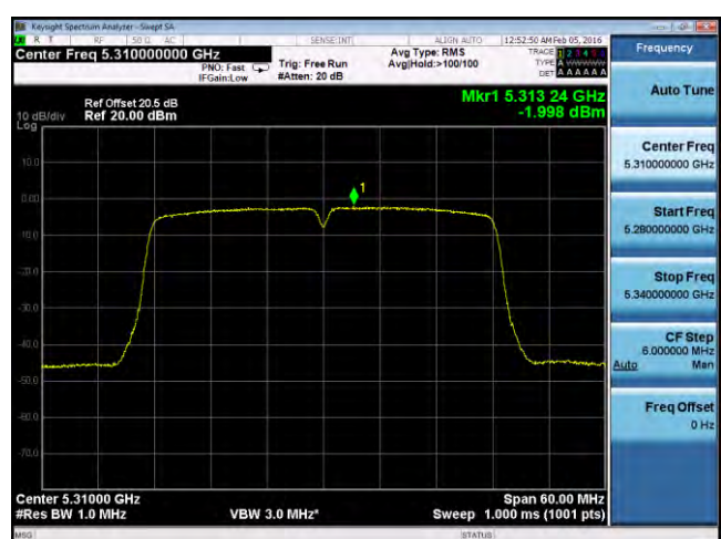
PSD-802.11n-40M-5310M-chain2
