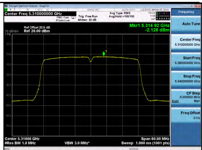
PSD-802.11n-40M-5310M-chain4
