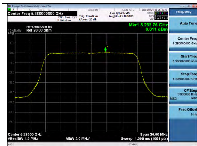
PSD-802.11n-20M-5280M-chain3
