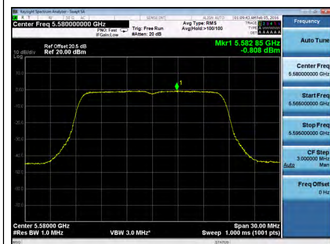
PSD-802.11a-5580M-chain1
