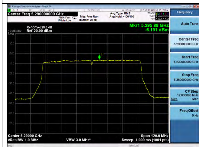
PSD-802.11ac-80M-5290M-chain1
