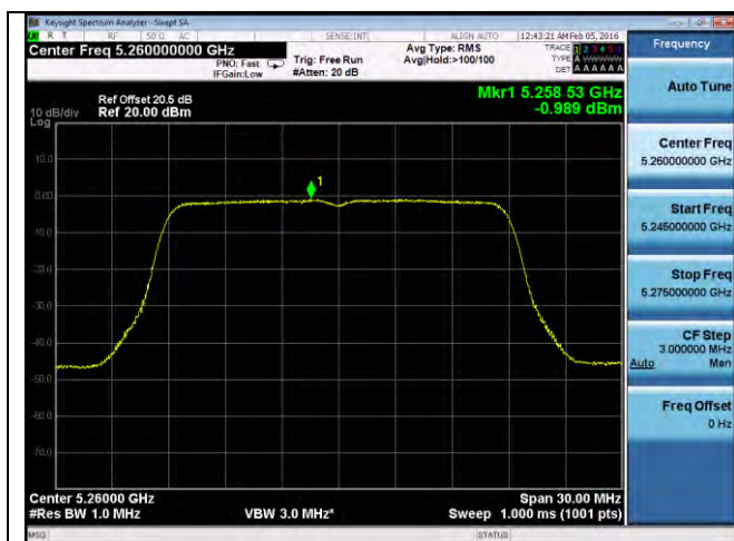
PSD-802.11n-20M-5260M-chain1
