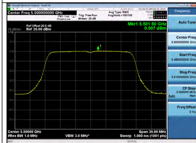
PSD-802.11a-5500M-chain3
