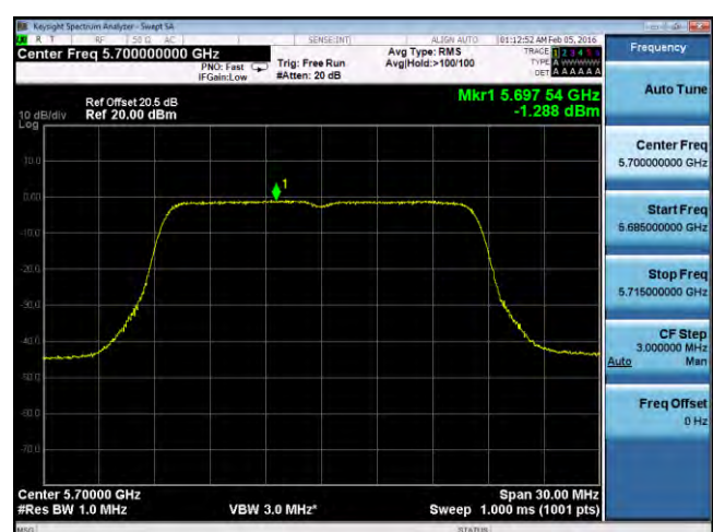
PSD-802.11a-5700M-chain4
