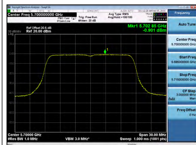
PSD-802.11a-5700M-chain3
