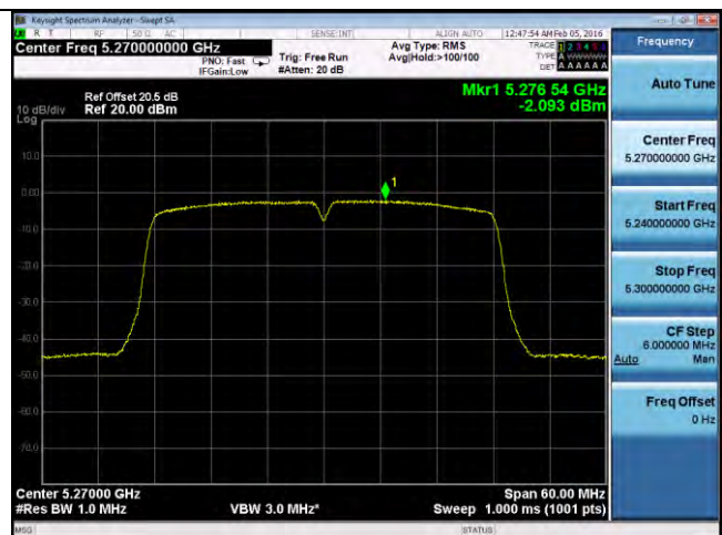
PSD-802.11n-40M-5270M-chain4
