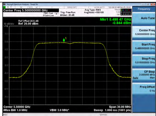
PSD-802.11a-5500M-chain4
