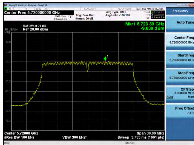
PSD-802.11n-20M-CROSS-5720M-chain2
