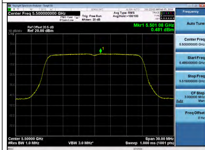
PSD-802.11n-20M-5500M-chain3
