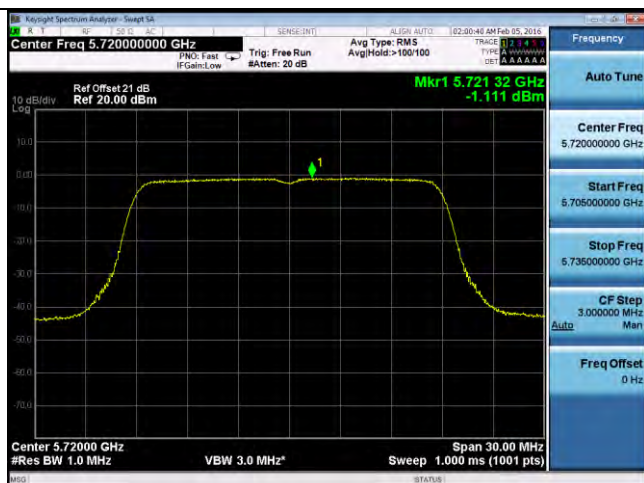
PSD-802.11n-20M-CROSS-5720M-chain1
