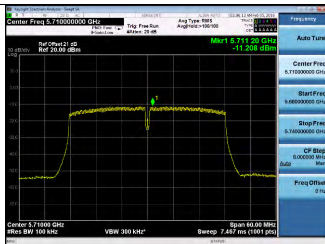
PSD-802.11n-40M-CROSS-5710M-chain4
