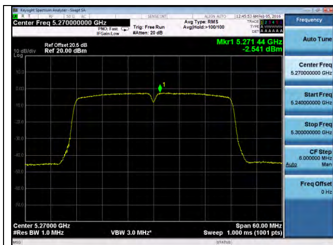
PSD-802.11n-40M-5270M-chain1
