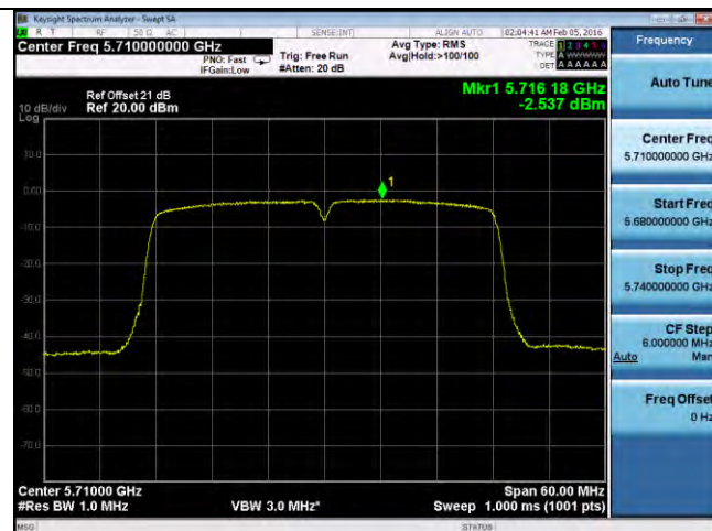
PSD-802.11n-40M-CROSS-5710M-chain2
