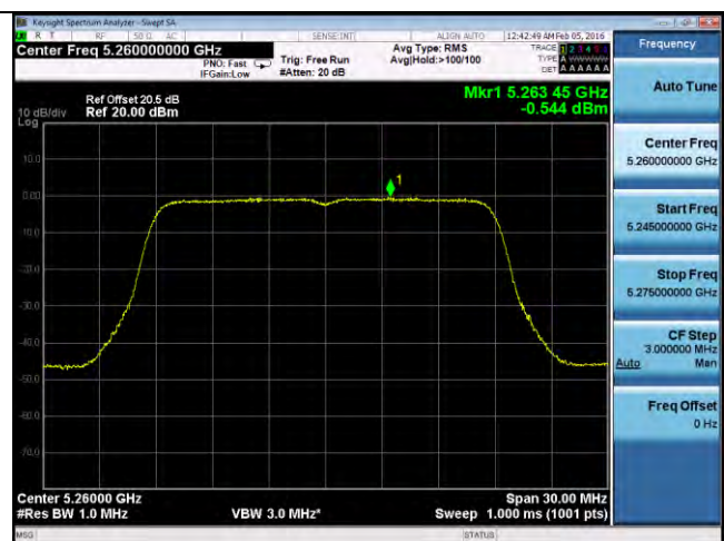
PSD-802.11n-20M-5260M-chain2
