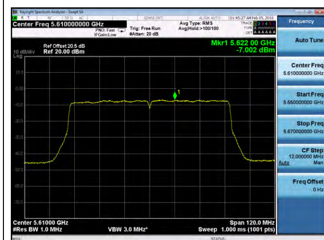
PSD-802.11ac-80M-5610M-chain1
