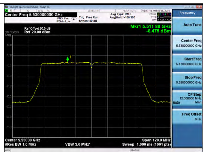
PSD-802.11ac-80M-5530M-chain4
