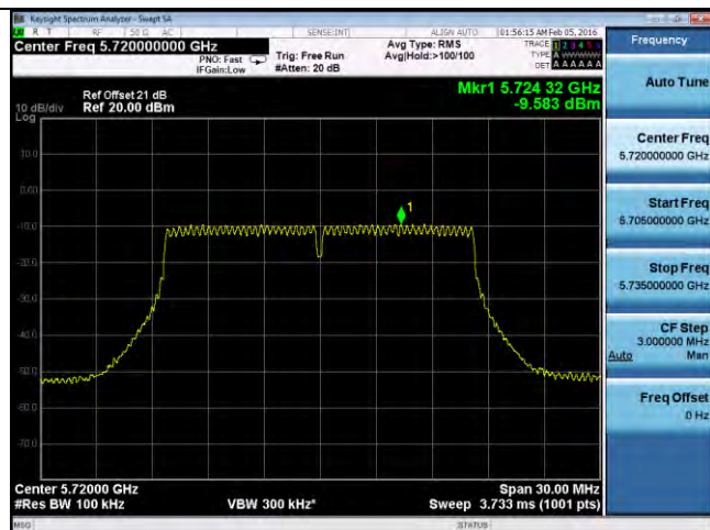
PSD-802.11a-CROSS-5720M-chain3
