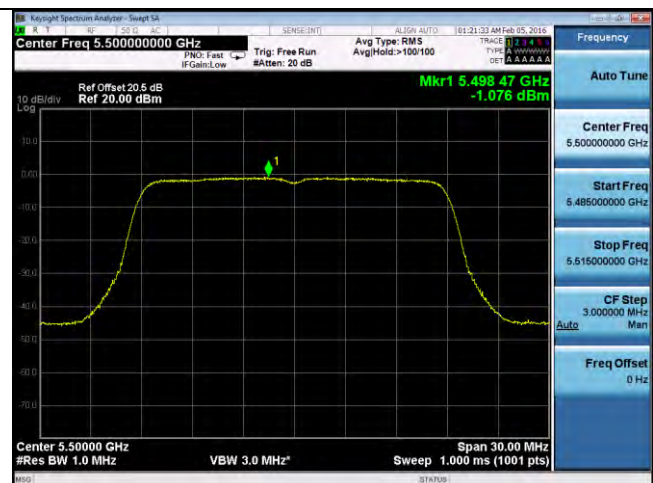
PSD-802.11n-20M-5500M-chain4
