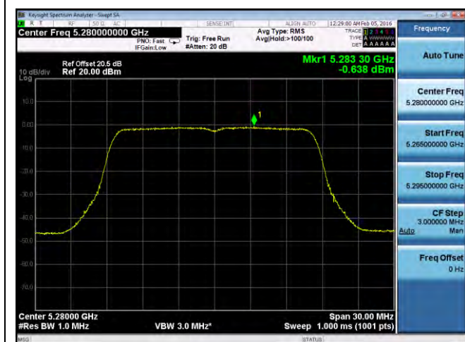
PSD-802.11a-5280M-chain1
