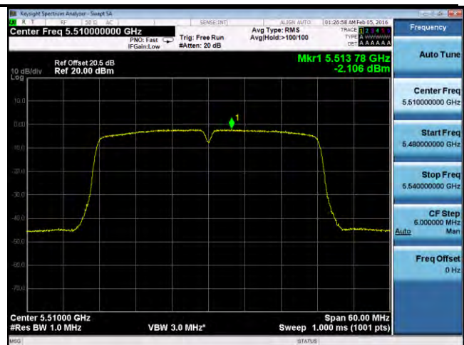
PSD-802.11n-40M-5510M-chain2
