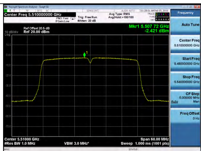
PSD-802.11n-40M-5510M-chain4
