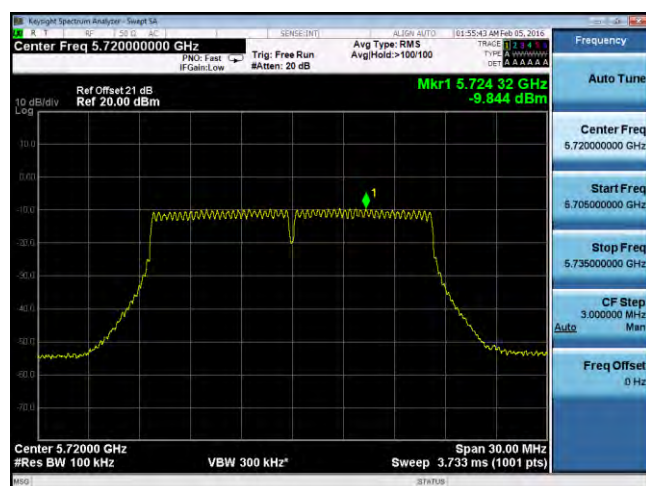
PSD-802.11a-CROSS-5720M-chain2
