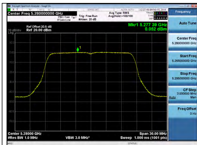
PSD-802.11a-5280M-chain3
