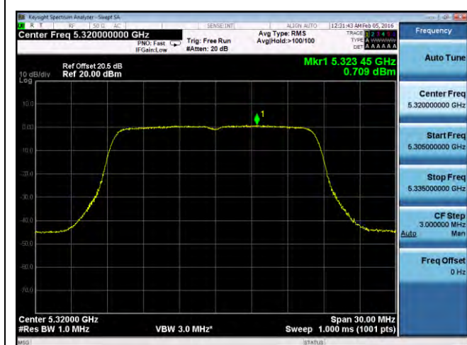
PSD-802.11a-5320M-chain3
