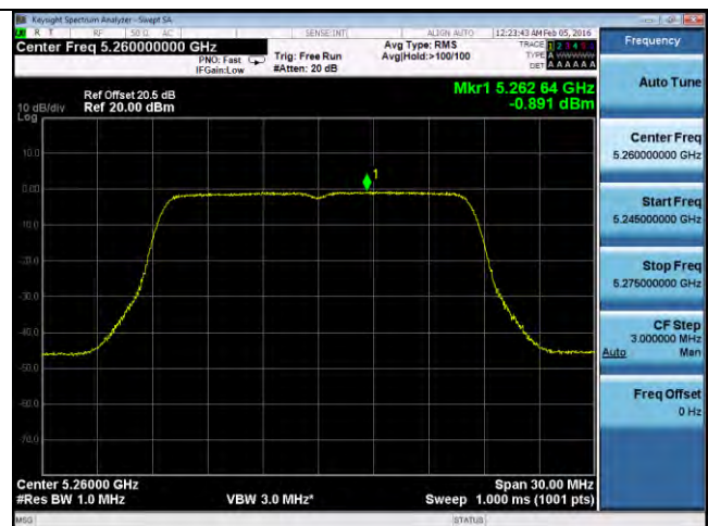
PSD-802.11a-5260M-chain2
