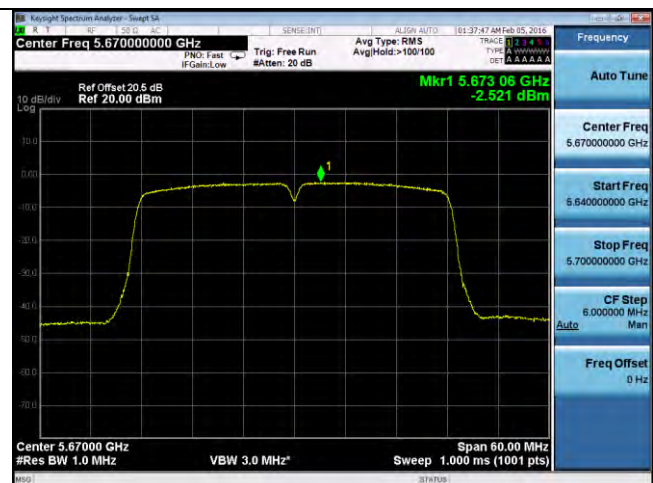
PSD-802.11n-40M-5670M-chain2
