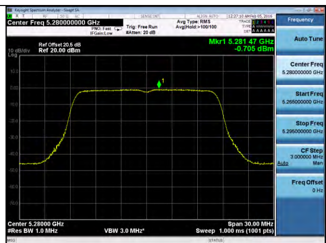
PSD-802.11a-5280M-chain4
