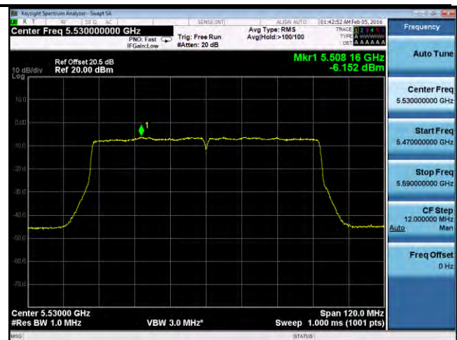
PSD-802.11ac-80M-5530M-chain2
