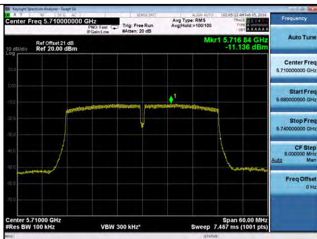
PSD-802.11n-40M-CROSS-5710M-chain3
