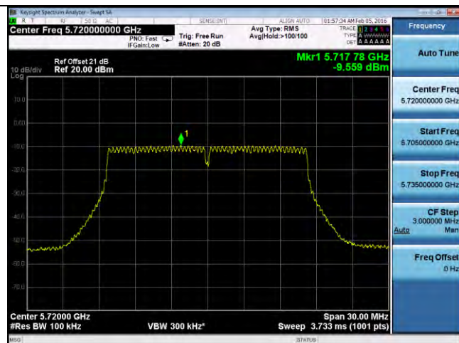
PSD-802.11a-CROSS-5720M-chain4
