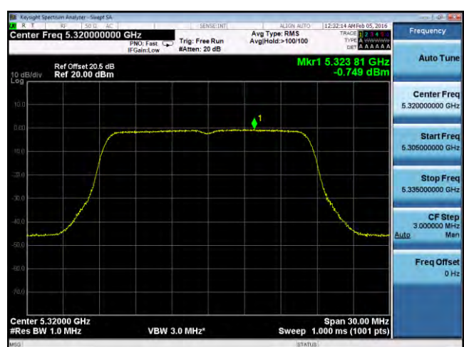
PSD-802.11a-5320M-chain4
