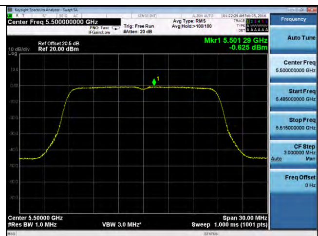
PSD-802.11n-20M-5500M-chain2
