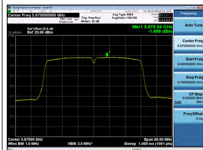
PSD-802.11n-40M-5670M-chain3
