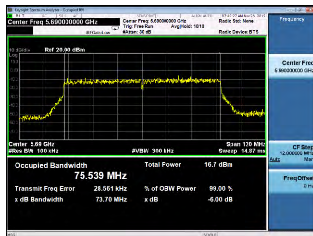
6dB BW -802.11ac CROSS 5690MHz
