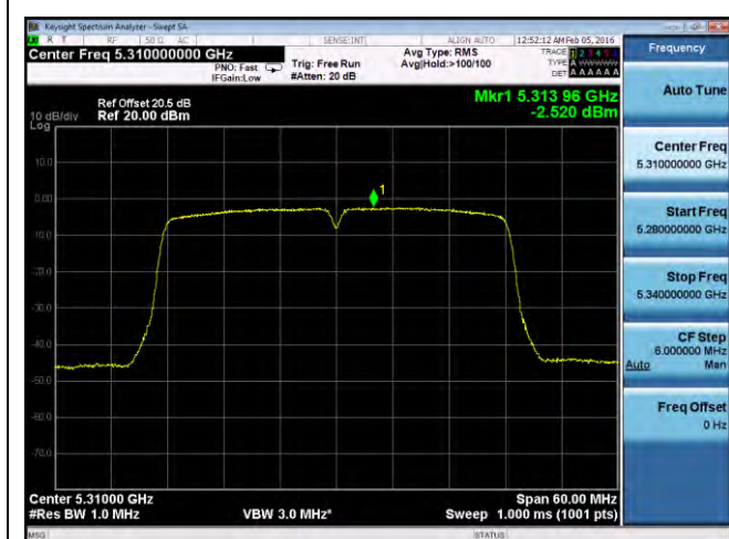
PSD-802.11n-40M-5310M-chain1
