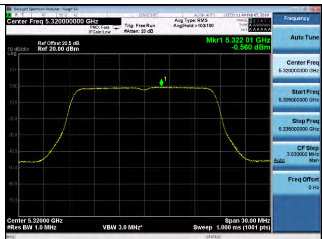
PSD-802.11a-5320M-chain2
