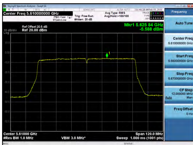
PSD-802.11ac-80M-5610M-chain3
