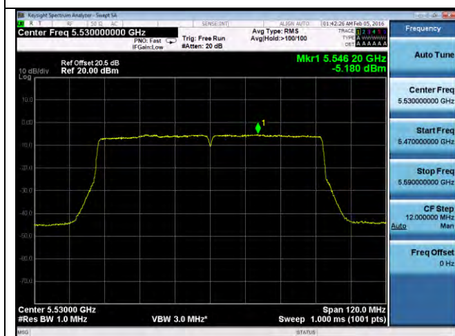
PSD-802.11ac-80M-5530M-chain3
