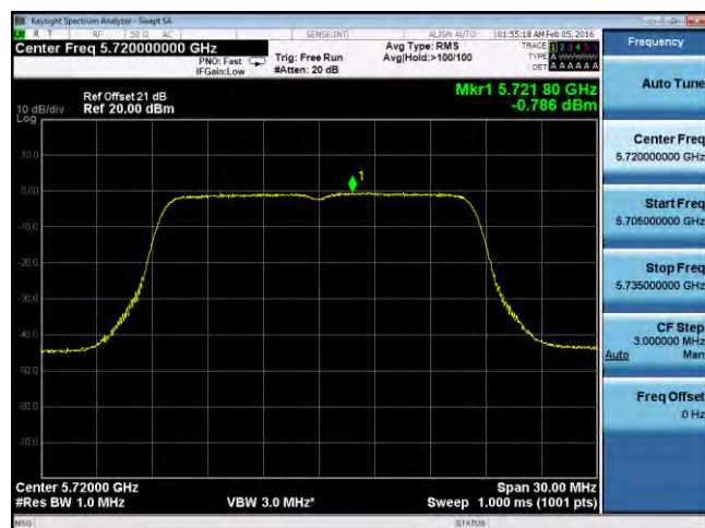
PSD-802.11a-CROSS-5720M-chain2
