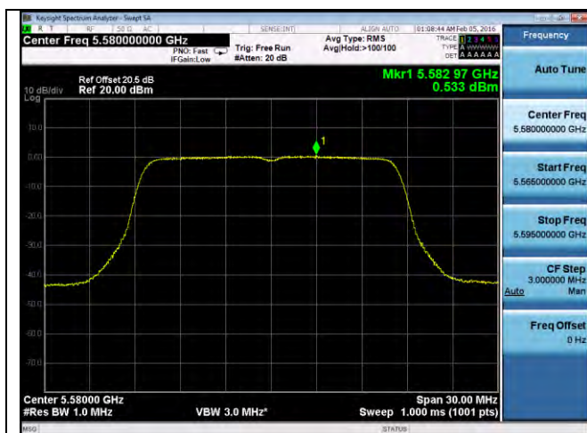
PSD-802.11a-5580M-chain3
