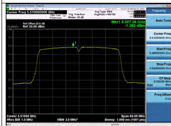
PSD-802.11n-40M-5510M-chain3
