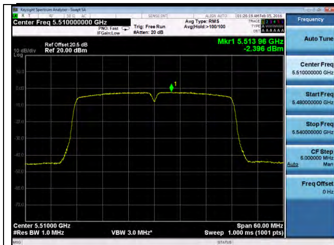
PSD-802.11n-40M-5510M-chain1
