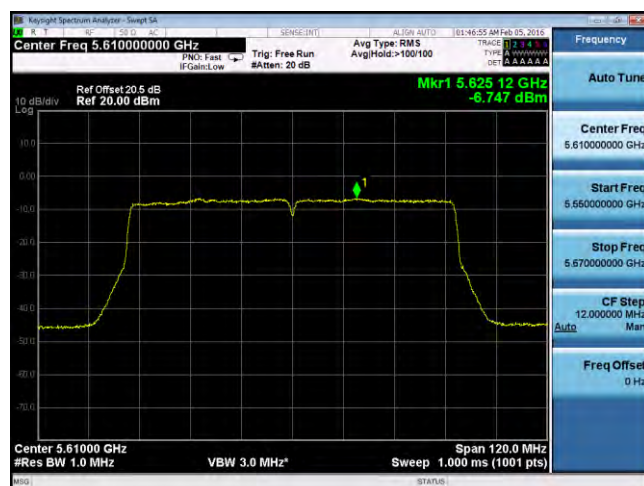
PSD-802.11ac-80M-5610M-chain4
