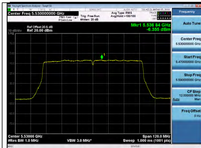
PSD-802.11ac-80M-5530M-chain1
