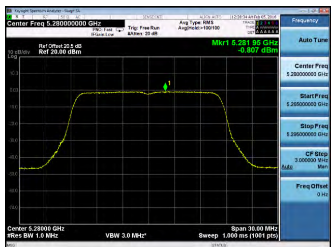
PSD-802.11a-5280M-chain2
