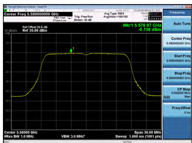
PSD-802.11a-5580M-chain2
