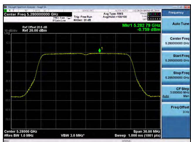
PSD-802.11n-20M-5280M-chain2
