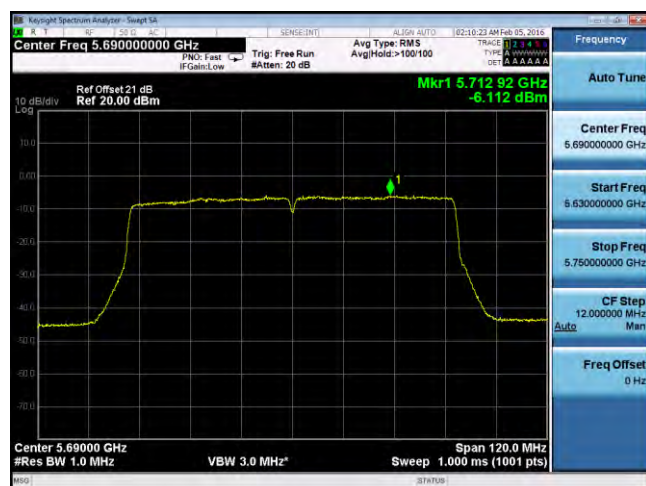
PSD-802.11ac-CROSS-5690M-chain2
