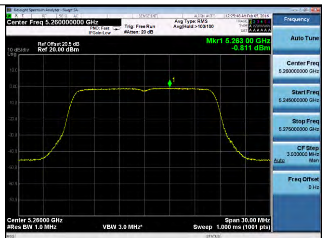
PSD-802.11a-5260M-chain4
