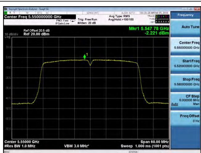
PSD-802.11n-40M-5550M-chain2
