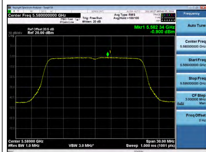
PSD-802.11n-20M-5580M-chain1
