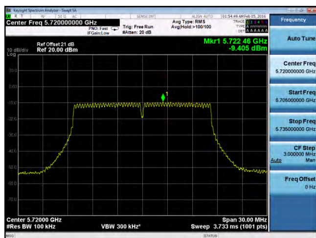
PSD-802.11a-CROSS-5720M-chain1
