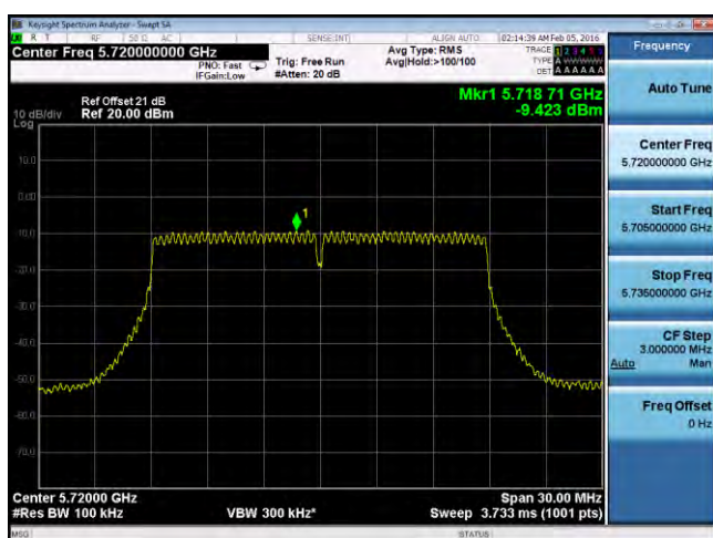
PSD-802.11n-20M-CROSS-5720M-chain3
