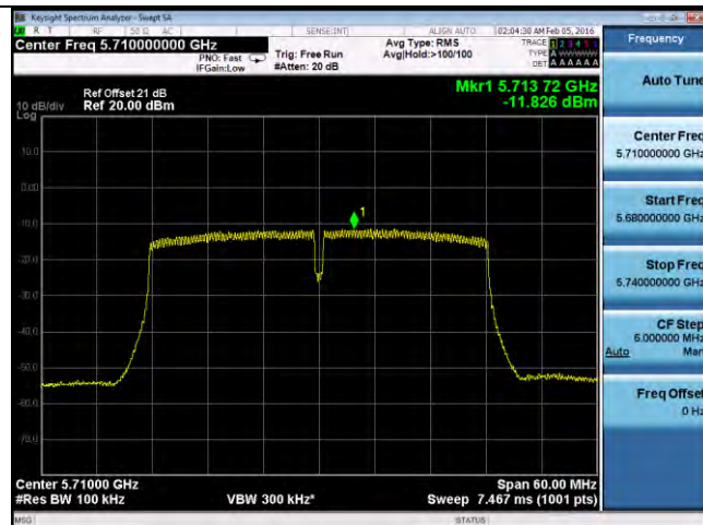
PSD-802.11n-40M-CROSS-5710M-chain2
