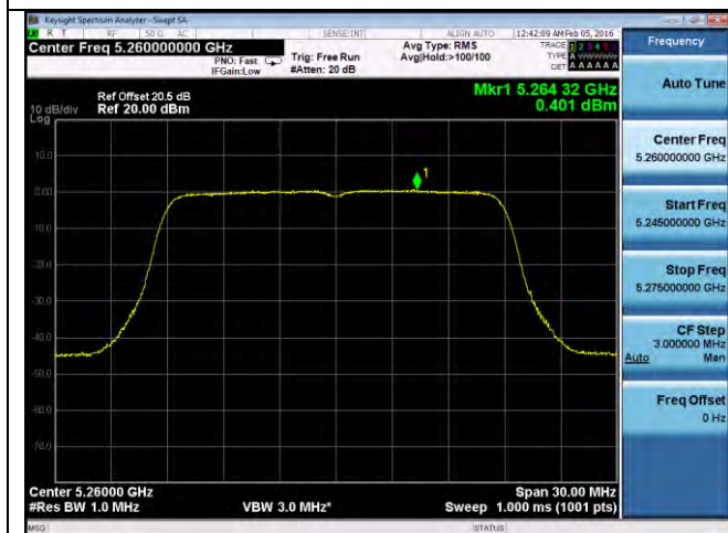
PSD-802.11n-20M-5260M-chain3
