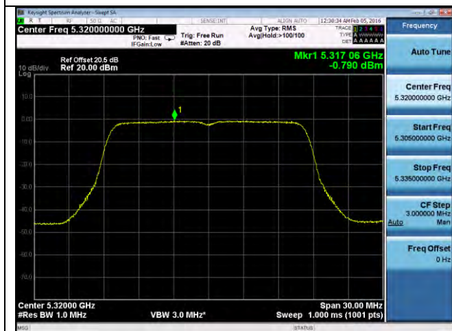
PSD-802.11a-5320M-chain1
