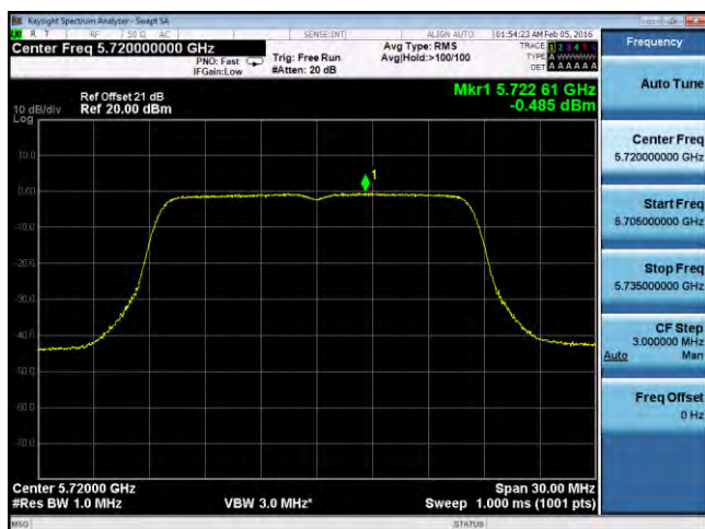
PSD-802.11a-CROSS-5720M-chain1
