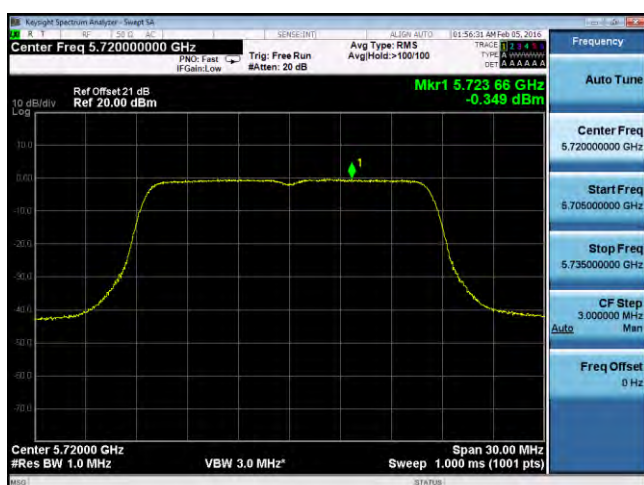
PSD-802.11a-CROSS-5720M-chain3
