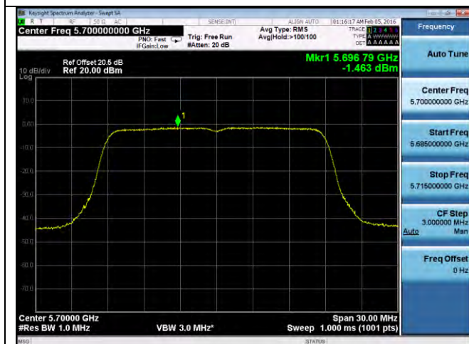
PSD-802.11n-20M-5700M-chain1
