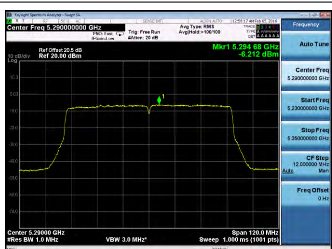
PSD-802.11ac-80M-5290M-chain4
