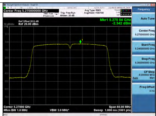
PSD-802.11n-40M-5270M-chain2
