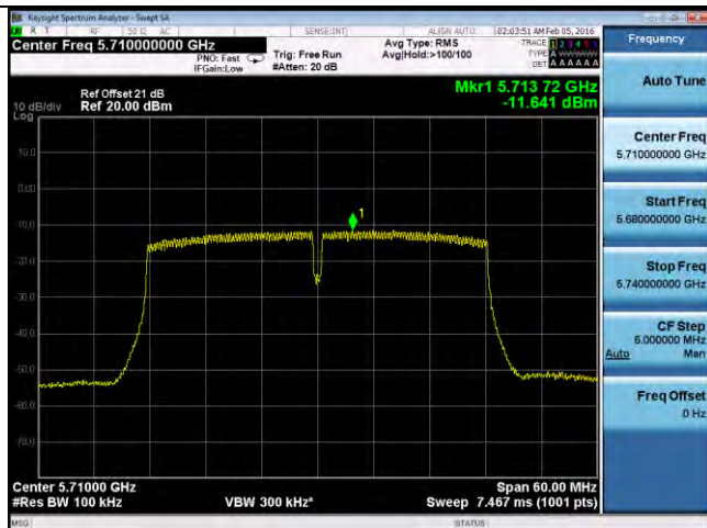
PSD-802.11n-40M-CROSS-5710M-chain1
