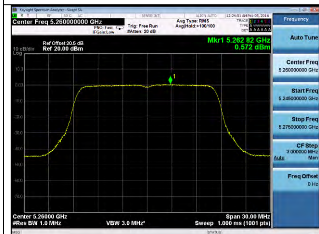
PSD-802.11a-5260M-chain3
