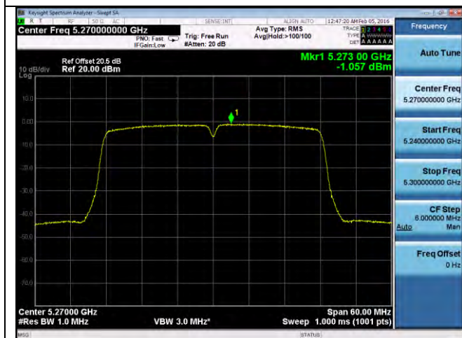
PSD-802.11n-40M-5270M-chain3
