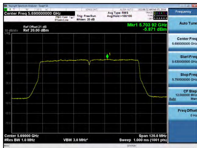
PSD-802.11ac-CROSS-5690M-chain4
