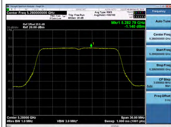
PSD-802.11n-20M-5280M-chain1
