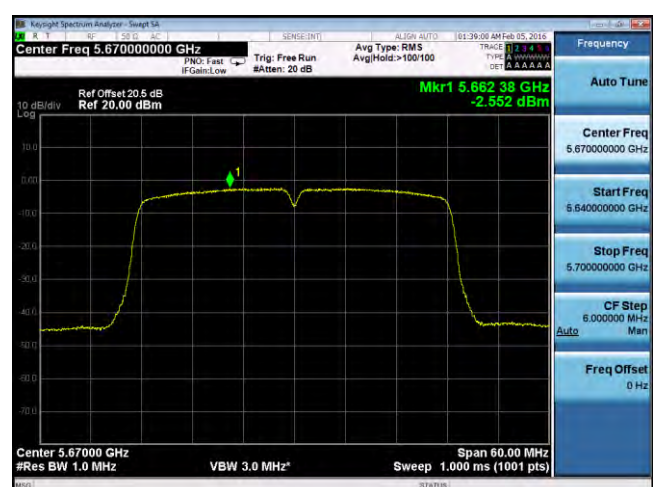
PSD-802.11n-40M-5670M-chain4
