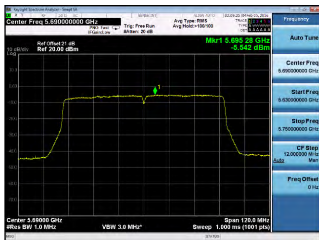
PSD-802.11ac-CROSS-5690M-chain3
