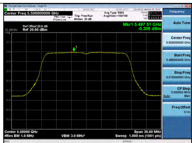
PSD-802.11a-5500M-chain2
