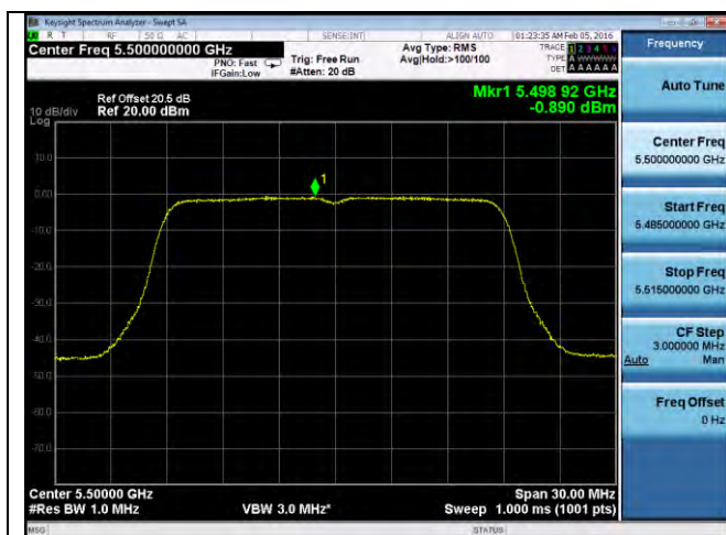
PSD-802.11n-20M-5500M-chain1
