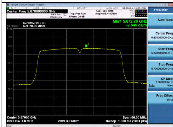
PSD-802.11n-40M-5670M-chain1
