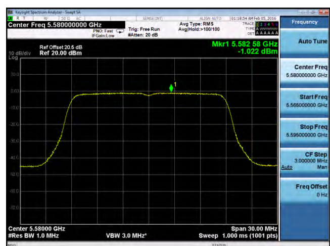
PSD-802.11n-20M-5580M-chain2
