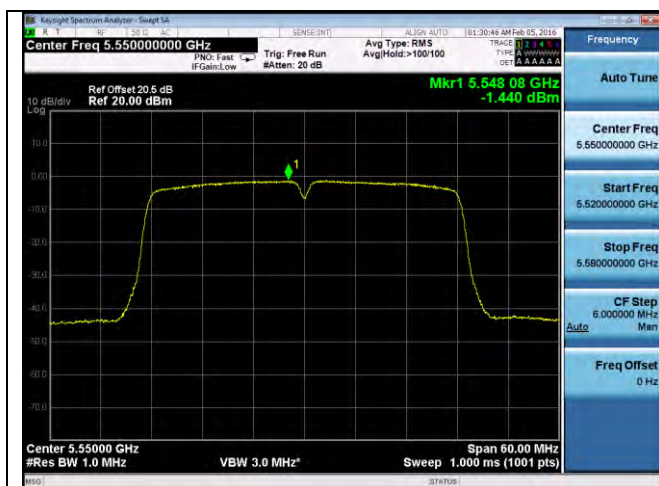
PSD-802.11n-40M-5550M-chain3
