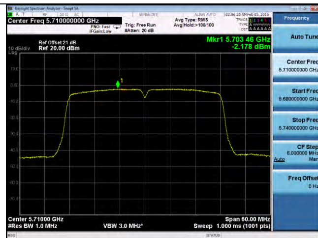
PSD-802.11n-40M-CROSS-5710M-chain4
