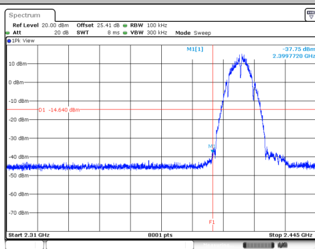
Channel 01 Plot
