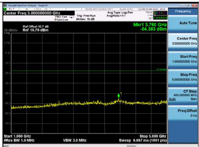
CUE-802.11ac-80-5610M-chain2(1GHz-5GHz)
