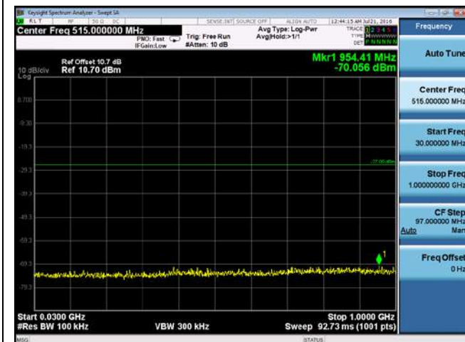
CUE-802.11ac-80-5530M-chain2(30MHz-1GHz)
