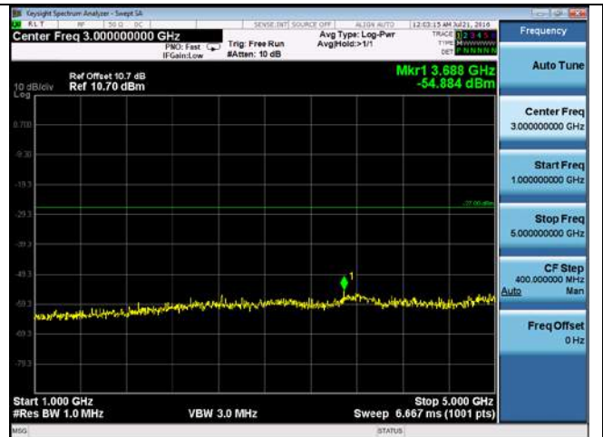
CUE-802.11ac-80-5530M-chain1(1GHz-5GHz)
