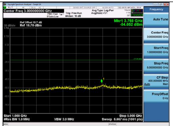
CUE-802.11ac-80-5530M chain4(1GHz-5GHz)
