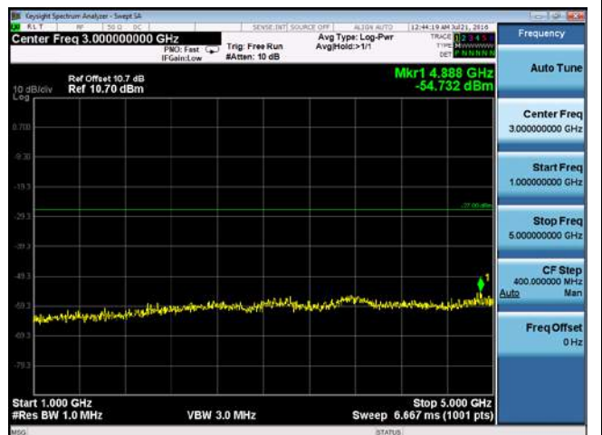
CUE-802.11ac-80-5530M-chain2(1GHz-5GHz)
