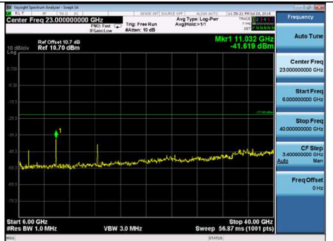
CUE-802.11n-40-5510M-chain1(6GHz-40GHz)
