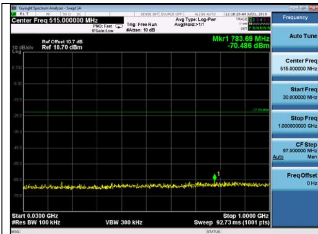
CUE-802.11a-5720M -chain2(30MHz-1GHz)
