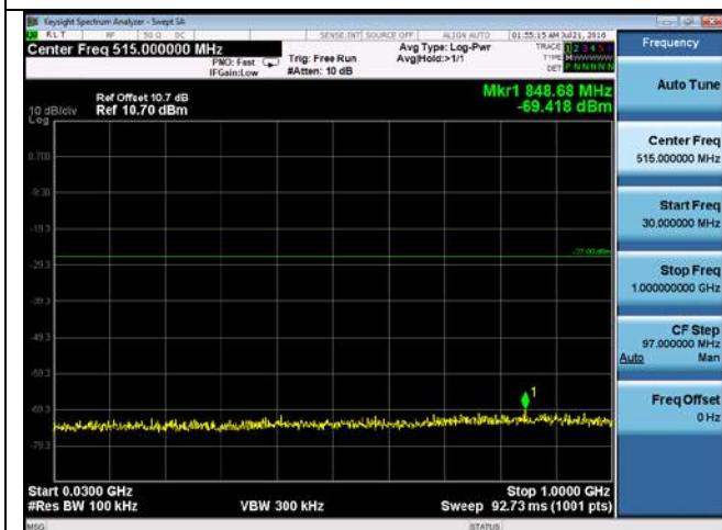
CUE-802.11a-5720M -chain4(30MHz-1GHz)
