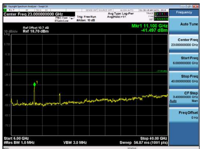
CUE-802.11ac-80-5530M -chain3(6GHz-40GHz)
