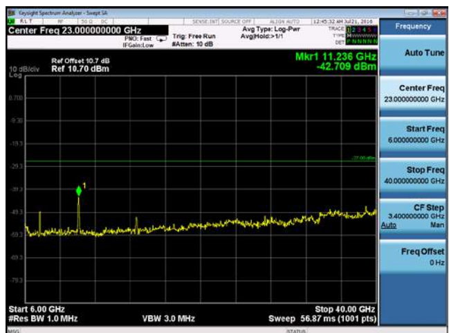
CUE-802.11ac-80-5610M-chain2(6GHz-40GHz)
