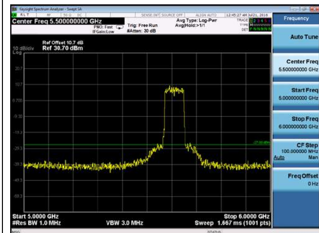
CUE-802.11ac-80-5610M-chain2(5GHz-6GHz)
