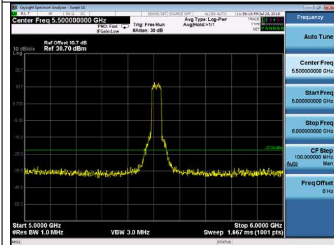
CUE-802.11n-40-5510M-chain1(5GHz-6GHz)
