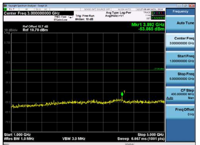
CUE-802.11n20-5720M -chain2(1GHz-5GHz)
