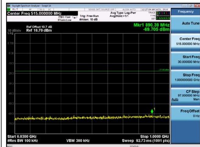
CUE-802.11n20-5720M -chain2(30MHz-1GHz)
