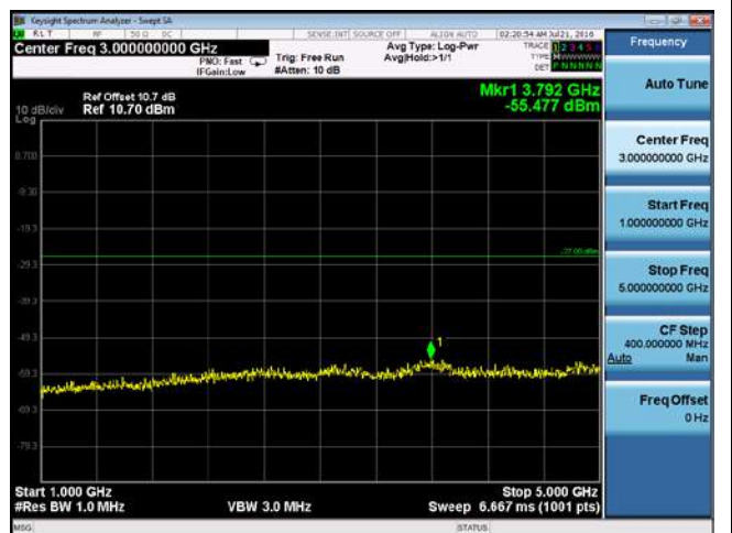
CUE-802.11ac-80-5610M-chain4(1GHz-5GHz)
