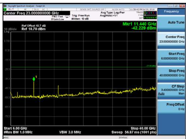
CUE-802.11n40-5710M -chain1 (6GHz-40GHz)
