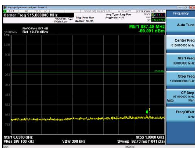
CUE-802.11n40-5710M -chain2(30MHz-1GHz)
