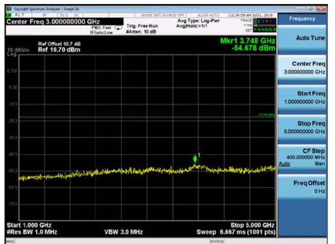
CUE-802.11n-40-5510M-chain2(1GHz-5GHz)
