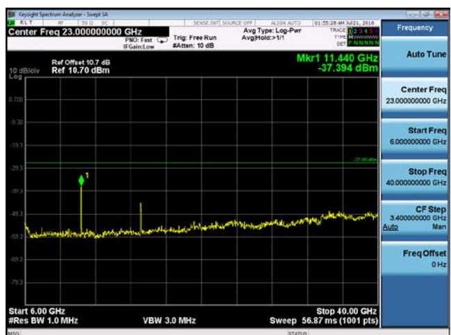
CUE-802.11a-5720M -chain4 (6GHz-40GHz)
