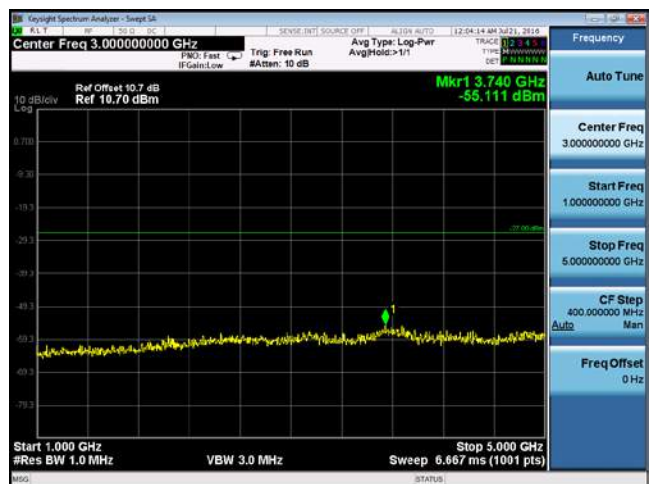
CUE-802.11ac-80-5610M-chain1(1GHz-5GHz)
