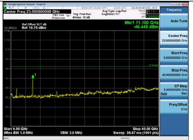
CUE-802.11ac-80-5530M-chain4(6GHz-40GHz)
