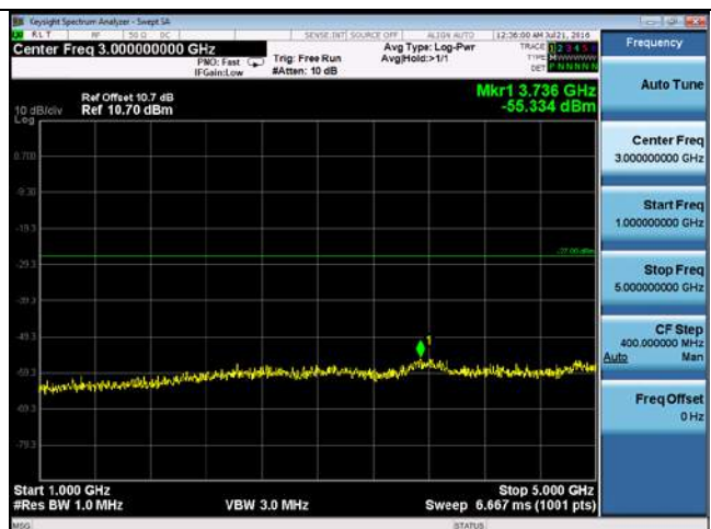
CUE-802.11n-40-5550M-chain2(1GHz-5GHz)
