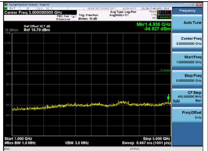
CUE-802.11n-40-5550M-chain3(1GHz-5GHz)
