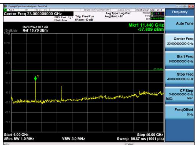
CUE-802.11a-5720M -chain3 (6GHz-40GHz)
