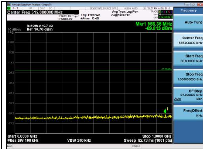
CUE-802.11n-40-5510M-chain1(30MHz-1GHz)
