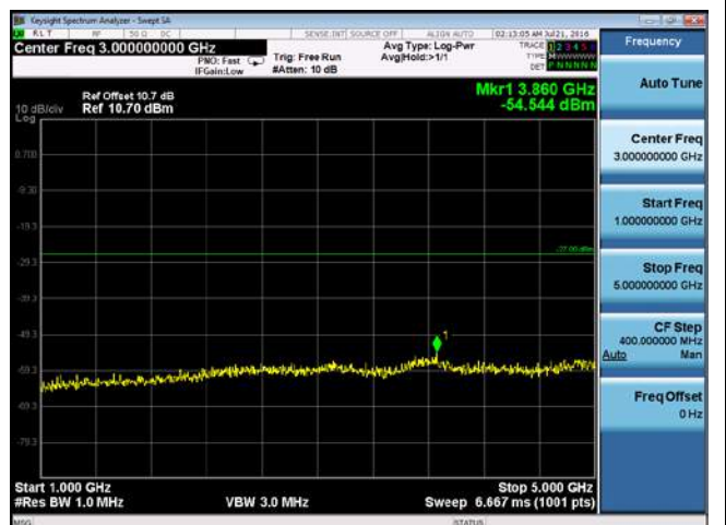
CUE-802.11n-40-5550M-chain4(1GHz-5GHz)
