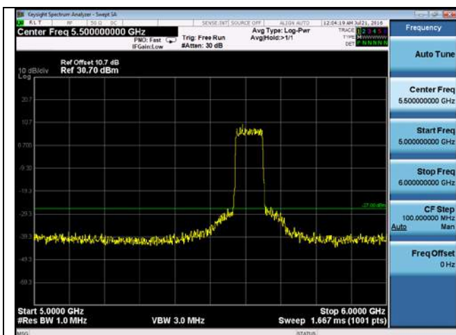
CUE-802.11ac-80-5610M-chain1(5GHz-6GHz)
