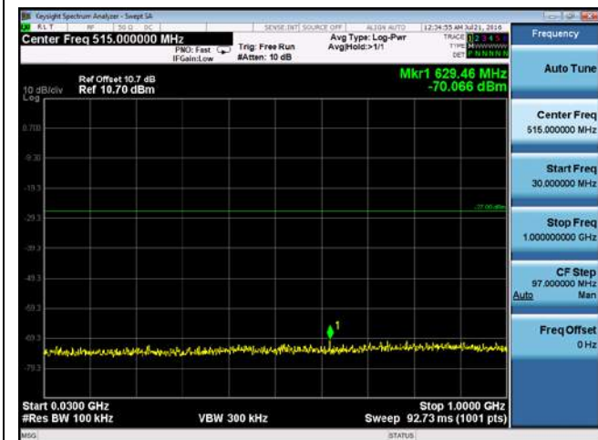
CUE-802.11n-40-5510M-chain2(30MHz-1GHz)
