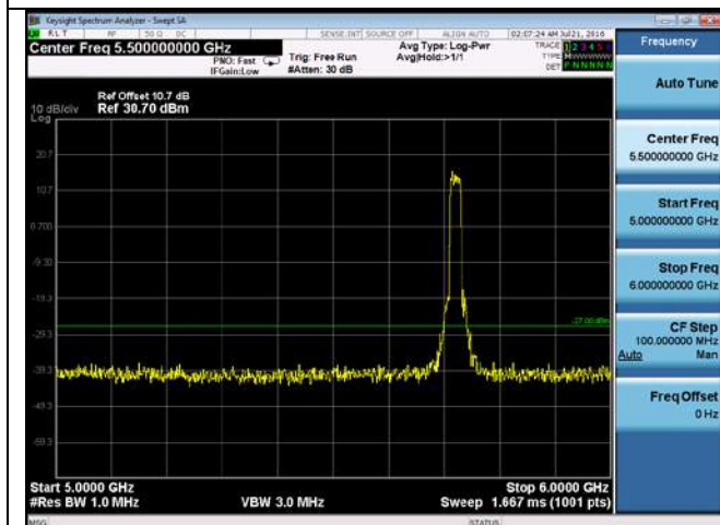
CUE-802.11n20-5720M -chain4(5GHz-6GHz)
