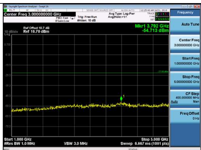
CUE-802.11n-20-5700M -chain 2(1GHz-5GHz)
