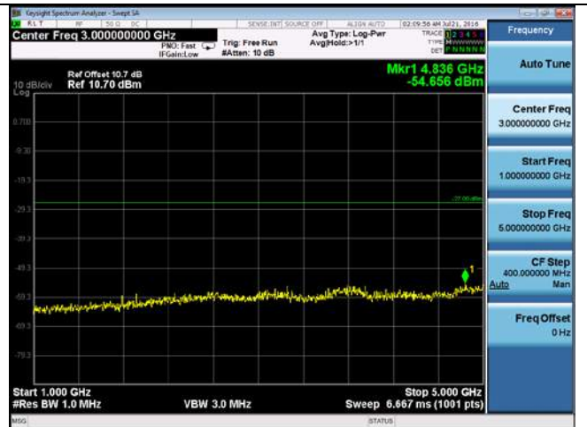
CUE-802.11n-40-5270M-chain4(1GHz-5GHz)
