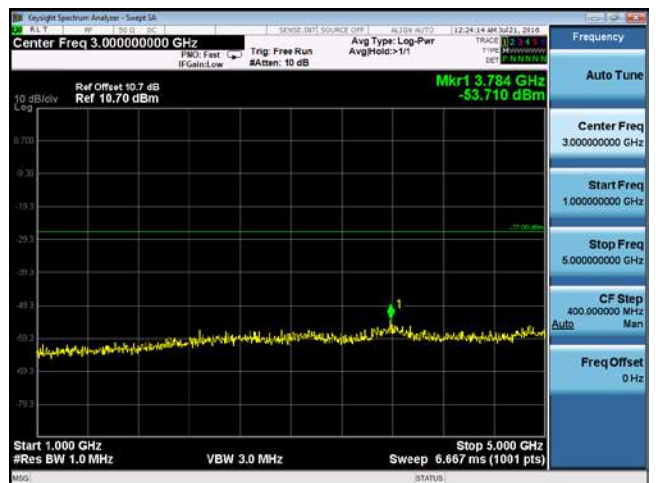
CUE-802.11n-20-5500M-chain2(1GHz-5GHz)
