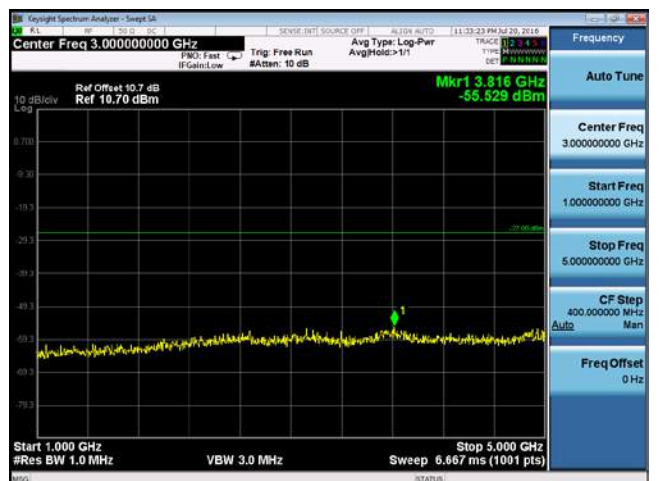
CUE-802.11n-20-5580M-chain1(1GHz-5GHz)
