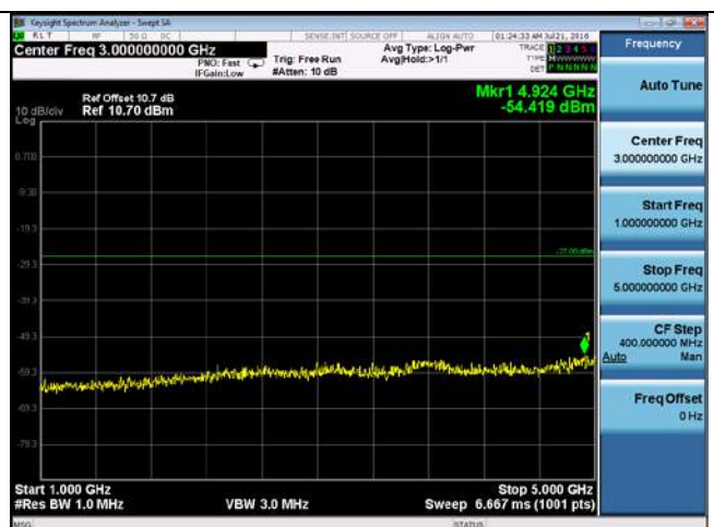
CUE-802.11n-40-5310M-chain3(1GHz-5GHz)
