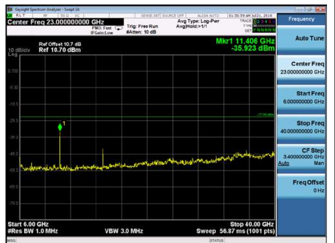
CUE-802.11a-5700M-chain 4(6GHz-40GHz)
