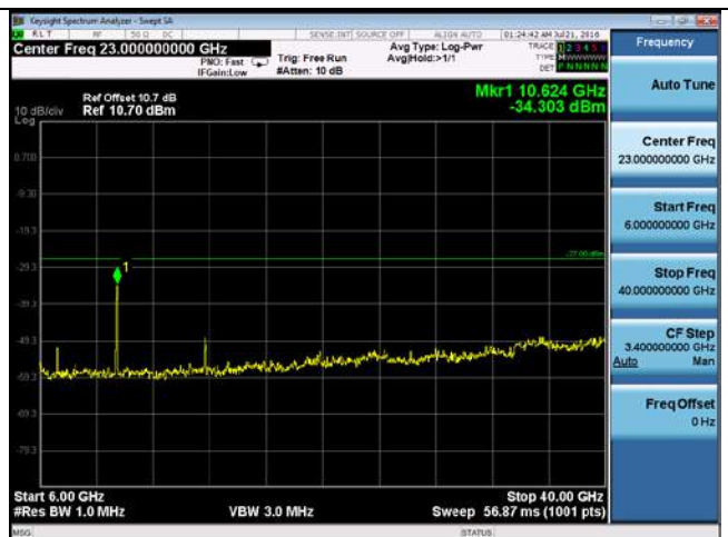
CUE-802.11n-40-5310M-chain3(6GHz-40GHz)
