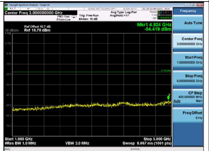
CUE-802.11n-40-5270M-chain3(1GHz-5GHz)
