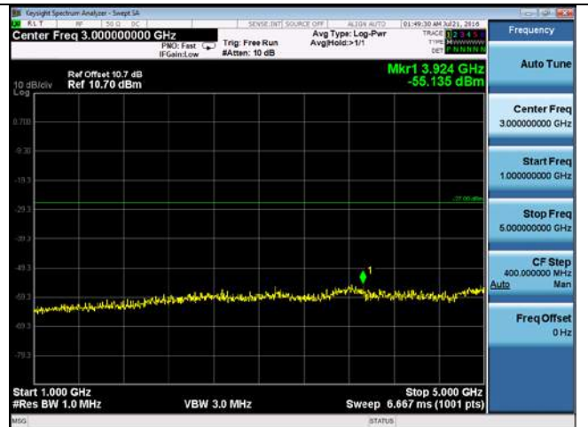
CUE-802.11n-20-5500M-chain4(1GHz-5GHz)
