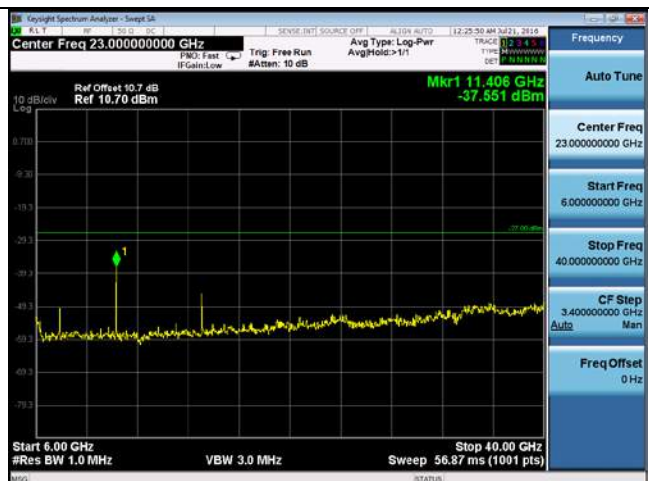
CUE-802.11n-20-5700M chain 2(6GHz-40GHz)
