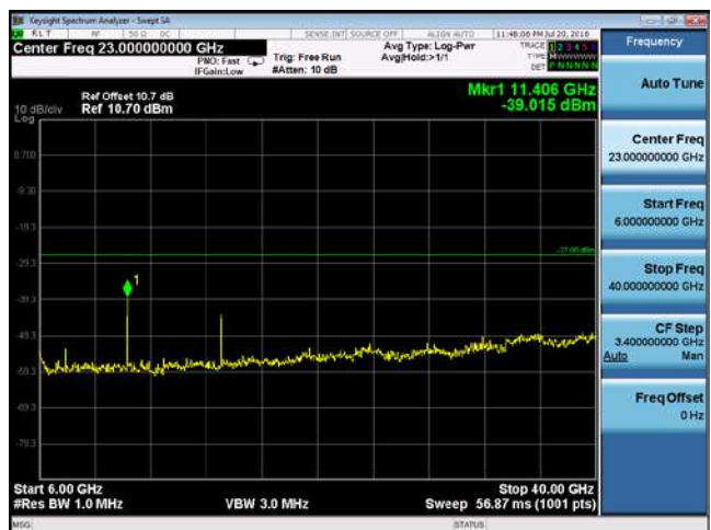
CUE-802.11n-20-5700M -chain 1(6GHz-40GHz)
