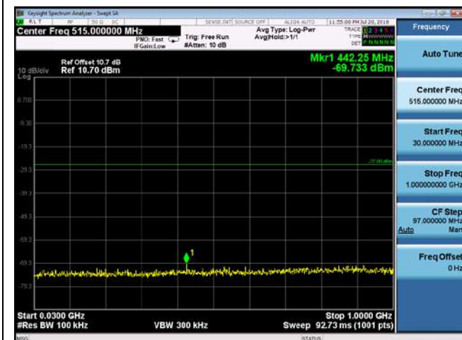
CUE-802.11n-40-5310M-chain1(30MHz-1GHz)
