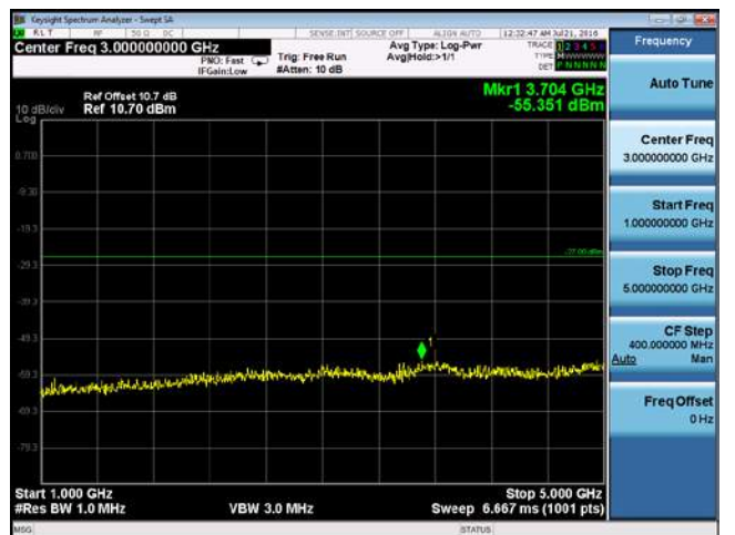
CUE-802.11n-40-5270M-chain2(1GHz-5GHz)
