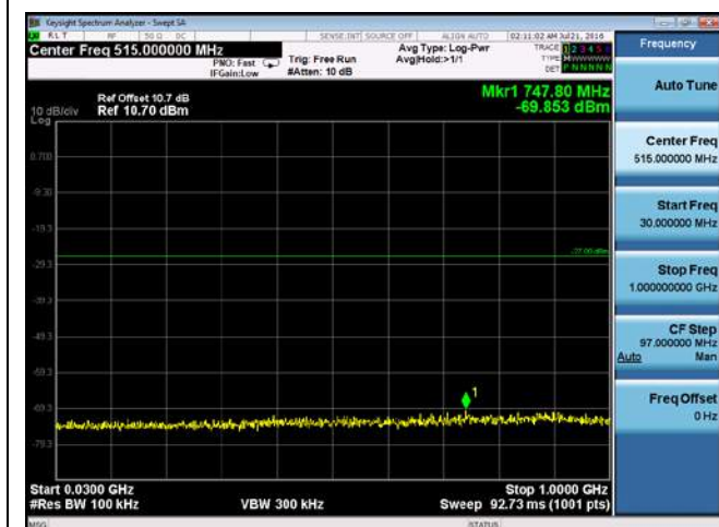
CUE-802.11n-40-5310M-chain4(30MHz-1GHz)
