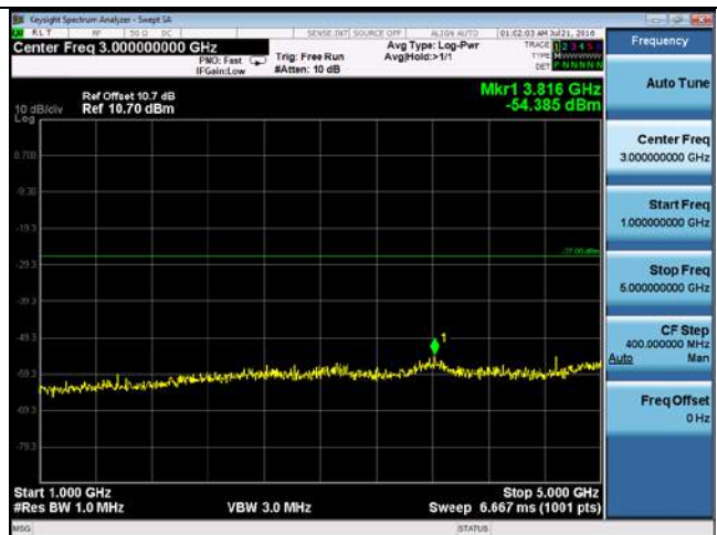
CUE-802.11n-20-5500M-chain3(1GHz-5GHz)
