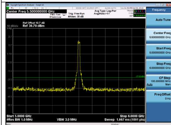
CUE-802.11a-5500M-chain1(5GHz-6GHz)
