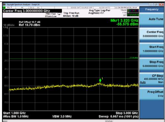
CUE-802.11a-5700M-chain 1(1GHz-5GHz)
