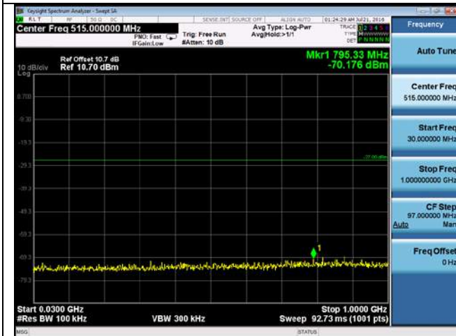
CUE-802.11n-40-5270M-chain3(30MHz-1GHz)
