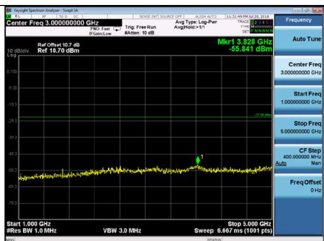
CUE-802.11a-5500M-chain1(1GHz-5GHz)
