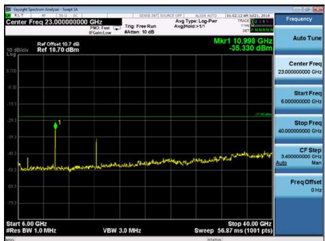
CUE-802.11a-5500M -chain3(6GHz-40GHz)
