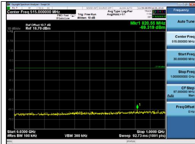
CUE-802.11n-40-5270M-chain1(30MHz-1GHz)
