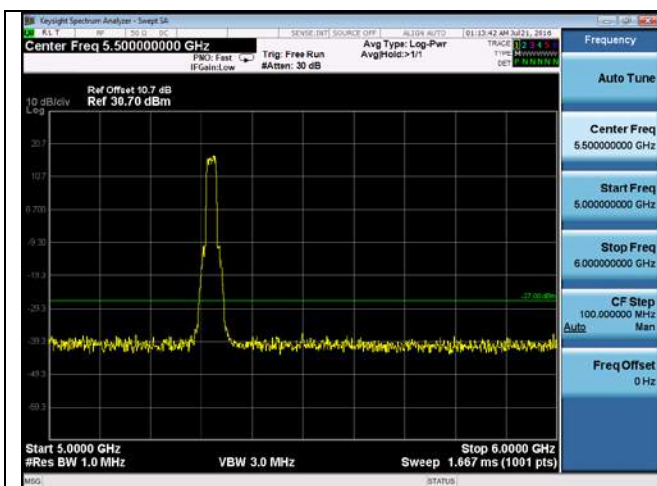
CUE-802.11n-20-5320M-chain 3(5GHz-6GHz)
