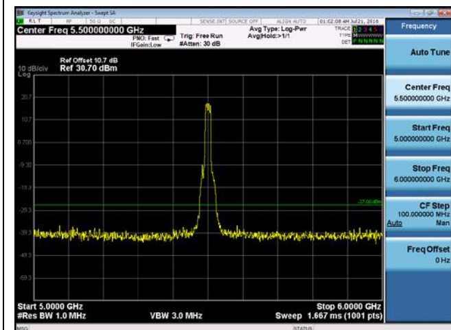
CUE-802.11a-5500M -chain3(5GHz-6GHz)
