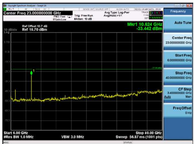
CUE-802.11n-20-5320M-chain 4(6GHz-40GHz)
