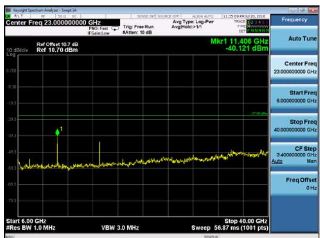
CUE-802.11a-5700M-chain 1(6GHz-40GHz)
