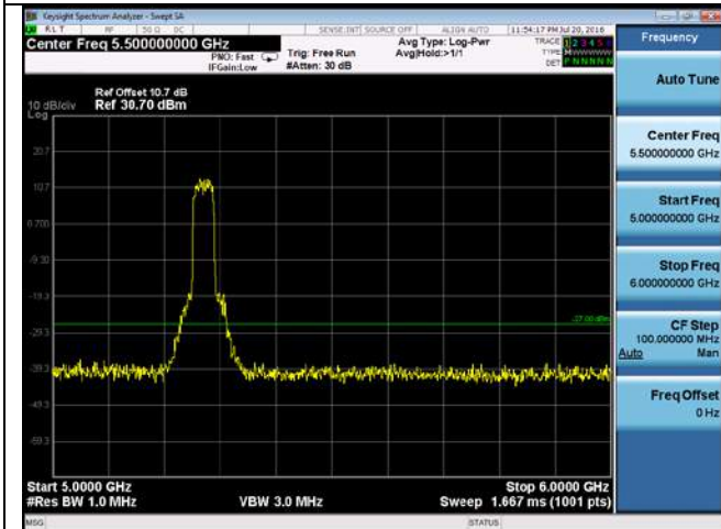
CUE-802.11n-40-5270M-chain1(5GHz-6GHz)
