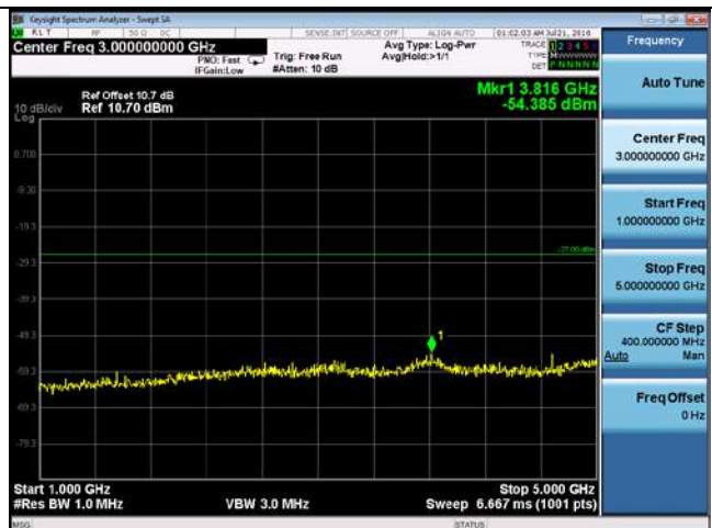
CUE-802.11a-5500M -chain3(1GHz-5GHz)
