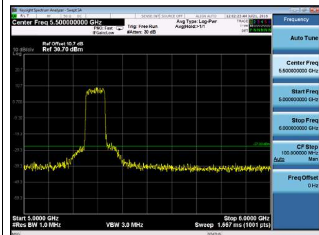
CUE-802.11ac-80-5290M-chain 1(5GHz-6GHz)
