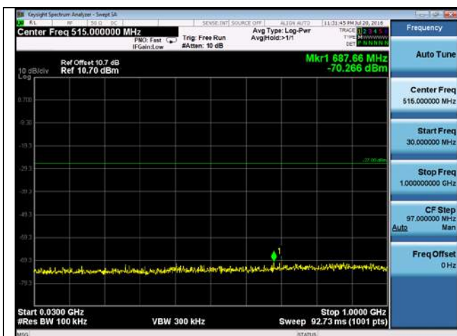
CUE-802.11a-5500M-chain1(30MHz-1GHz)
