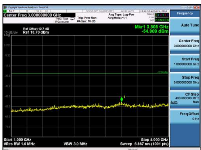
CUE-802.11a-5500M-chain2(1GHz-5GHz)
