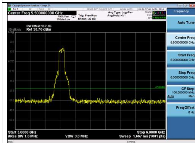
CUE-802.11n-40-5310M-chain3(5GHz-6GHz)
