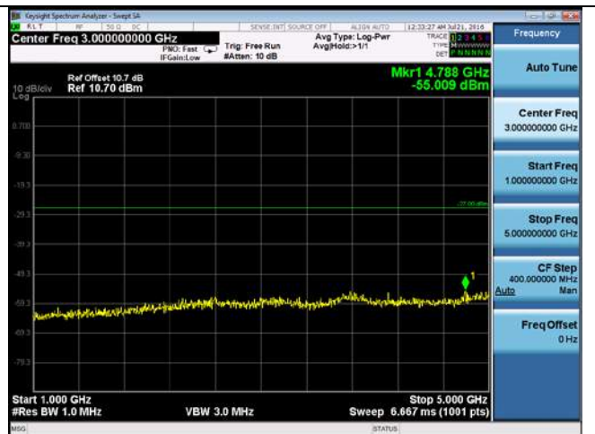
CUE-802.11n-40-5310M chain2(1GHz-5GHz)
