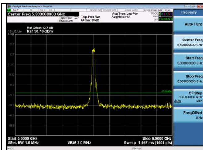
CUE-802.11n-20-5500M-chain2(5GHz-6GHz)
