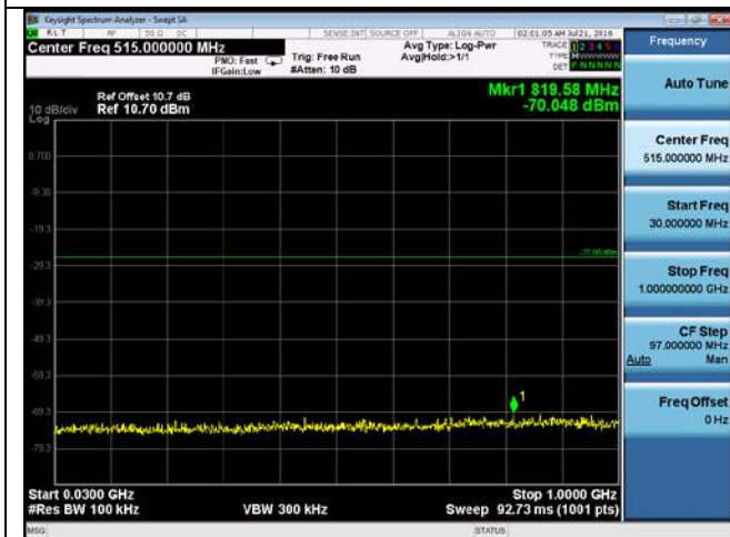
CUE-802.11n-20-5320M-chain 4(30MHz-1GHz)
