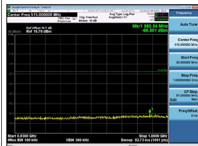
CUE-802.11a-5500M-chain2(30MHz-1GHz)
