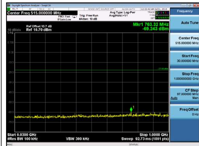
CUE-802.11n-40-5270M-chain2(30MHz-1GHz)
