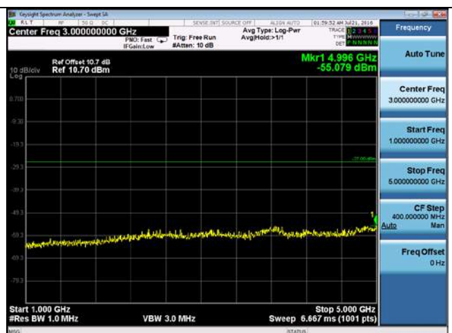
CUE-802.11n-20-5260M-chain4(1GHz-5GHz)
