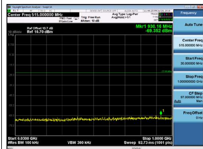
CUE-802.11n-20-5280M-chain1(30MHz-1GHz)
