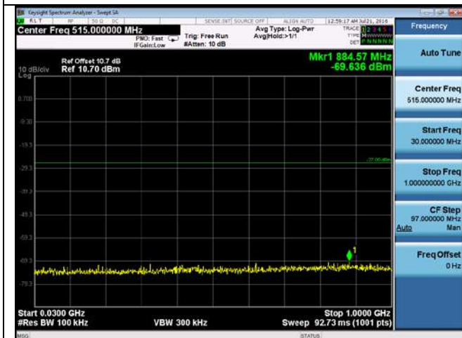
CUE-802.11a-5260M-chain3(30MHz-1GHz)
