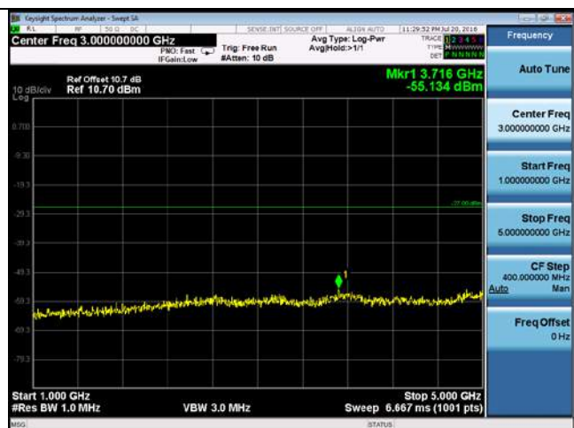
CUE-802.11a-5260M-chain1(1GHz-5GHz)
