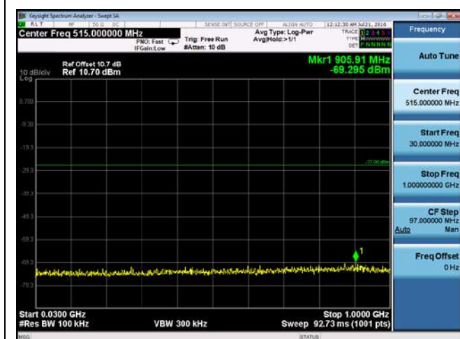
CUE-802.11a-5260M-chain2(30MHz-1GHz)
