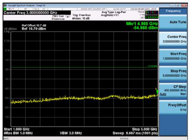
CUE-802.11n-20-5280M-chain4(1GHz-5GHz)
