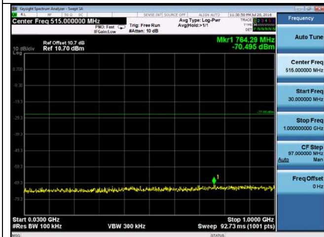
CUE-802.11a-5320M-chain 1(30MHz-1GHz)
