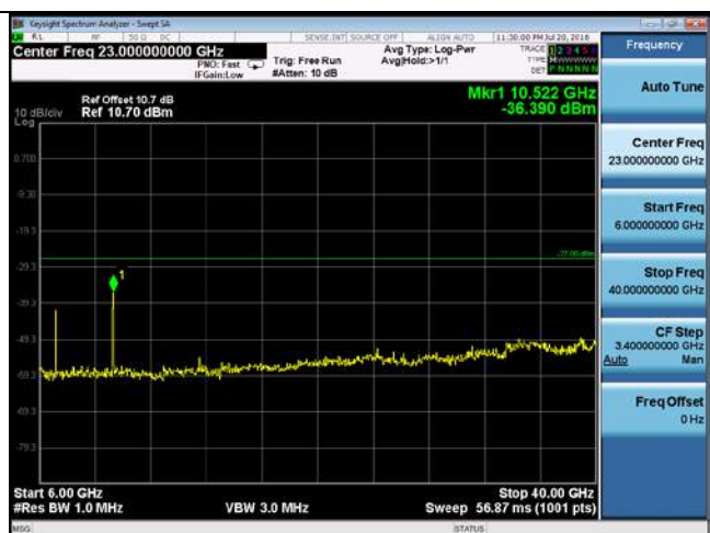
CUE-802.11a-5260M-chain1(6GHz-40GHz)
