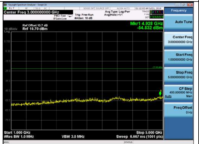
CUE-802.11n-20-5260M chain3(1GHz-5GHz)
