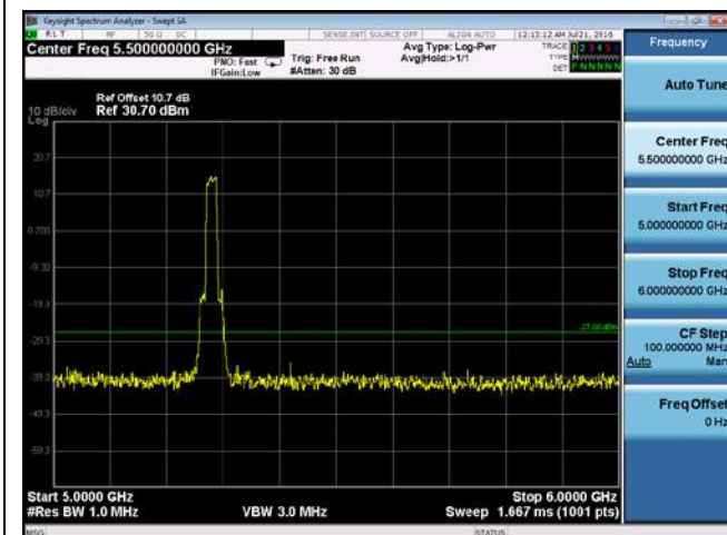
CUE-802.11a-5280M -chain2(5GHz-6GHz)
