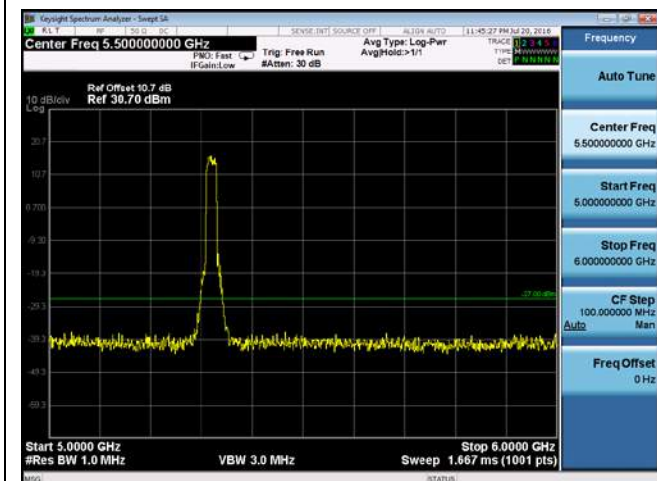
CUE-802.11n-20-5320M-chain 1(5GHz-6GHz)
