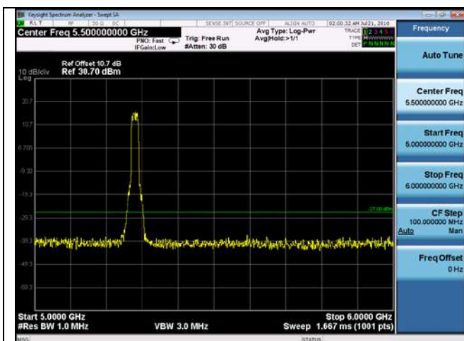
CUE-802.11n-20-5280M-chain 4(5GHz-6GHz)
