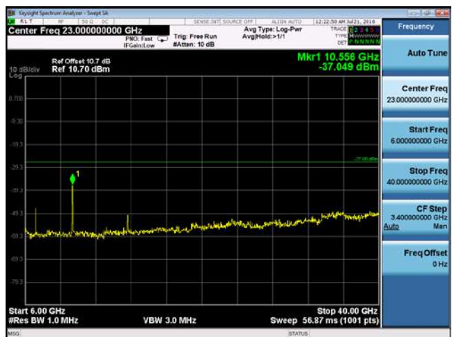
CUE-802.11n-20-5280M -chain2(6GHz-40GHz)
