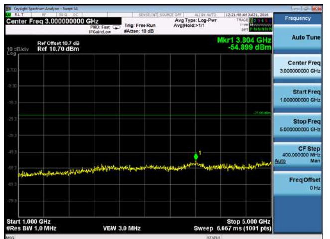
CUE-802.11n-20-5260M-chain2(1GHz-5GHz)
