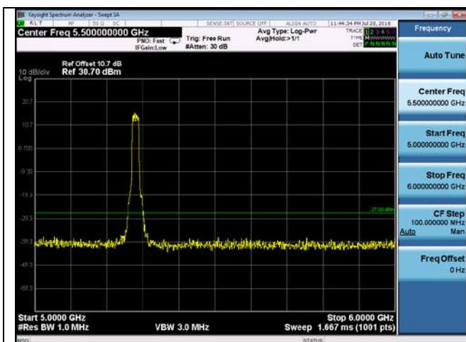
CUE-802.11n-20-5280M -chain1(5GHz-6GHz)
