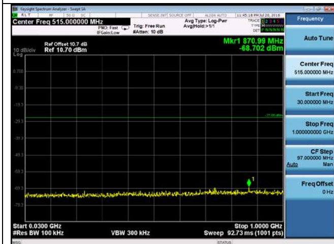
CUE-802.11n-20-5320M-chain 1(30MHz-1GHz)
