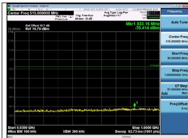
CUE-802.11a-5260M-chain1(30MHz-1GHz)
