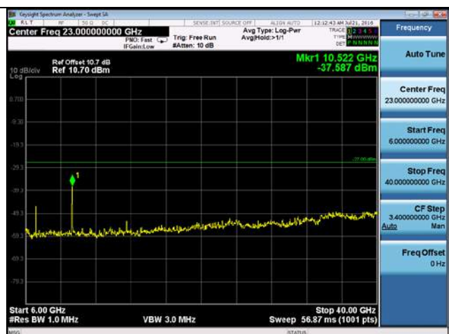
CUE-802.11a-5260M-chain2(6GHz-40GHz)
