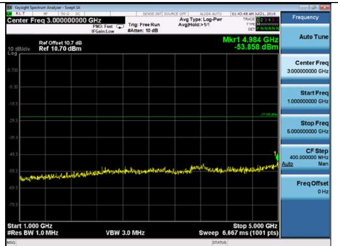
CUE-802.11a-5260M-chain4(1GHz-5GHz)
