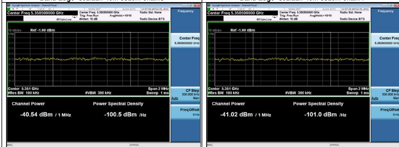
Band Edge -802.11ac-80M-5290M-chain1
