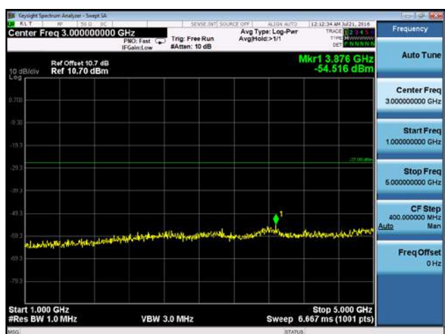
CUE-802.11a-5260M-chain2(1GHz-5GHz)
