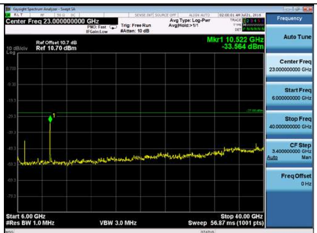
CUE-802.11n-20-5260M-chain4(6GHz-40GHz)
