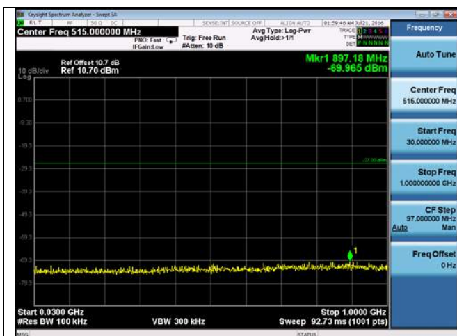
CUE-802.11n-20-5260M-chain4(30MHz-1GHz)
