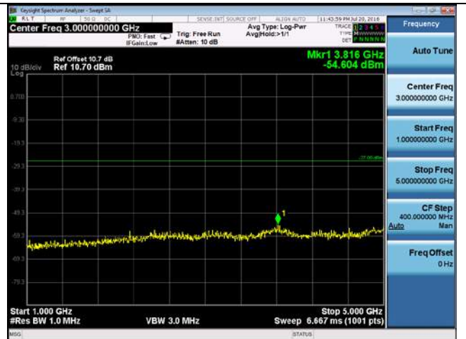
CUE-802.11n-20-5260M-chain1(1GHz-5GHz)
