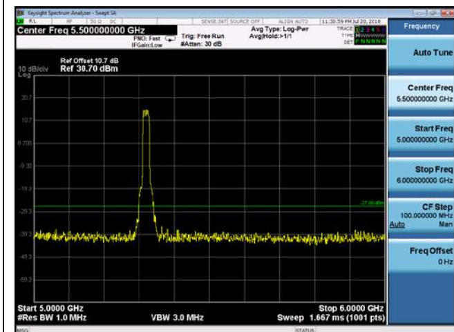
CUE-802.11a-5320M -chain 1(5GHz-6GHz)
