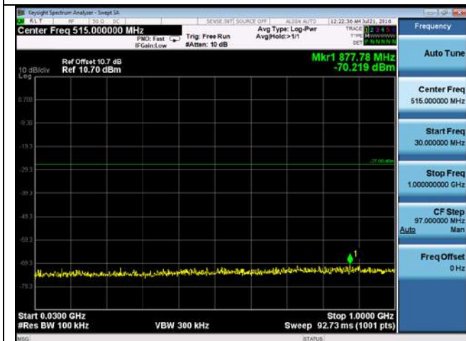
CUE-802.11n-20-5280M -chain2(30MHz-1GHz)
