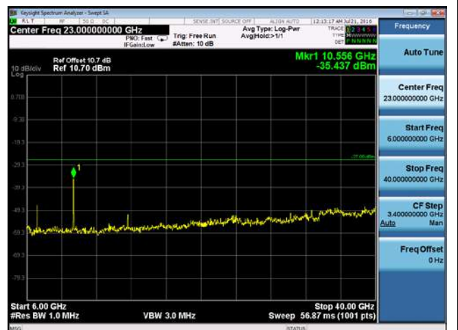
CUE-802.11a-5280M -chain2(6GHz-40GHz)
