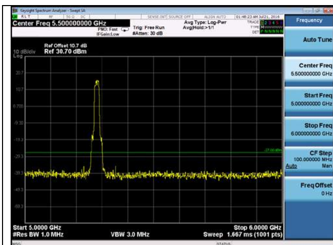
CUE-802.11a-5280M chain 4(5GHz-6GHz)
