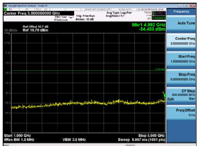
CUE-802.11a-5280M-chain1(1GHz-5GHz)
