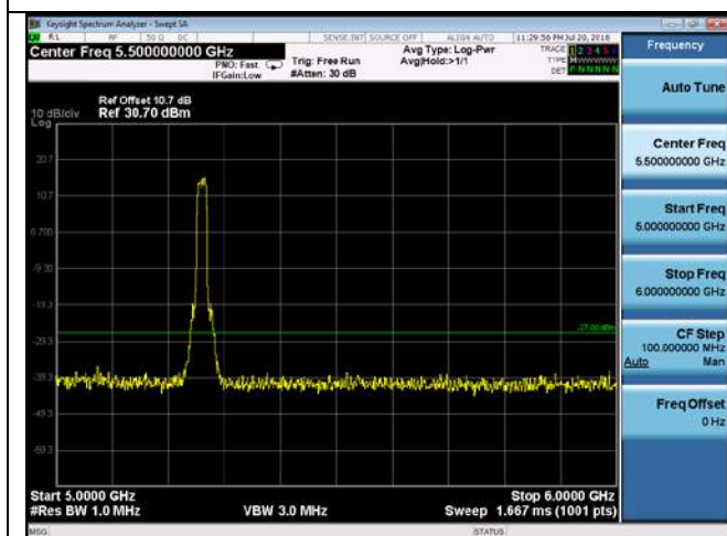
CUE-802.11a-5260M-chain1(5GHz-6GHz)
