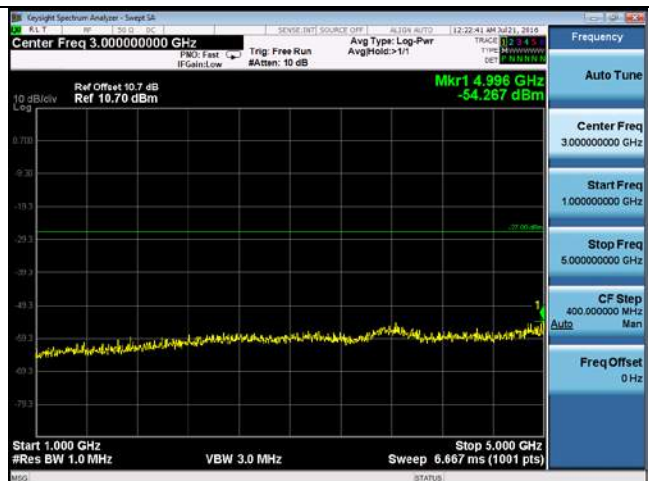
CUE-802.11n-20-5280M -chain2(1GHz-5GHz)
