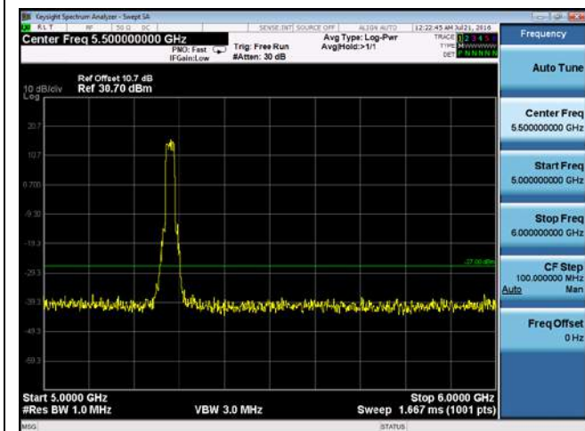
CUE-802.11n-20-5280M -chain2(5GHz-6GHz)
