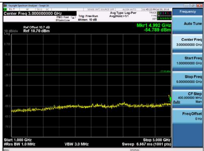
CUE-802.11n-20-5320M-chain 1(1GHz-5GHz)
