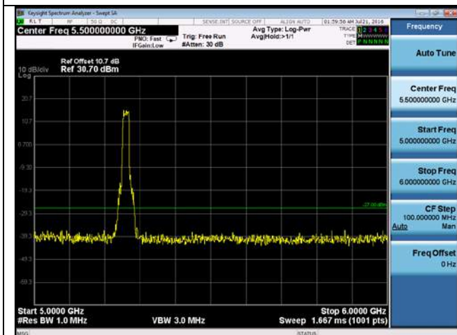
CUE-802.11n-20-5260M-chain4(5GHz-6GHz)
