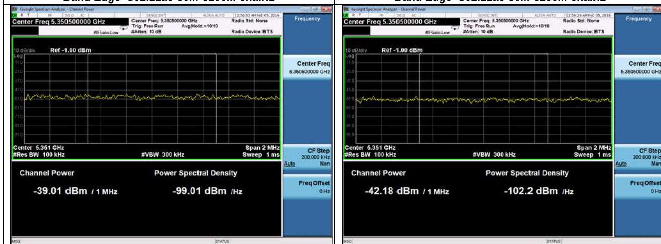
Band Edge -802.11ac-80M-5290M-chain3
