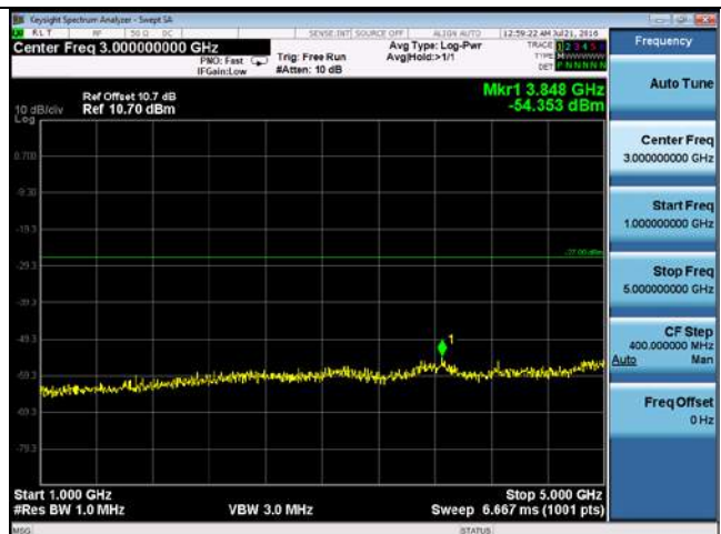
CUE-802.11a-5260M-chain3(1GHz-5GHz)
