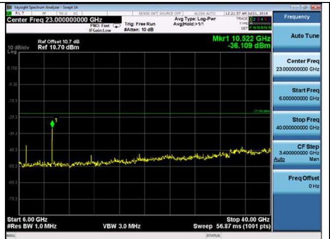
CUE-802.11n-20-5260M chain2(6GHz-40GHz)
