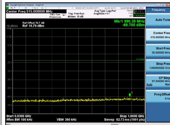
CUE-802.11n20-5720M -chain2(30MHz-1GHz)
