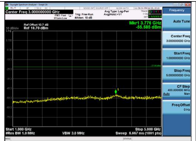
CUE-802.11a-5720M -chain1(1GHz-5GHz)
