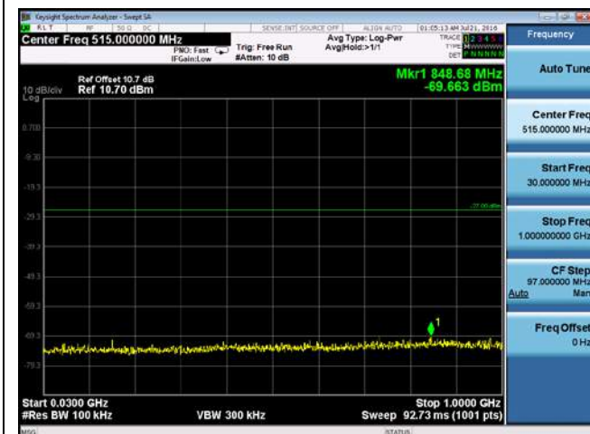
CUE-802.11a-5720M -chain3 (30MHz-1GHz)
