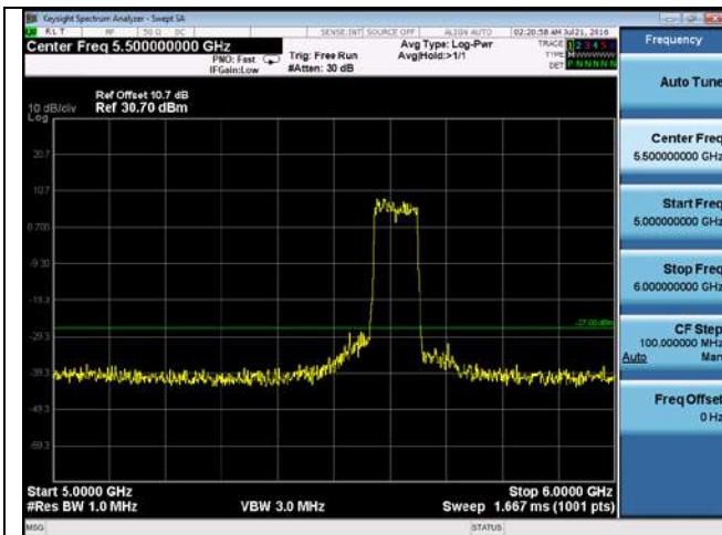
CUE-802.11ac-80-5610M chain 4(5GHz-6GHz)
