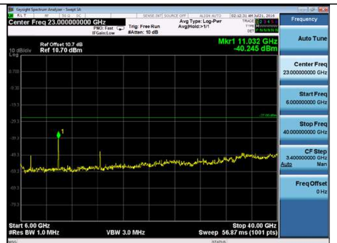
CUE-802.11n-40-5510M-chain4(6GHz-40GHz)
