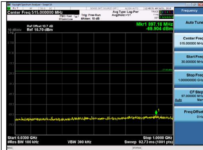
CUE-802.11ac80-5690M -chain2 (30MHz-1GHz)
