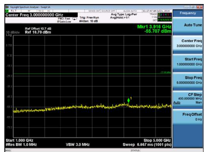
CUE-802.11n20-5720M -chain3(1GHz-5GHz)
