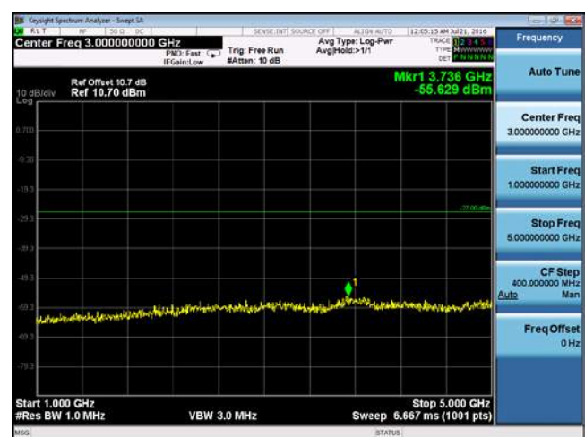
CUE-802.11ac80-5690M -chain1(1GHz-5GHz)
