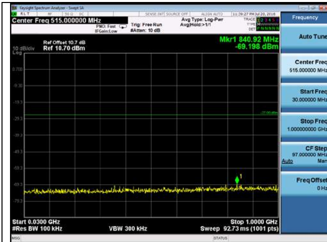
CUE-802.11a-5720M -chain1(30MHz-1GHz)
