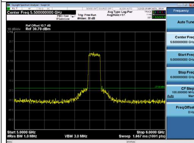
CUE-802.11ac-80-5530M-chain1(5GHz-6GHz)
