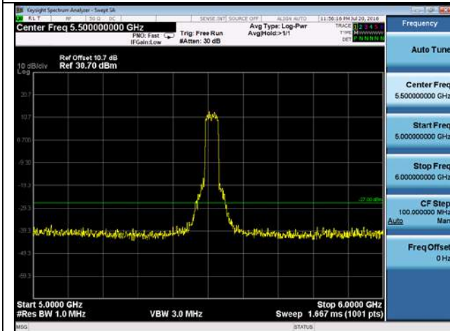
CUE-802.11n-40-5510M-chain1(5GHz-6GHz)
