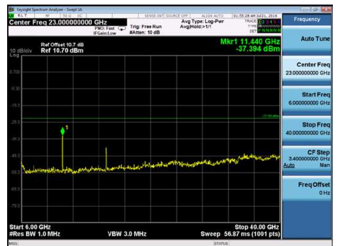
CUE-802.11a-5720M -chain4 (6GHz-40GHz)
