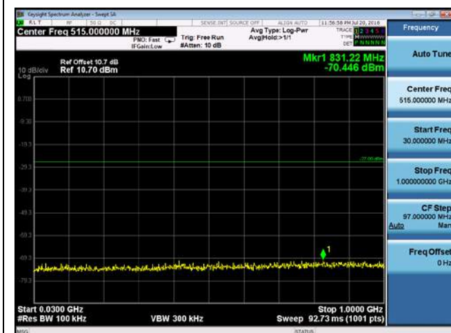
CUE-802.11n-40-5550M-chain1(30MHz-1GHz)
