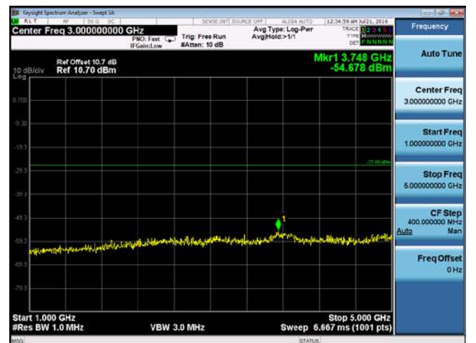
CUE-802.11n-40-5510M-chain2(1GHz-5GHz)
