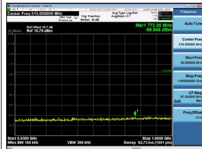
CUE-802.11ac-80-5610M-chain1(30MHz-1GHz)
