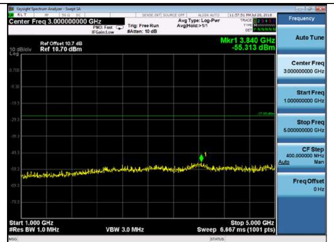
CUE-802.11n-40-5670M-chain 1(1GHz-5GHz)
