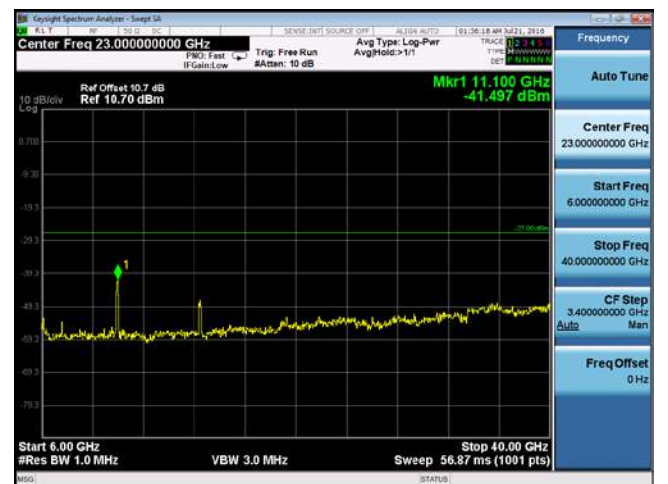
CUE-802.11ac-80-5530M -chain3(6GHz-40GHz)
