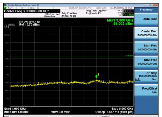
CUE-802.11n-40-5550M-chain1(1GHz-5GHz)
