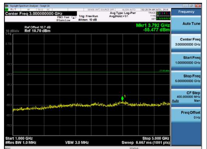
CUE-802.11ac-80-5610M-chain4(1GHz-5GHz)
