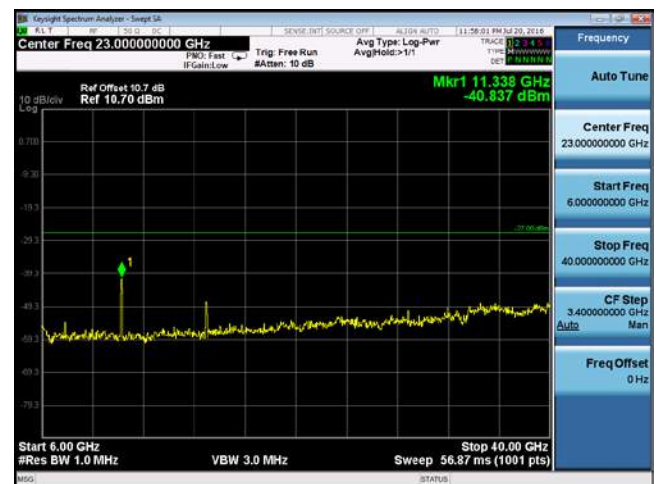
CUE-802.11n-40-5670M-chain 1(6GHz-40GHz)
