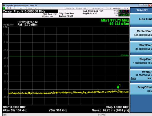
CUE-802.11ac80-5690M -chain1(30MHz-1GHz)
