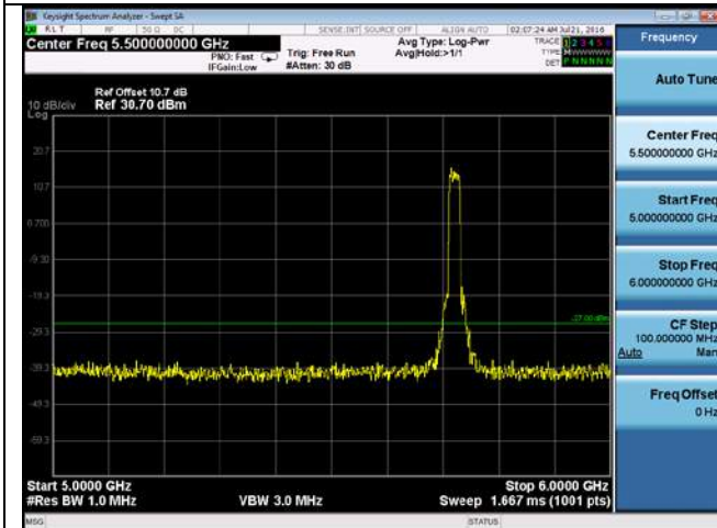
CUE-802.11n20-5720M -chain4(5GHz-6GHz)
