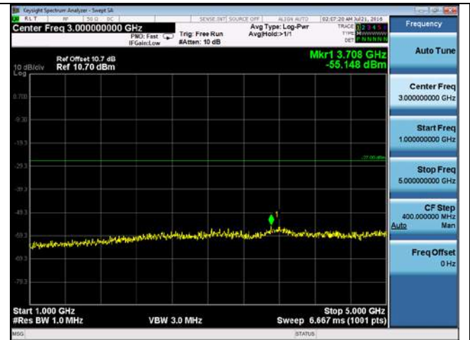
CUE-802.11n20-5720M -chain4(1GHz-5GHz)
