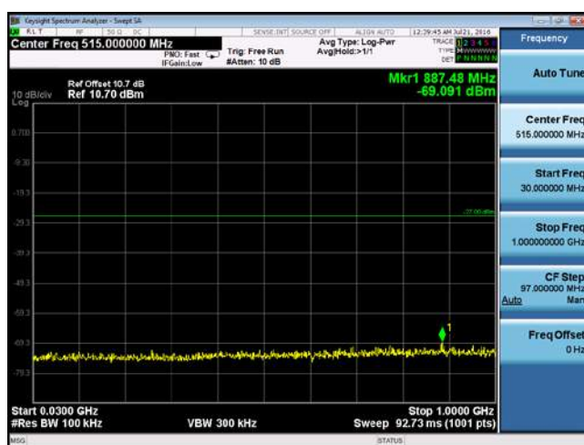
CUE-802.11n40-5710M -chain2(30MHz-1GHz)
