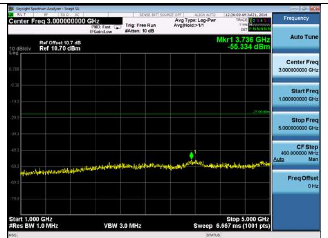
CUE-802.11n-40-5550M-chain2(1GHz-5GHz)
