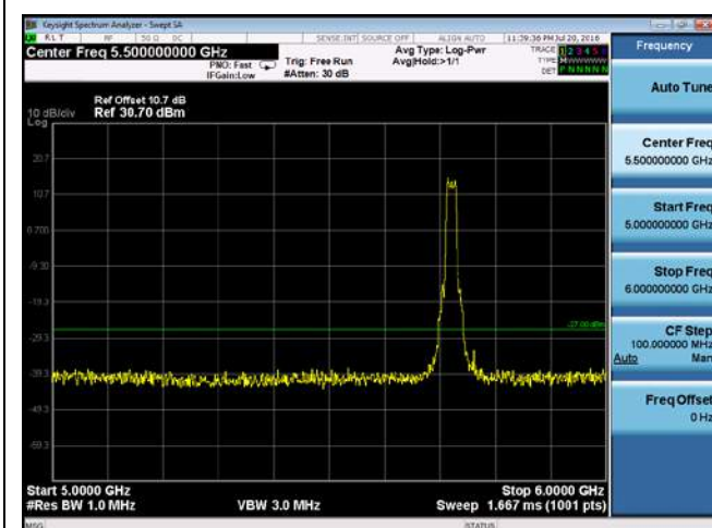
CUE-802.11a-5720M -chain1(5GHz-6GHz)
