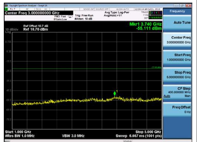
CUE-802.11ac-80-5610M-chain1(1GHz-5GHz)
