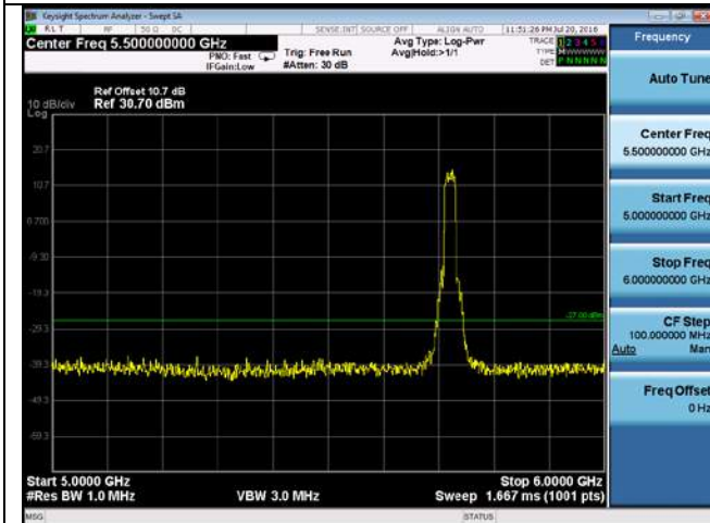
CUE-802.11n20-5720M -chain1(5GHz-6GHz)
