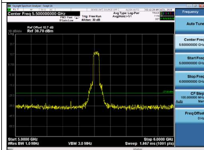
CUE-802.11n-40-5510M-chain4(5GHz-6GHz)
