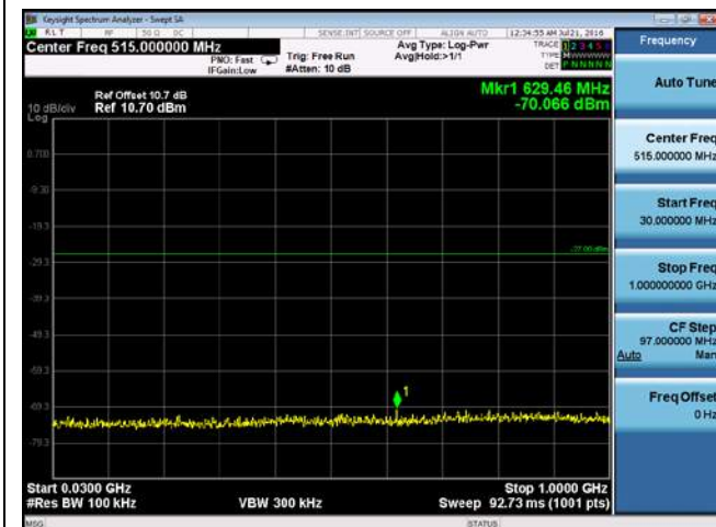
CUE-802.11n-40-5510M-chain2(30MHz-1GHz)
