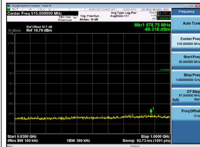
CUE-802.11ac80-5690M -chain3 (30MHz-1GHz)
