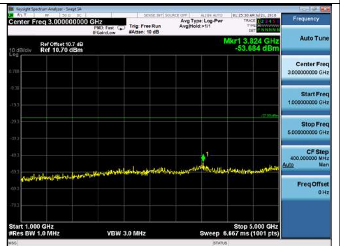
CUE-802.11n-40-5510M-chain3(1GHz-5GHz)
