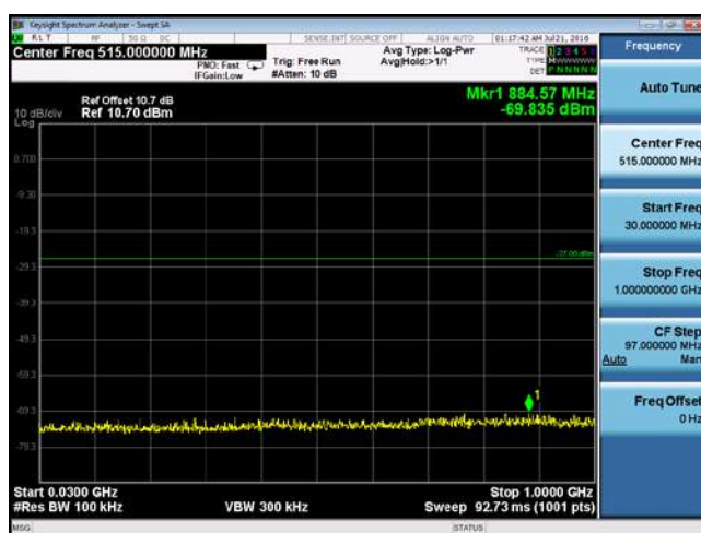
CUE-802.11n20-5720M -chain3(30MHz-1GHz)
