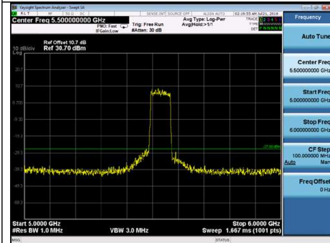
CUE-802.11ac-80-5530M-chain4(5GHz-6GHz)
