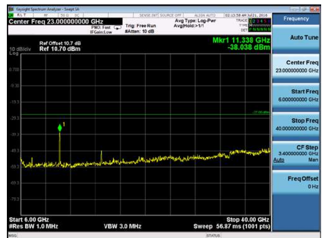
CUE-802.11n-40-5670M-chain 4 (6GHz-40GHz)
