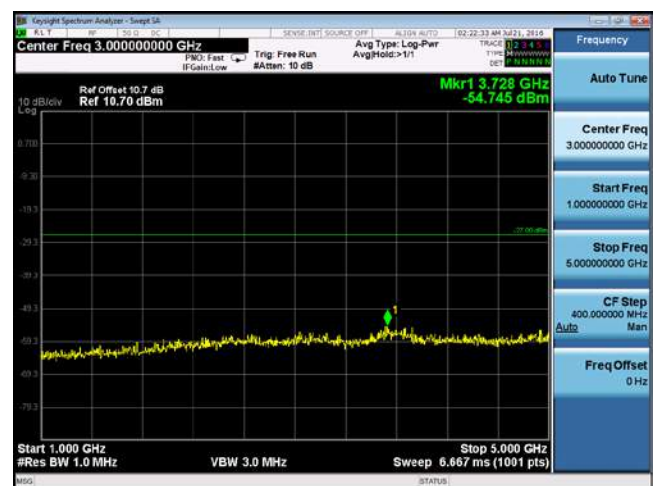
CUE-802.11ac80-5690M -chain4 (1GHz-5GHz)
