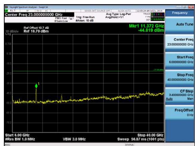
CUE-802.11ac80-5690M -chain1 (6GHz-40GHz)
