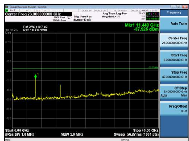
CUE-802.11n20-5720M -chain3 (6GHz-40GHz)
