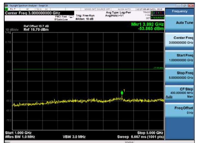
CUE-802.11n20-5720M -chain2(1GHz-5GHz)
