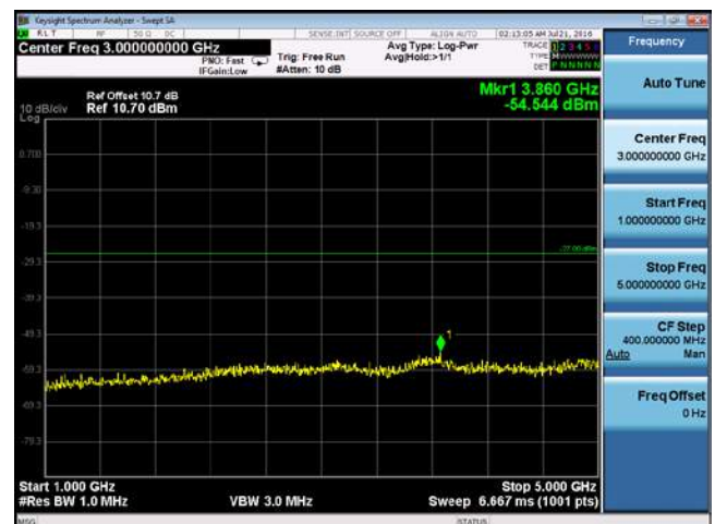
CUE-802.11n-40-5550M-chain4(1GHz-5GHz)
