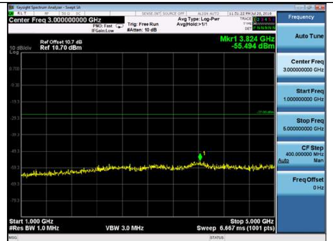
CUE-802.11n20-5720M -chain1(1GHz-5GHz)
