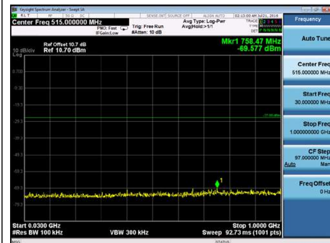
CUE-802.11n-40-5550M-chain4(30MHz-1GHz)
