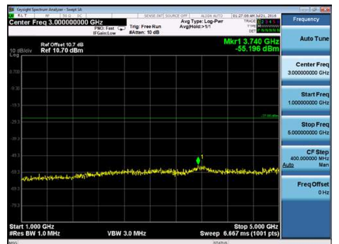
CUE-802.11n-40-5670M -chain 3(1GHz-5GHz)
