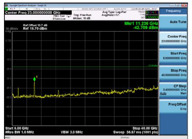
CUE-802.11ac-80-5610M-chain2(6GHz-40GHz)
