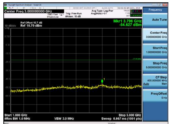
CUE-802.11n-20-5580M-chain4(1GHz-5GHz)
