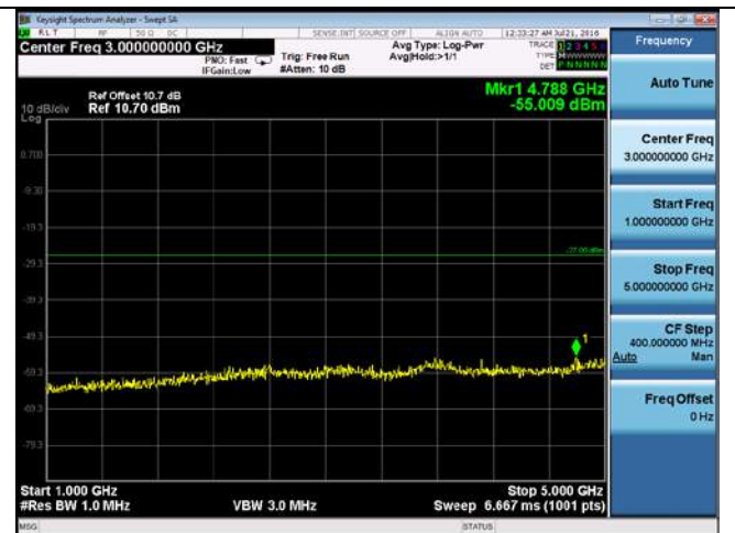
CUE-802.11n-40-5310M chain2(1GHz-5GHz)
