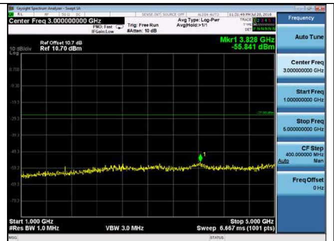
CUE-802.11a-5500M-chain1(1GHz-5GHz)
