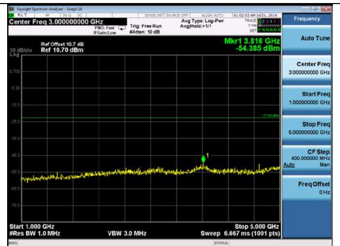
CUE-802.11a-5500M -chain3(1GHz-5GHz)
