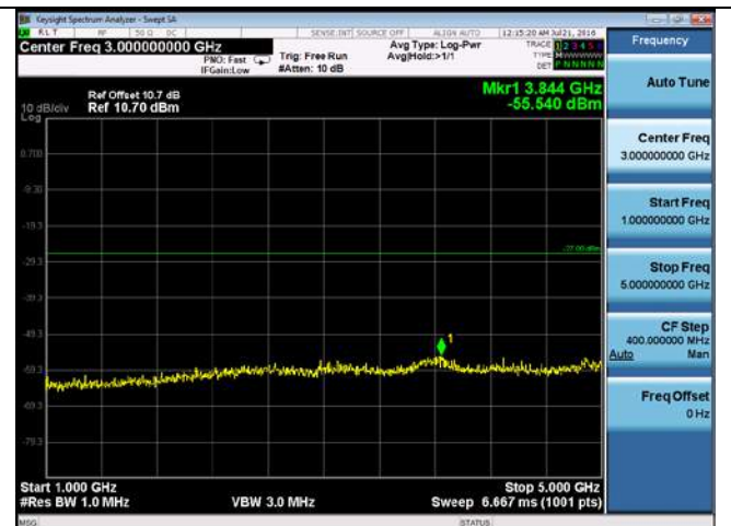
CUE-802.11a-5580M--chain2(1GHz-5GHz)
