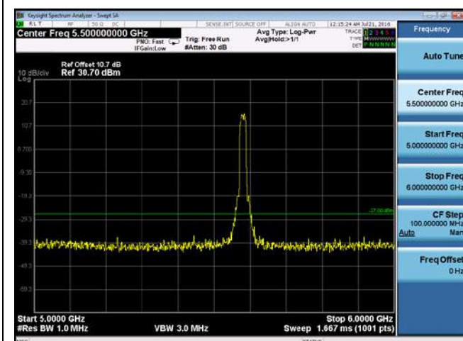
CUE-802.11a-5580M--chain2(5GHz-6GHz)
