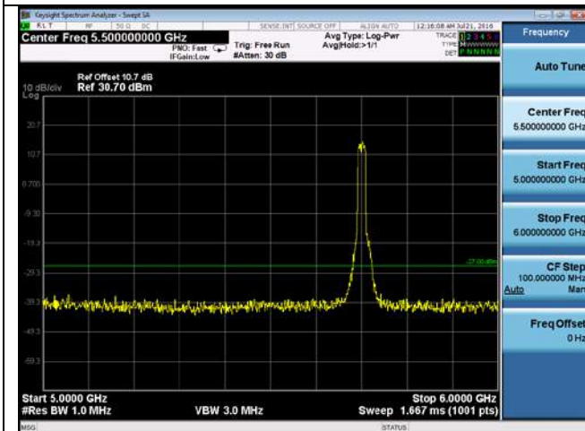
CUE-802.11a-5700M-chain 2(5GHz-6GHz)
