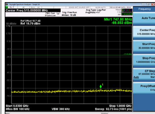
CUE-802.11n-40-5310M-chain4(30MHz-1GHz)
