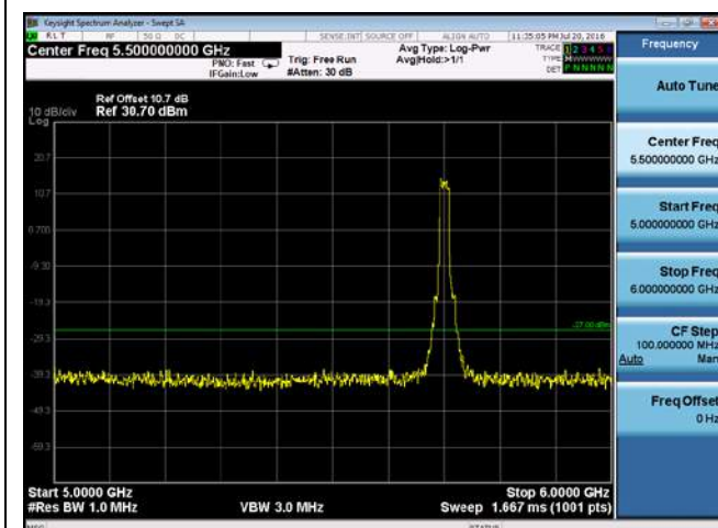
CUE-802.11a-5700M-chain 1(5GHz-6GHz)
