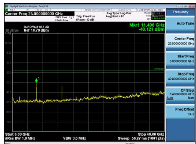
CUE-802.11a-5700M-chain 1(6GHz-40GHz)
