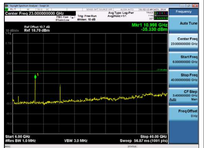
CUE-802.11n-20-5500M-chain3(6GHz-40GHz)
