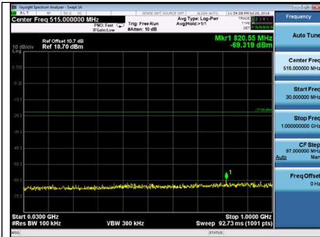
CUE-802.11n-40-5270M-chain1(30MHz-1GHz)
