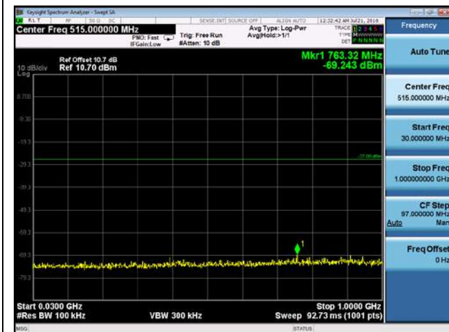
CUE-802.11n-40-5270M-chain2(30MHz-1GHz)
