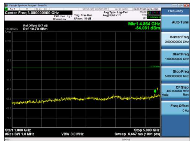
CUE-802.11ac-80-5290M-chain 3(1GHz-5GHz)
