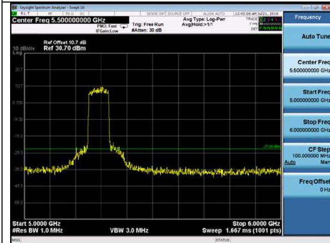
CUE-802.11ac-80-5290M-chain 2(5GHz-6GHz)
