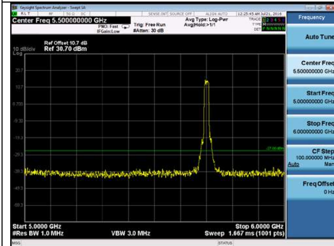
CUE-802.11n-20-5700M -chain 2(5GHz-6GHz)
