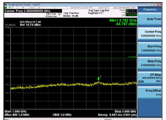
CUE-802.11n-40-5310M-chain4(1GHz-5GHz)
