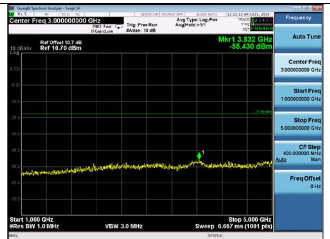
CUE-802.11n-20-5320M-chain 2(1GHz-5GHz)
