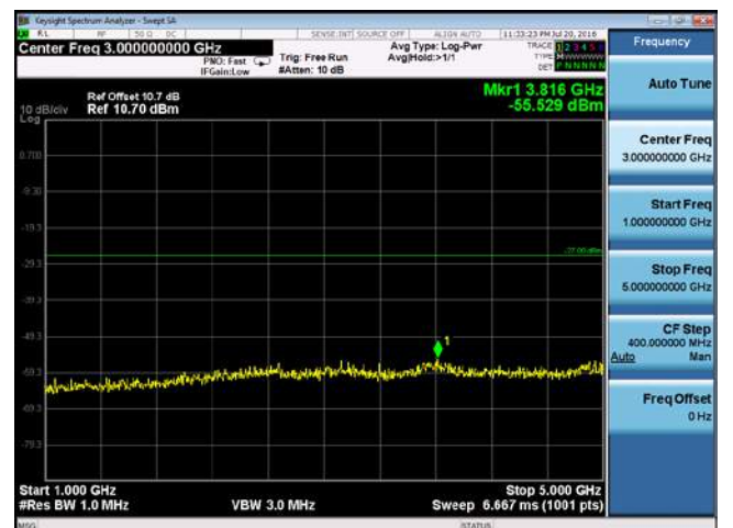
CUE-802.11n-20-5580M-chain1(1GHz-5GHz)
