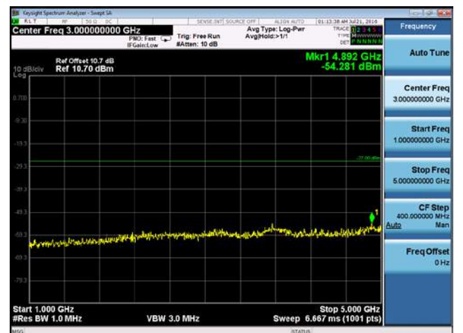
CUE-802.11n-20-5320M-chain 3(1GHz-5GHz)
