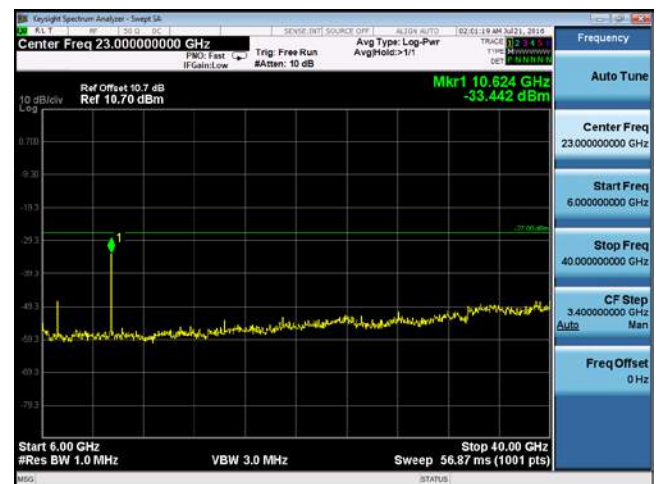
CUE-802.11n-20-5320M-chain 4(6GHz-40GHz)
