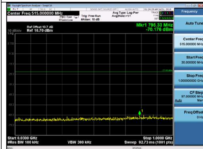
CUE-802.11n-40-5270M-chain3(30MHz-1GHz)
