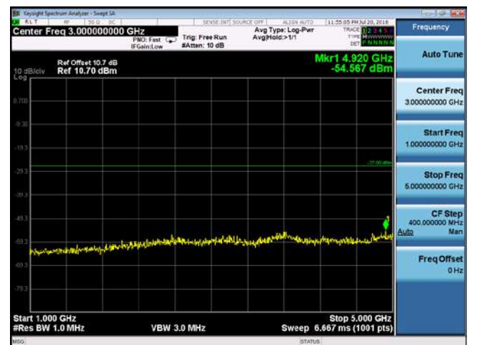
CUE-802.11n-40-5310M-chain1(1GHz-5GHz)
