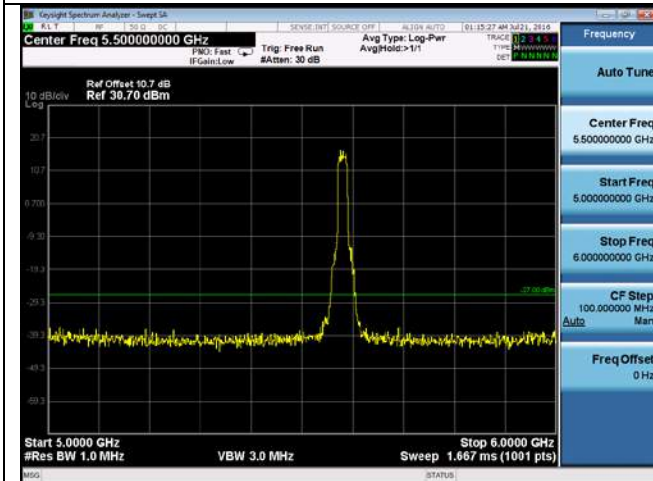
CUE-802.11n-20-5580M-chain3(5GHz-6GHz)
