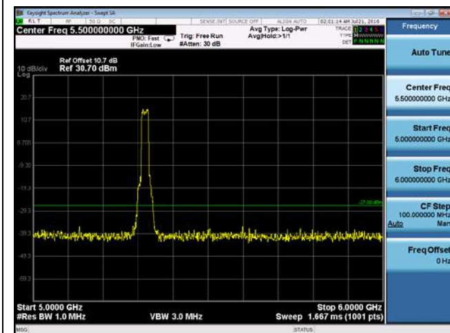
CUE-802.11n-20-5320M-chain 4(5GHz-6GHz)
