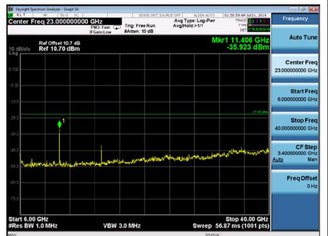
CUE-802.11a-5700M-chain 4(6GHz-40GHz)
