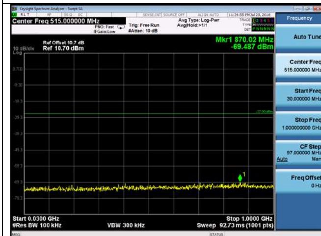
CUE-802.11a-5700M-chain 1(30MHz-1GHz)
