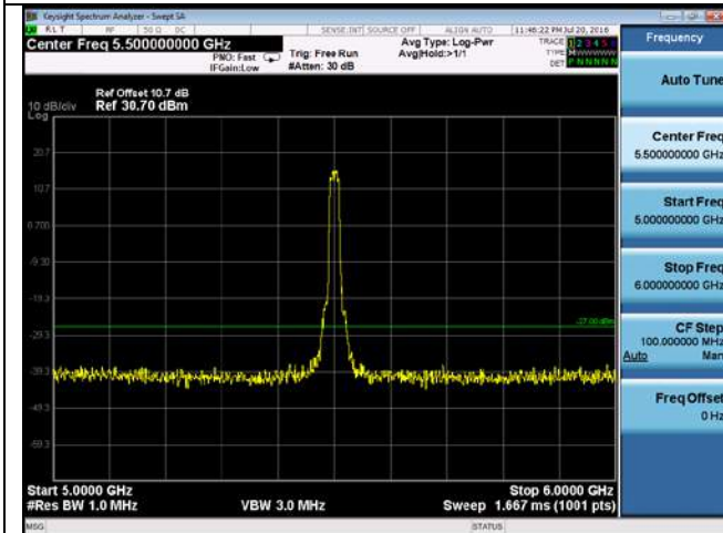
CUE-802.11n-20-5500M-chain1(5GHz-6GHz)
