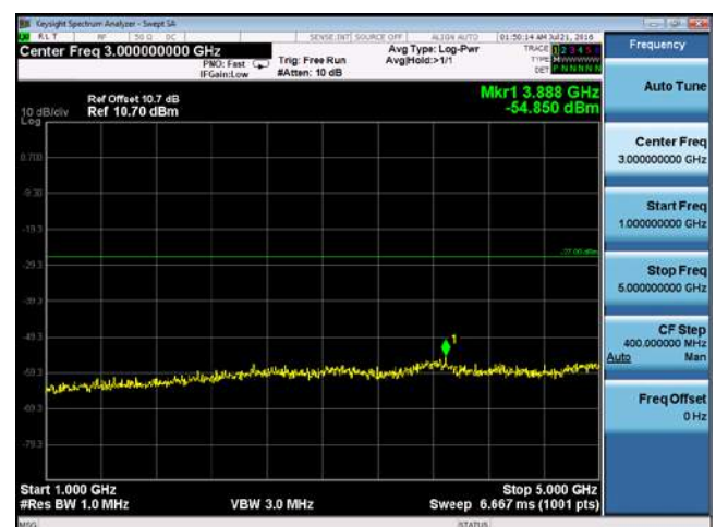
CUE-802.11a-5580M -chain4(1GHz-5GHz)
