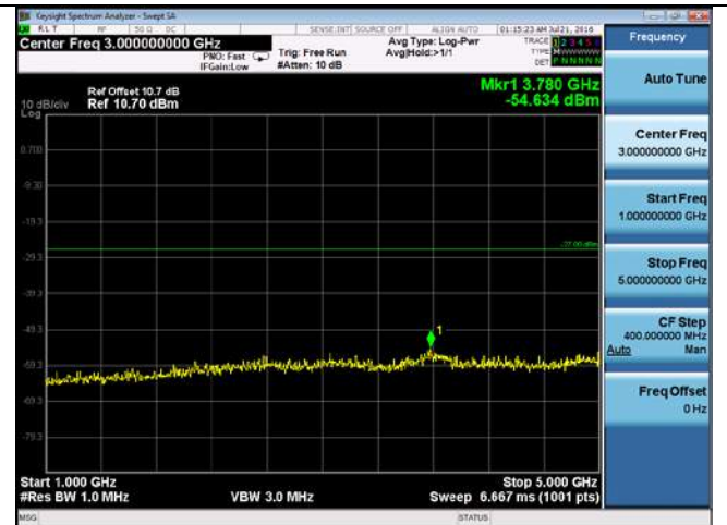
CUE-802.11n-20-5580M-chain3(1GHz-5GHz)
