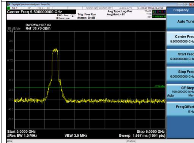
CUE-802.11n-40-5270M-chain1(5GHz-6GHz)
