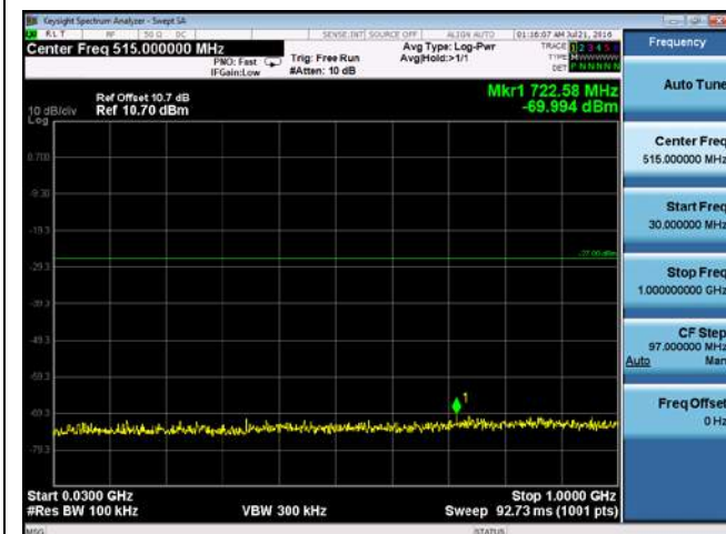
CUE-802.11n-20-5700M -chain 3(30MHz-1GHz)
