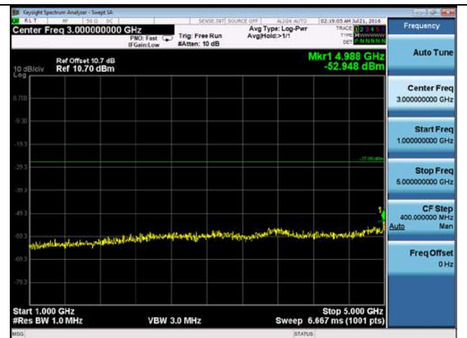
CUE-802.11ac-80-5290M-chain 4(1GHz-5GHz)
