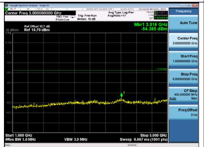
CUE-802.11n-20-5500M-chain3(1GHz-5GHz)
