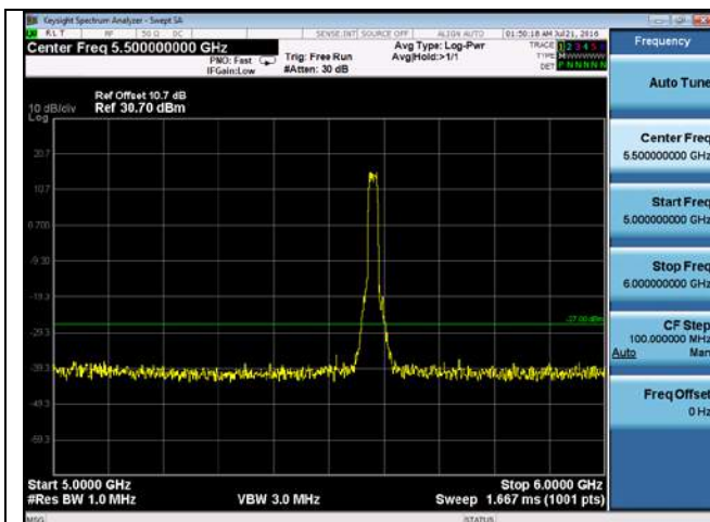
CUE-802.11a-5580M-chain 4(5GHz-6GHz)
