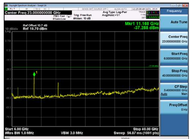
CUE-802.11n-20-5580M-chain2(6GHz-40GHz)
