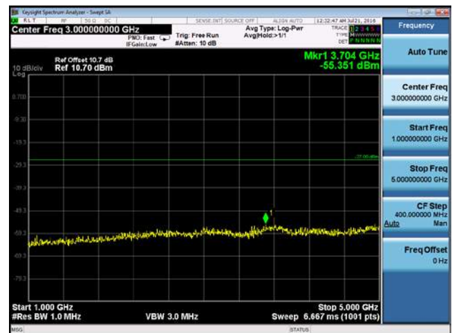
CUE-802.11n-40-5270M-chain2(1GHz-5GHz)
