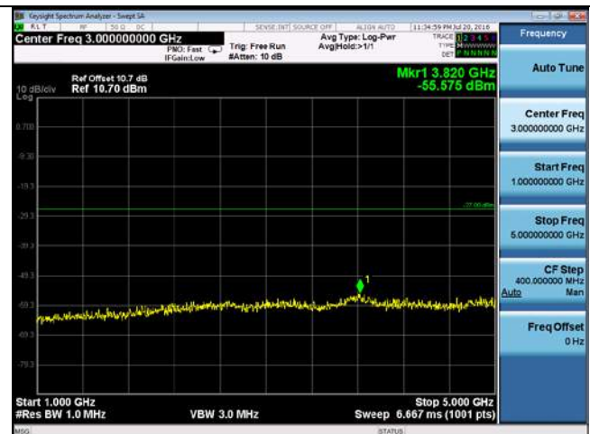
CUE-802.11a-5700M-chain 1(1GHz-5GHz)
