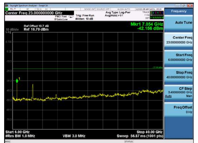
CUE-802.11ac-80-5290M-chain 1(6GHz-40GHz)
