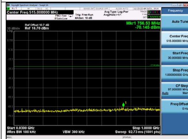
CUE-802.11n-40-5310M -chain2(30MHz-1GHz)
