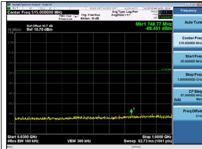
CUE-802.11n-20-5700M -chain 2(30MHz-1GHz)
