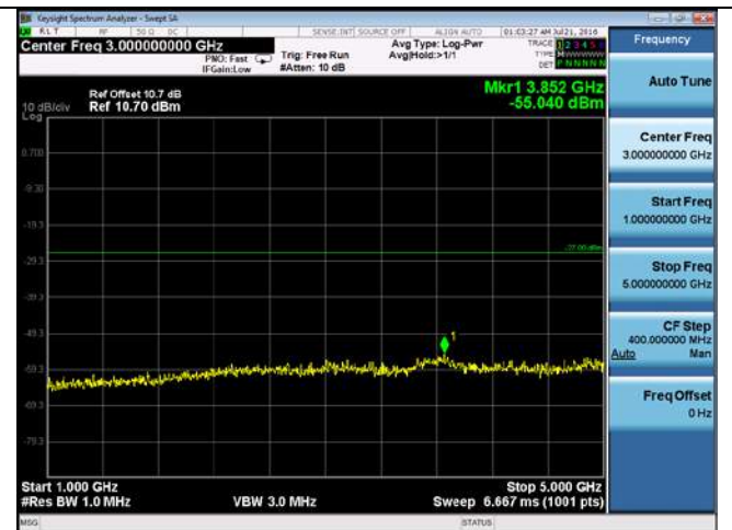
CUE-802.11a-5580M -chain3(1GHz-5GHz)
