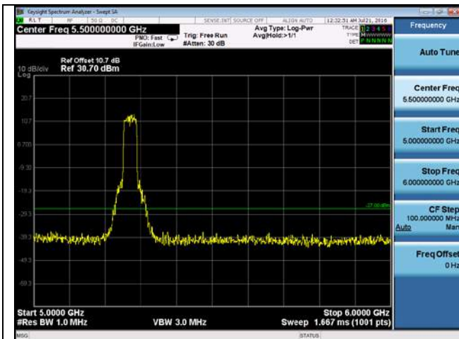
CUE-802.11n-40-5270M-chain2(5GHz-6GHz)
