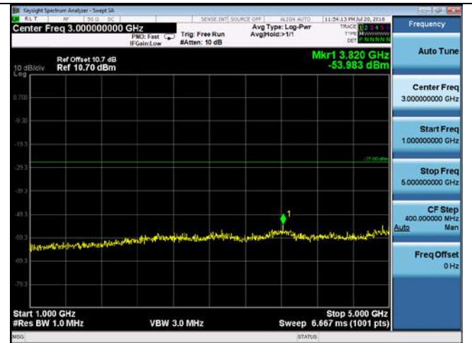
CUE-802.11n-40-5270M-chain1(1GHz-5GHz)
