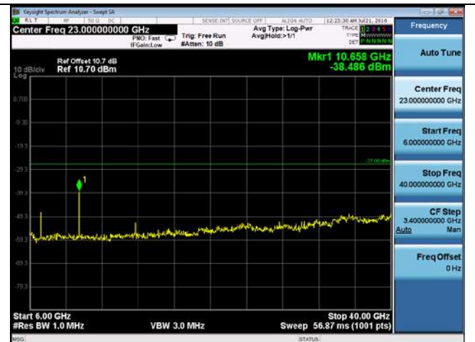
CUE-802.11n-20-5320M-chain 2(6GHz-40GHz)
