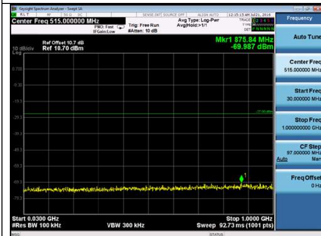
CUE-802.11a-5580M--chain2(30MHz-1GHz)
