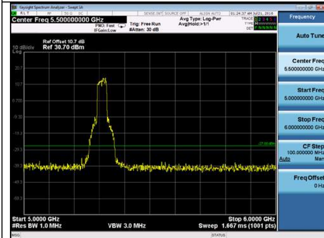
CUE-802.11n-40-5310M-chain3(5GHz-6GHz)
