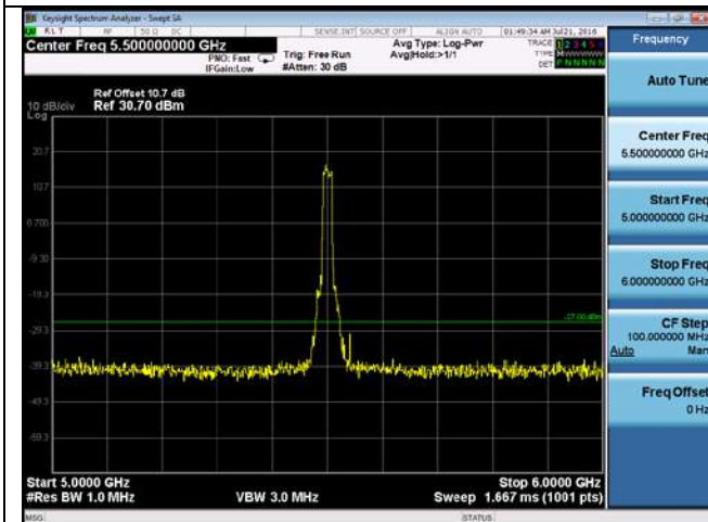
CUE-802.11n-20-5500M-chain4(5GHz-6GHz)
