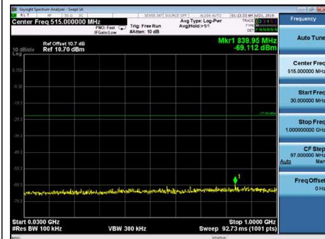
CUE-802.11n-20-5320M-chain 3(30MHz-1GHz)
