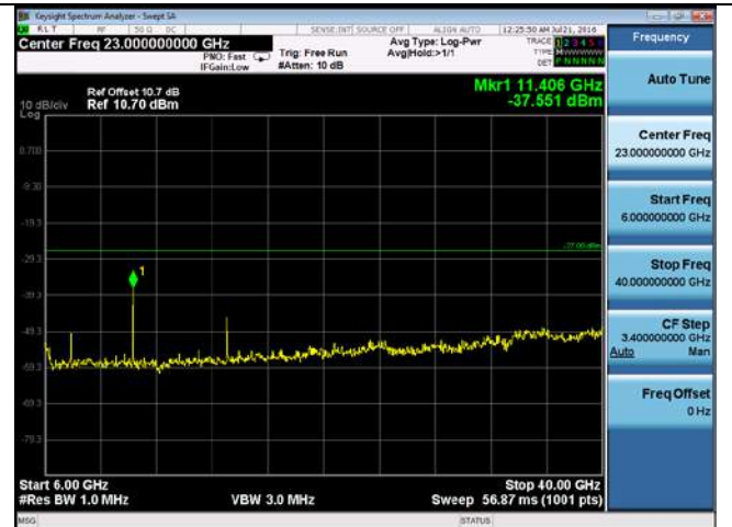
CUE-802.11n-20-5700M chain 2(6GHz-40GHz)
