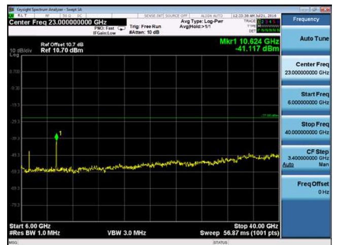
CUE-802.11n-40-5310M-chain2(6GHz-40GHz)
