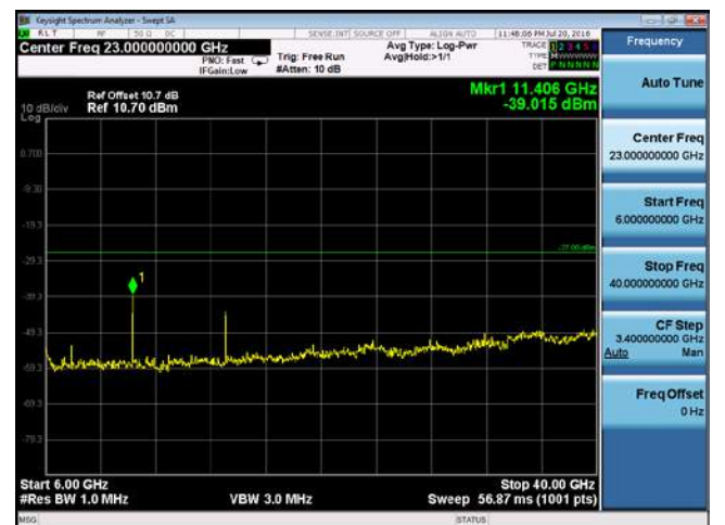
CUE-802.11n-20-5700M -chain 1(6GHz-40GHz)
