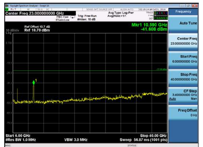
CUE-802.11ac-80-5290M-chain 4(6GHz-40GHz)
