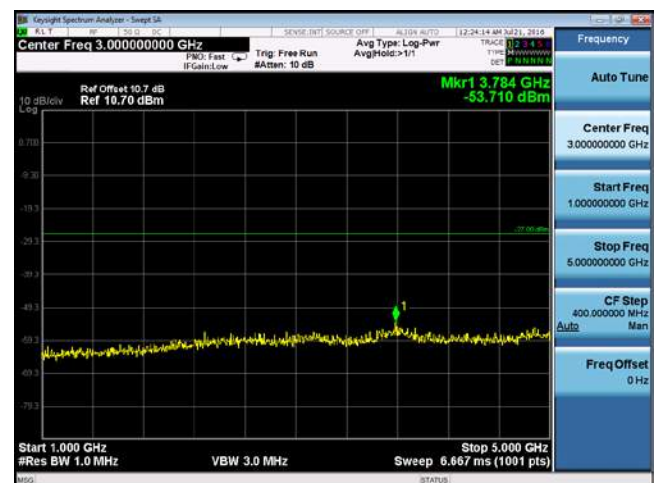
CUE-802.11n-20-5500M-chain2(1GHz-5GHz)
