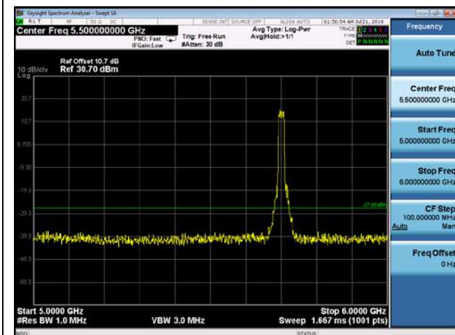
CUE-802.11a-5700M-chain 4(5GHz-6GHz)
