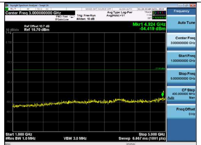
CUE-802.11n-40-5270M-chain3(1GHz-5GHz)
