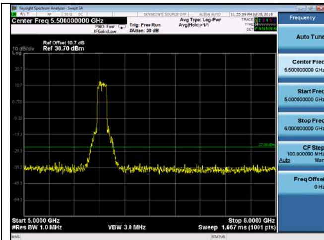
CUE-802.11n-40-5310M -chain1(5GHz-6GHz)
