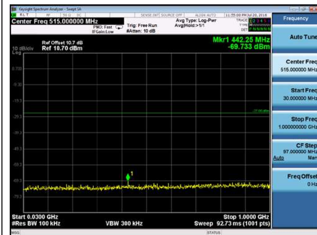
CUE-802.11n-40-5310M-chain1(30MHz-1GHz)
