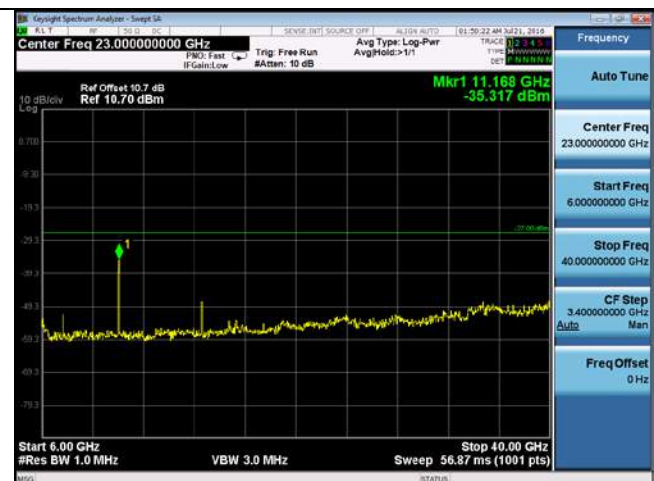
CUE-802.11a-5580M-chain 4(6GHz-40GHz)
