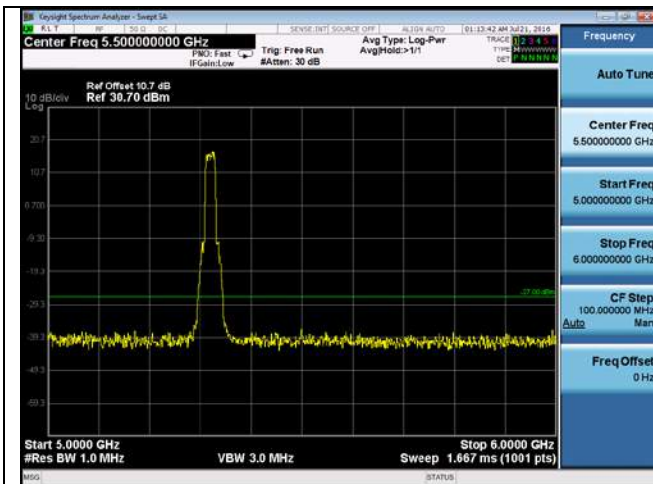
CUE-802.11n-20-5320M-chain 3(5GHz-6GHz)
