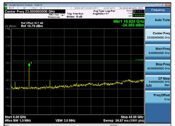
CUE-802.11n-40-5270M-chain3(6GHz-40GHz)
