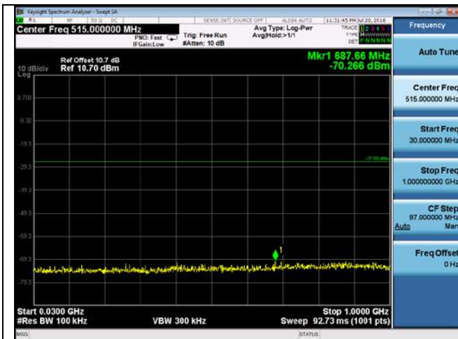
CUE-802.11a-5500M-chain1(30MHz-1GHz)
