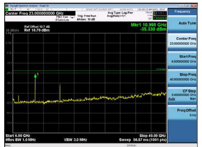
CUE-802.11a-5500M -chain3(6GHz-40GHz)
