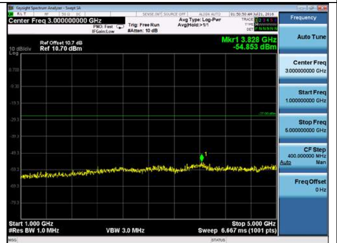
CUE-802.11a-5700M-chain 4(1GHz-5GHz)
