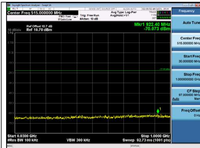
CUE-802.11n-40-5270M-chain4(30MHz-1GHz)
