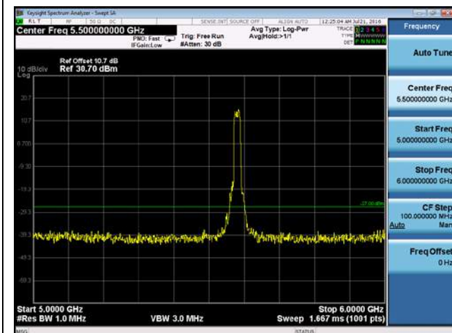
CUE-802.11n-20-5580M-chain2(5GHz-6GHz)
