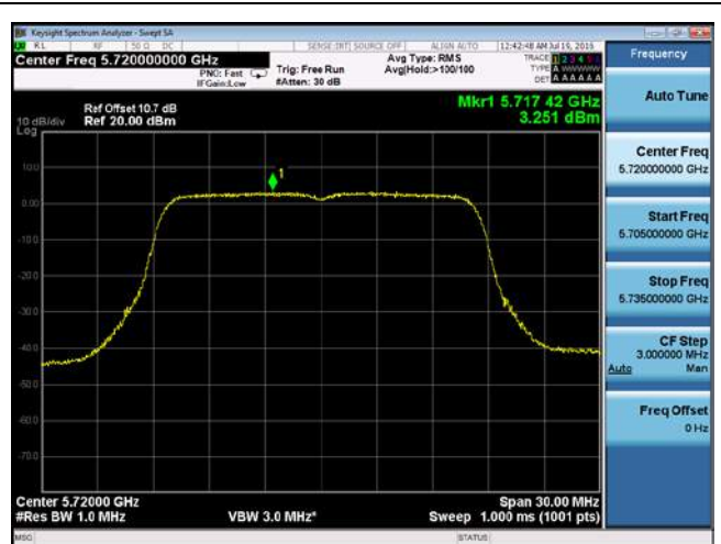
PSD-802.11a-CROSS-5720M-chain1
