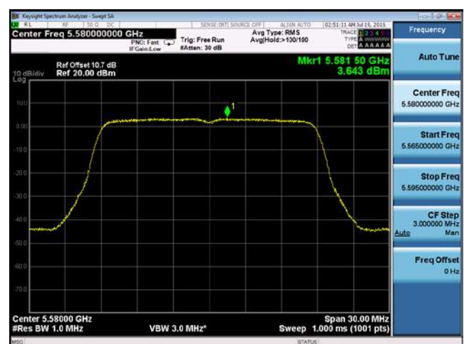
PSD-802.11n-20M-5580M-chain2
