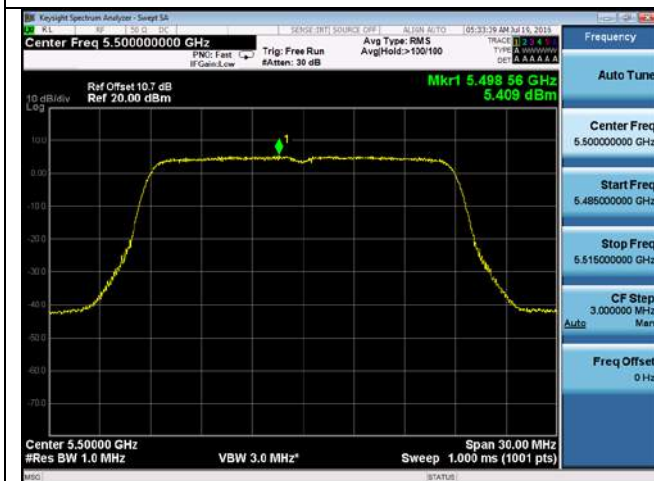
PSD-802.11n-20M-5500M-chain3
