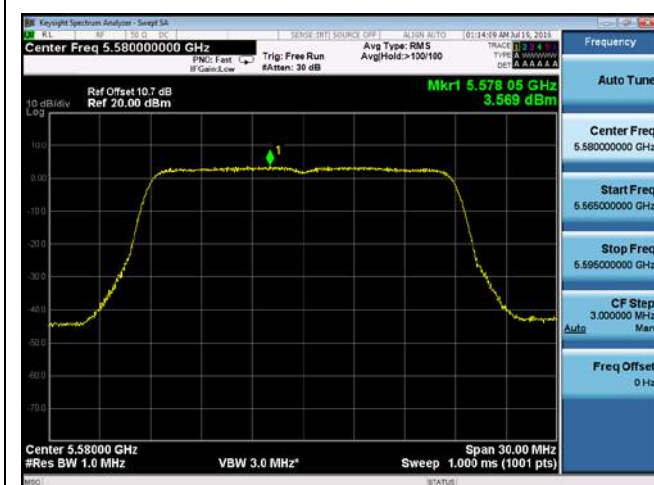
PSD-802.11n-20M-5580M-chain1
