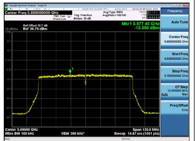
PSD-802.11ac-CROSS-5690M-chain2
