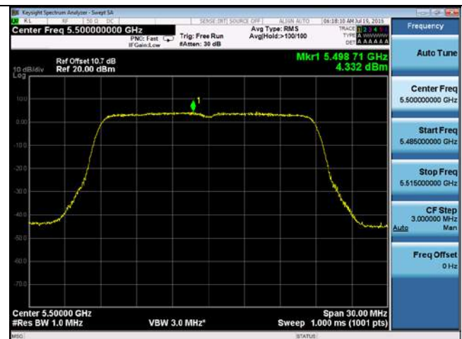
PSD-802.11n-20M-5500M-chain4
