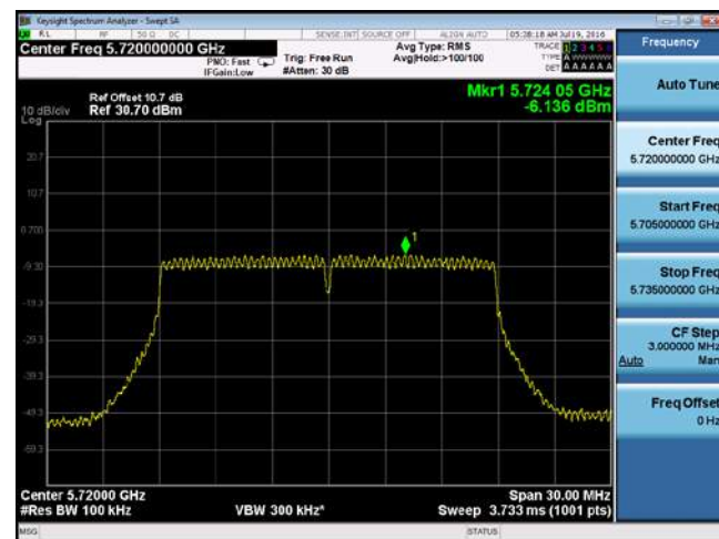
PSD-802.11n-20M-CROSS-5720M-chain3
