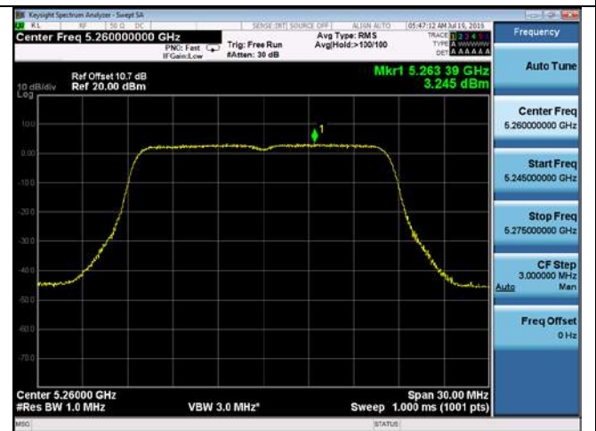
PSD-802.11a-5260M-chain4
