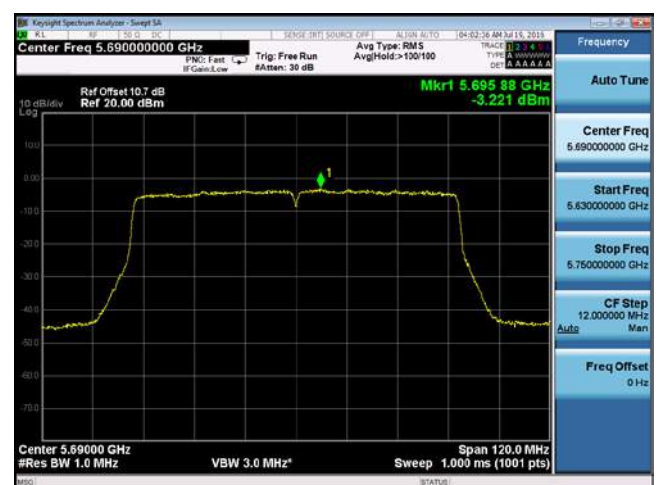
PSD-802.11ac-CROSS-5690M-chain2
