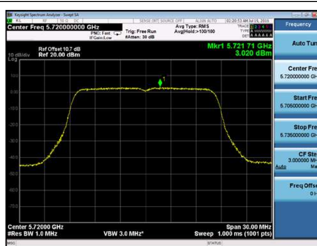
PSD-802.11a-CROSS-5720M-chain2
