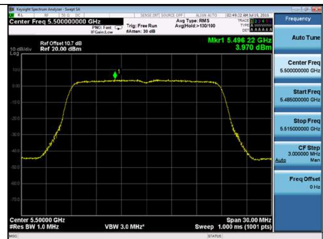
PSD-802.11n-20M-5500M-chain2
