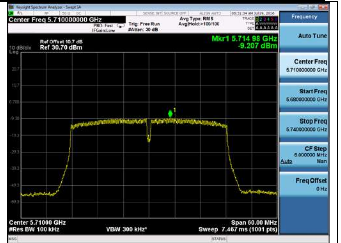
PSD-802.11n-40M-CROSS-5710M-chain4
