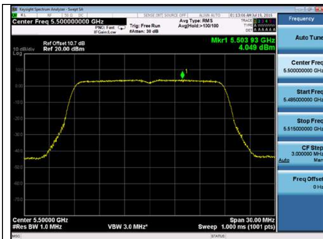
PSD-802.11n-20M-5500M-chain1
