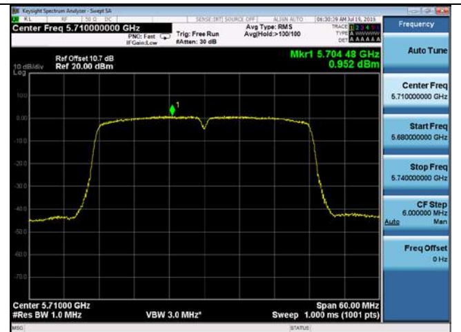
PSD-802.11n-40M-CROSS-5710M-chain4
