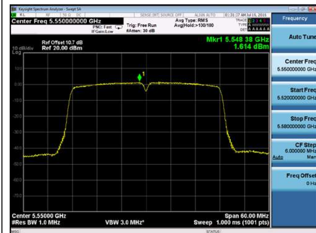
PSD-802.11n-40M-5550M-chain1
