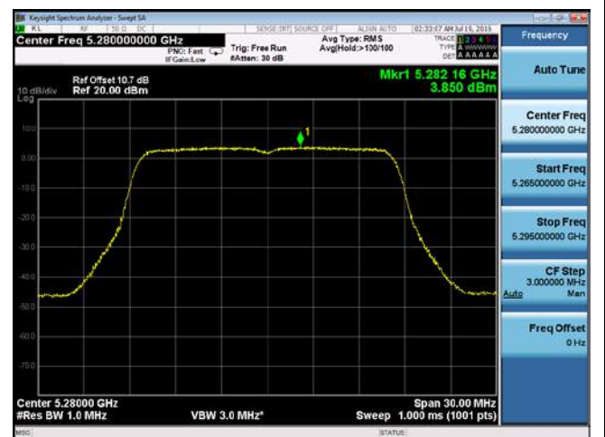
PSD-802.11a-5280M-chain2
