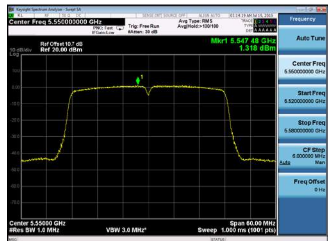
PSD-802.11n-40M-5550M-chain2
