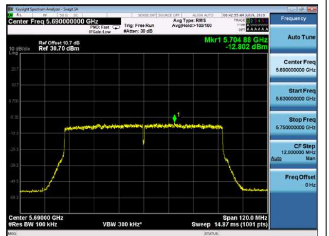
PSD-802.11ac-CROSS-5690M-chain4
