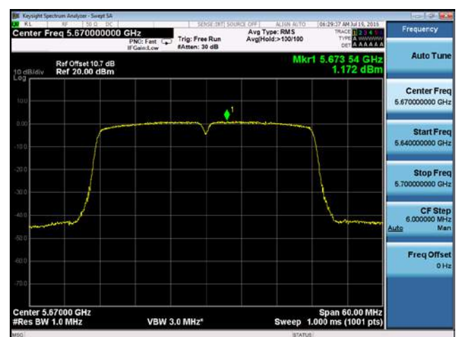
PSD-802.11n-40M-5670M-chain4
