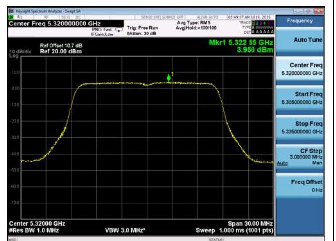
PSD-802.11a-5320M-chain4
