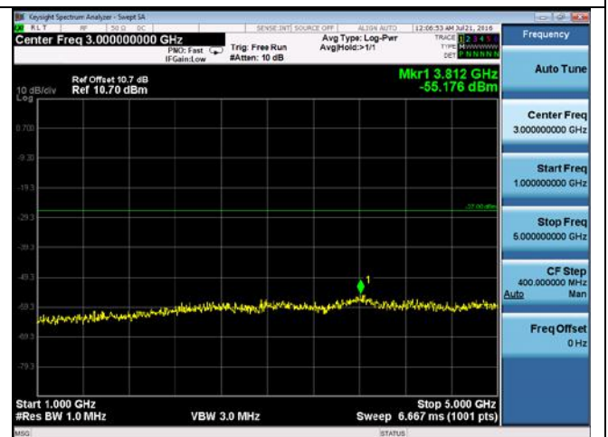
CUE-802.11ac-80-5775M-chain 1(1GHz-5GHz)
