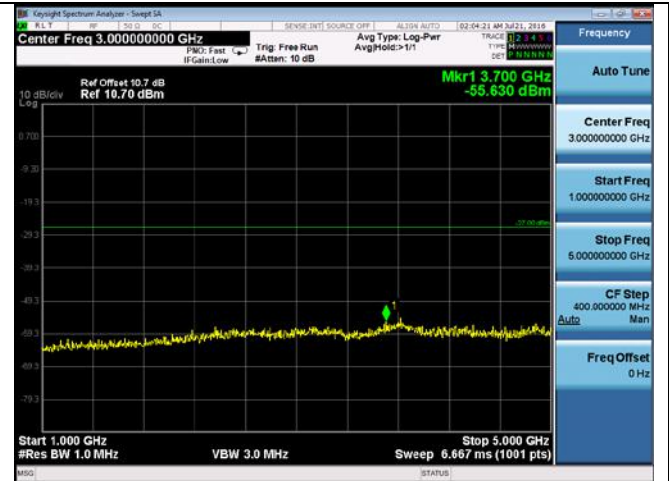
CUE-802.11n-20-5745M-chain4(1GHz-5GHz)
