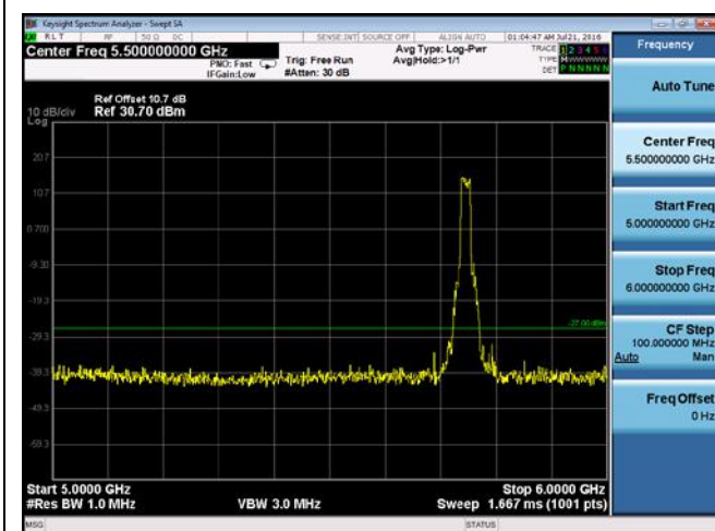
CUE-802.11a-5745M-chain3(5GHz-6GHz)
