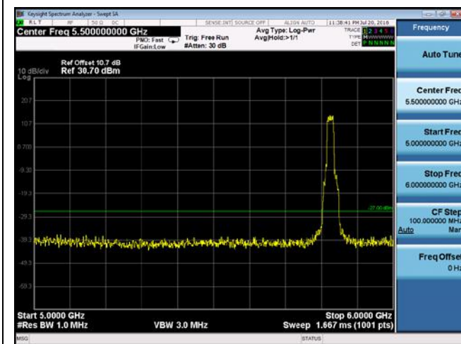
CUE-802.11a-5825M-chain 1(5GHz-6GHz)
