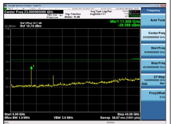
CUE-802.11a-5745M-chain3(6GHz-40GHz)
