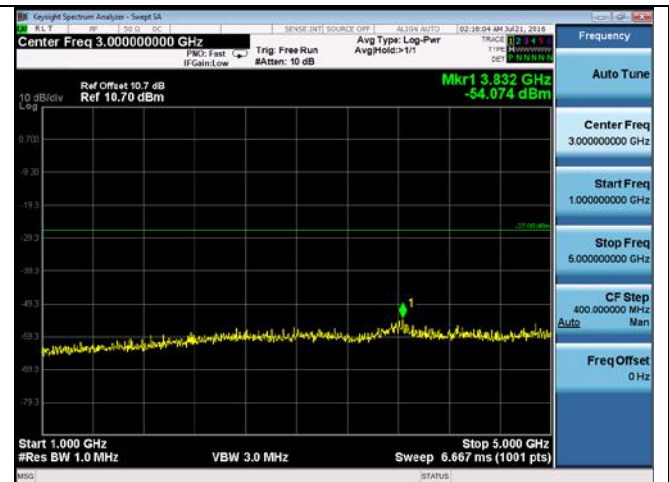
CUE-802.11n-40-5755M-chain4(1GHz-5GHz)
