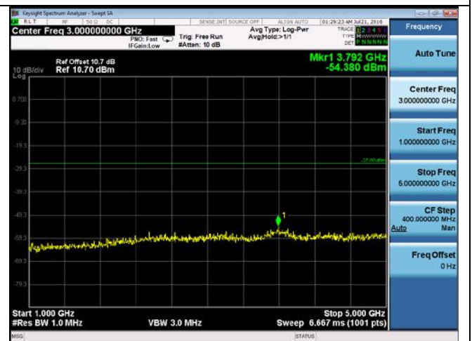
CUE-802.11n-40-5755M -chain3(1GHz-5GHz)
