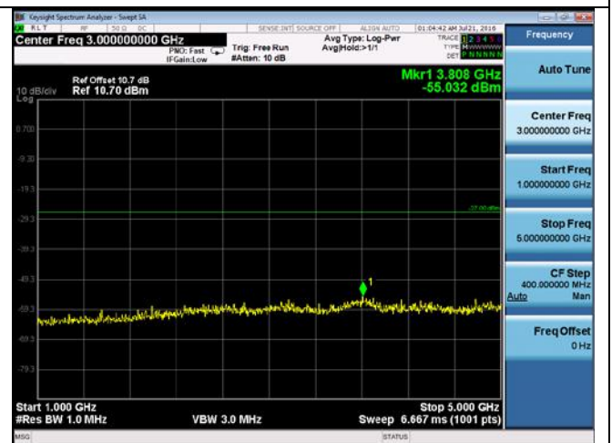
CUE-802.11a-5745M-chain3(1GHz-5GHz)
