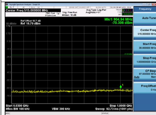
CUE-802.11a-5745M-chain3(30MHz-1GHz)
