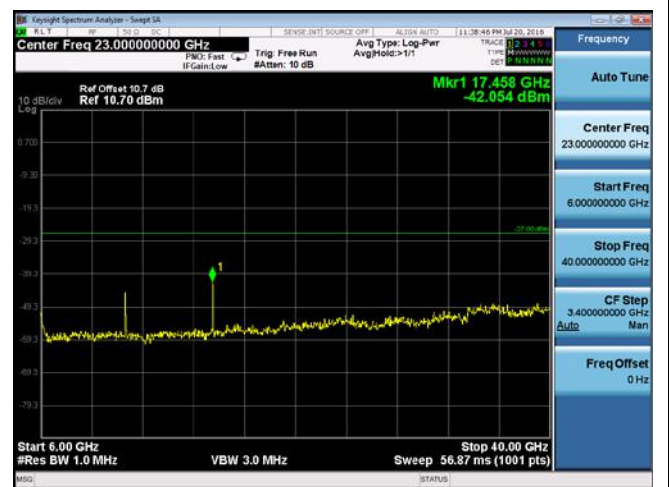
CUE-802.11a-5825M-chain 1(6GHz-40GHz)
