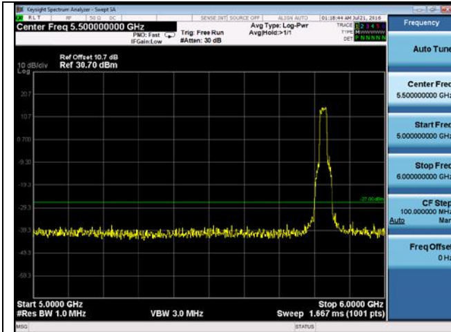
CUE-802.11n-20-5825M -chain 3(5GHz-6GHz)
