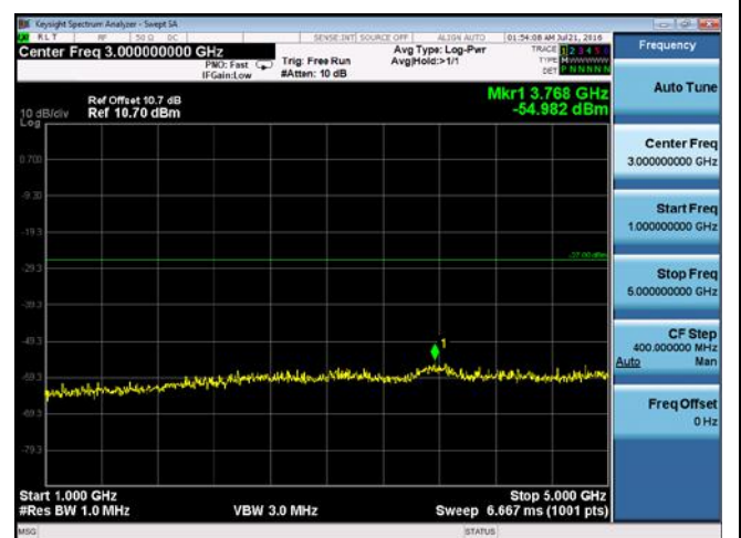
CUE-802.11a-5785M-chain4(1GHz-5GHz)
