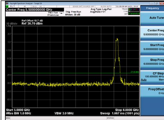
CUE-802.11a-5825M -chain 3(5GHz-6GHz)
