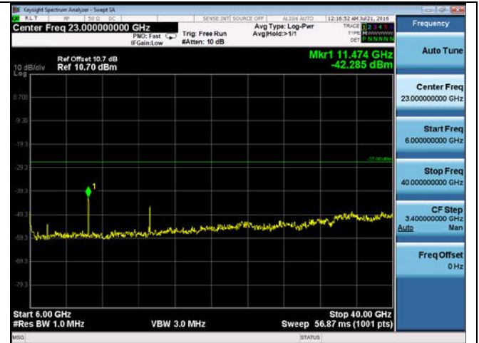
CUE-802.11a-5745M-chain2(6GHz-40GHz)
