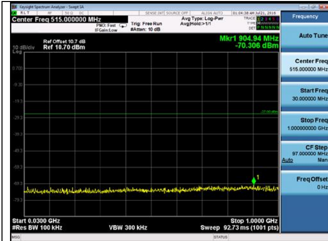
CUE-802.11a-5785M-chain3(30MHz-1GHz)
