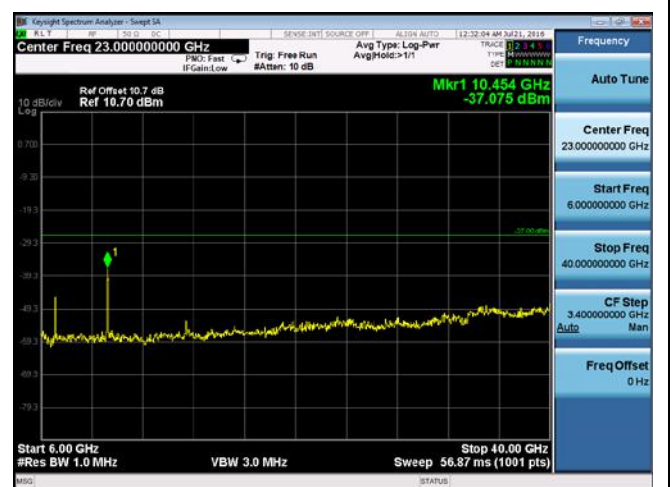
CUE-802.11n-40-5230M -chain2(6GHz-40GHz)
