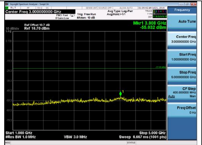
CUE-802.11a-5785M-chain3(1GHz-5GHz)
