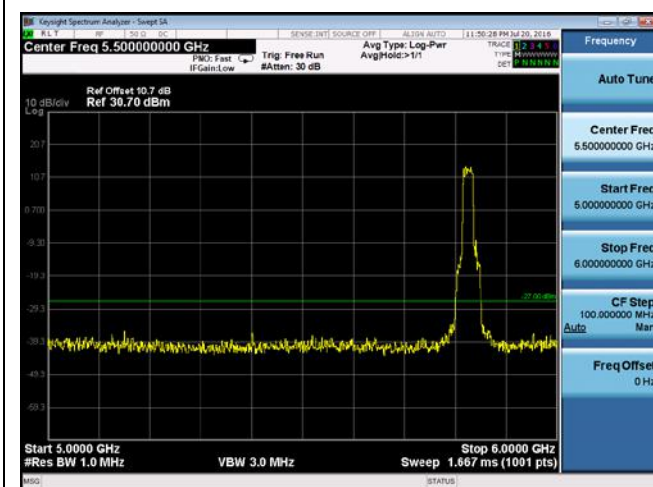
CUE-802.11n-20-5825M -chain 1(5GHz-6GHz)
