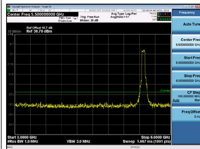
CUE-802.11n-20-5825M -chain 4(5GHz-6GHz)
