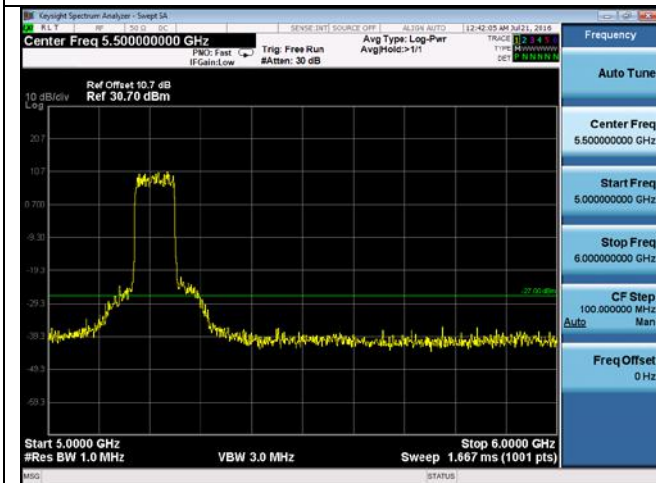
CUE-802.11ac-80-5210M -chain 2(5GHz-6GHz)
