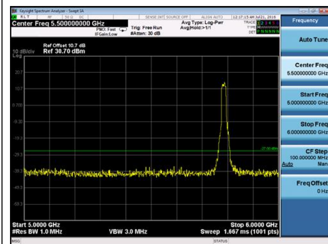
CUE-802.11a-5785M-chain2(5GHz-6GHz)
