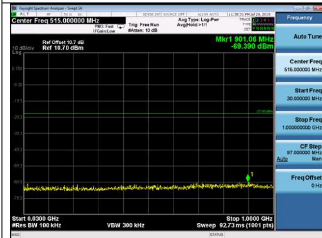
CUE-802.11a-5825M-chain 1(30MHz-1GHz)
