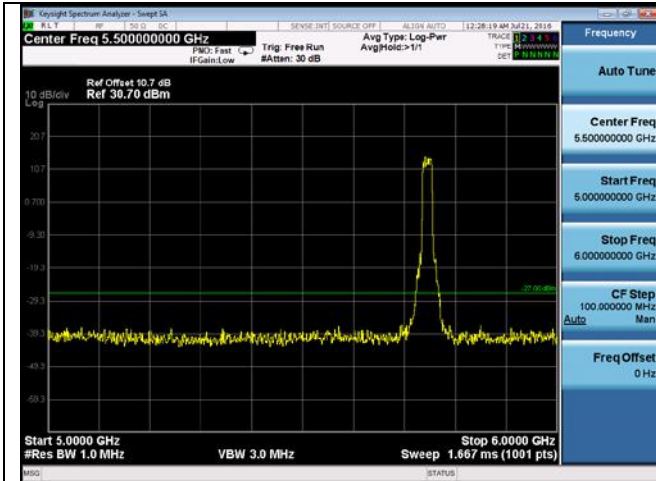
CUE-802.11n-20-5745M -chain2(5GHz-6GHz)
