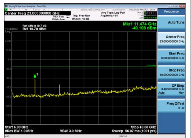
CUE-802.11n-20-5745M chain3(6GHz-40GHz)
