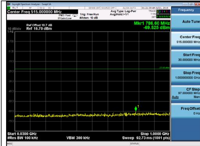
CUE-802.11n-40-5230M -chain3(30MHz-1GHz)
