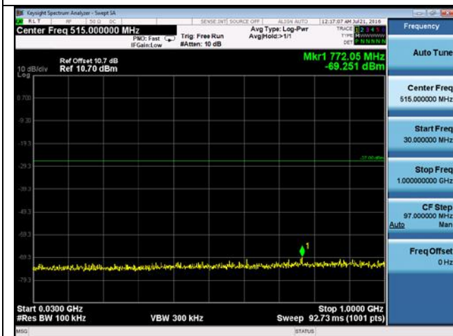
CUE-802.11a-5785M-chain2(30MHz-1GHz)
