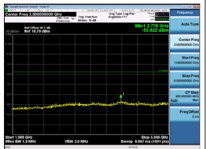
CUE-802.11a-5825M chain 3(1GHz-5GHz)
