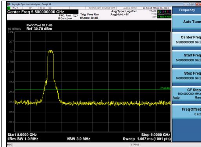
CUE-802.11n-40-5230M -chain1(5GHz-6GHz)
