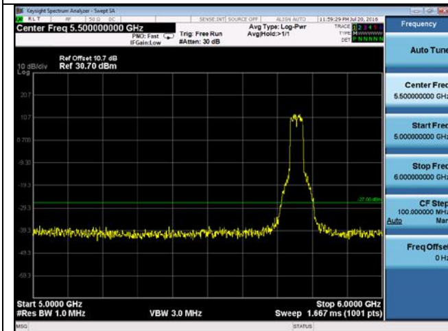
CUE-802.11n-40-5755M-chain1(5GHz-6GHz)
