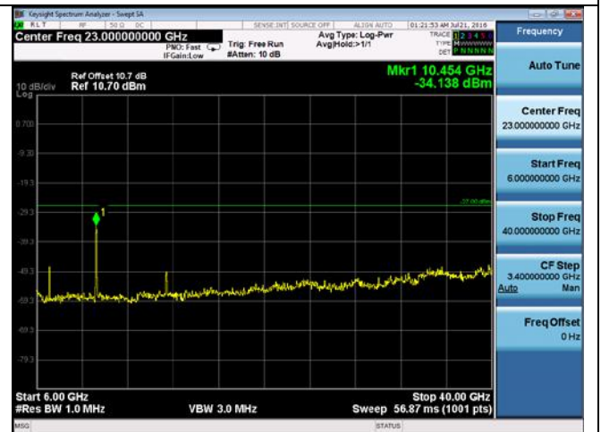
CUE-802.11n-40-5230M -chain3(6GHz-40GHz)
