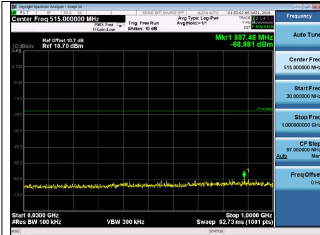
CUE-802.11a-5745M-chain4(30MHz-1GHz)
