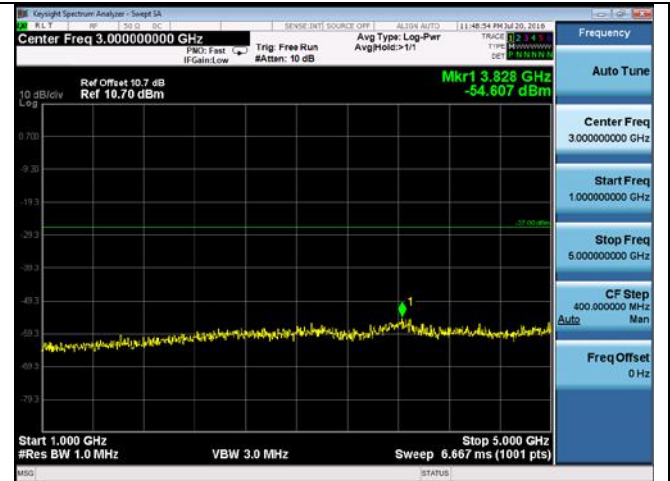
CUE-802.11n-20-5745M-chain1(1GHz-5GHz)
