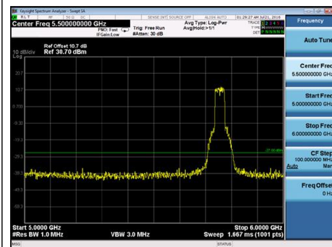
CUE-802.11n-40-5755M -chain3(5GHz-6GHz)
