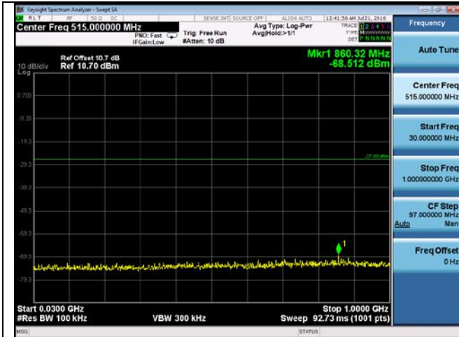
CUE-802.11ac-80-5210M -chain 2(30MHz-1GHz)
