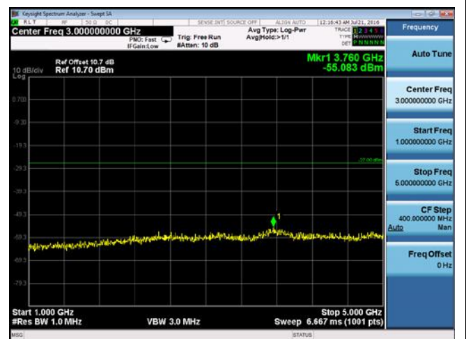
CUE-802.11a-5745M-chain2(1GHz-5GHz)
