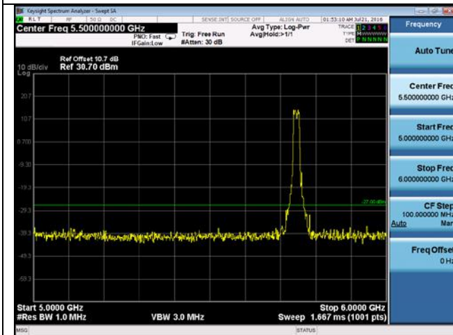
CUE-802.11a-5745M-chain4(5GHz-6GHz)
