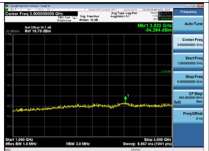
CUE-802.11n-20-5825M -chain 4(1GHz-5GHz)
