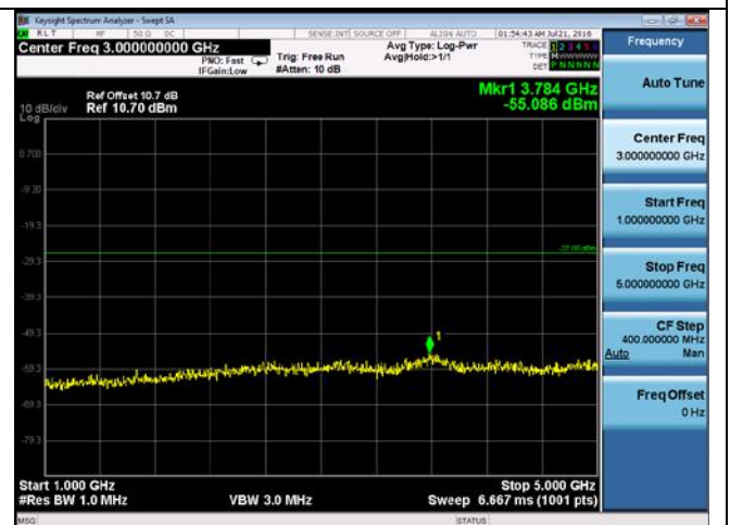
CUE-802.11a-5825M -chain 4(1GHz-5GHz)
