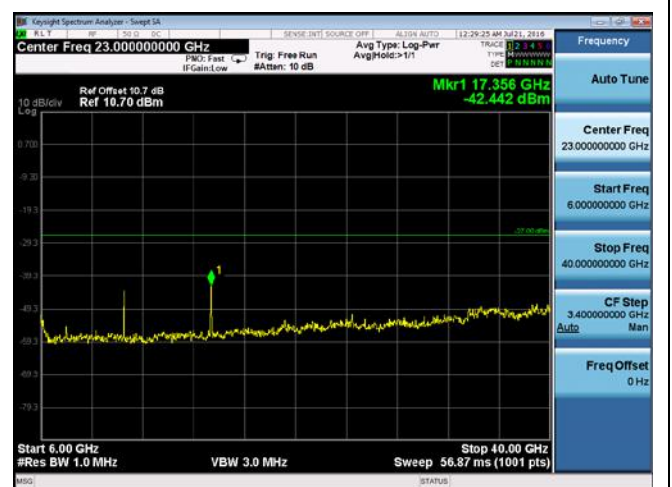
CUE-802.11n-20-5785M -chain2(6GHz-40GHz)
