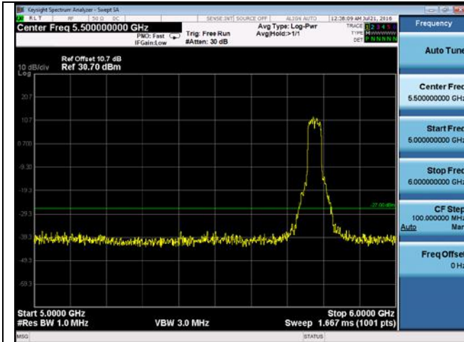
CUE-802.11n-40-5755M -chain2(5GHz-6GHz)
