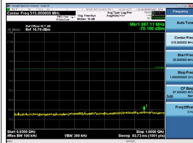
CUE-802.11a-5745M-chain2(30MHz-1GHz)
