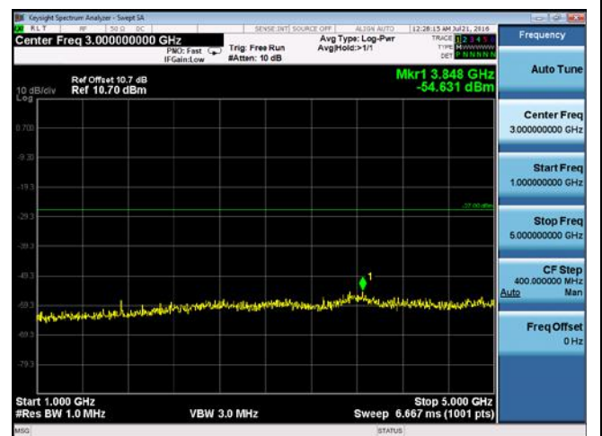
CUE-802.11n-20-5745M-chain2(1GHz-5GHz)
