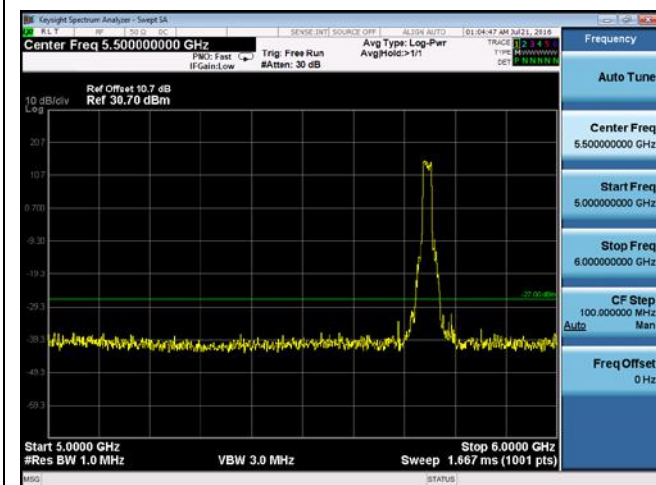
CUE-802.11a-5745M-chain3(5GHz-6GHz)
