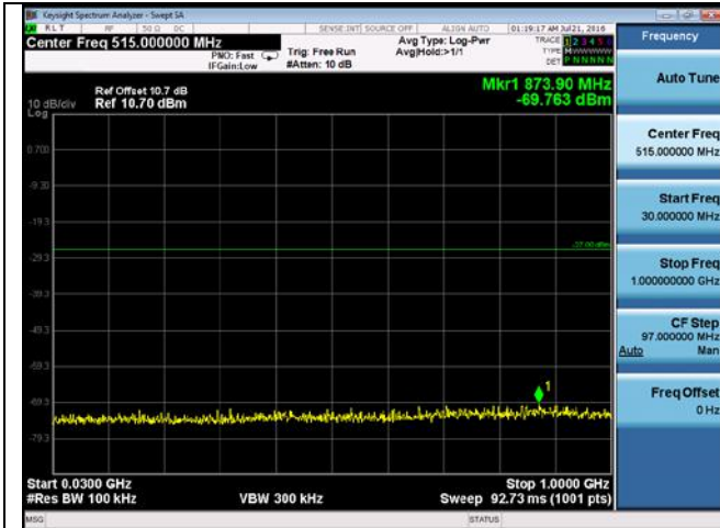
CUE-802.11n-20-5785M chain3(30MHz-1GHz)
