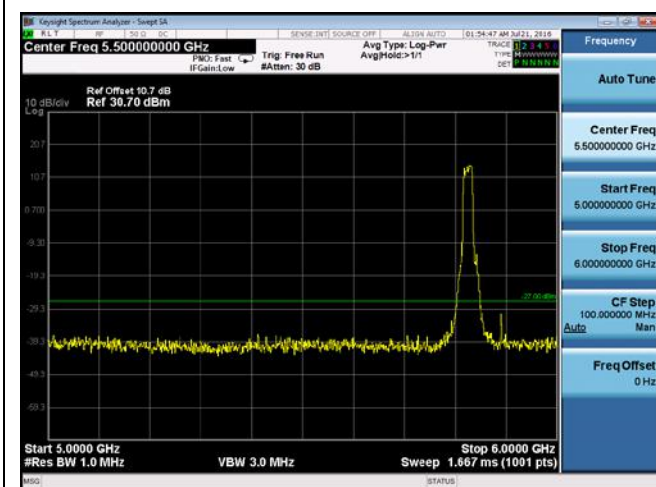
CUE-802.11a-5825M -chain 4(5GHz-6GHz)
