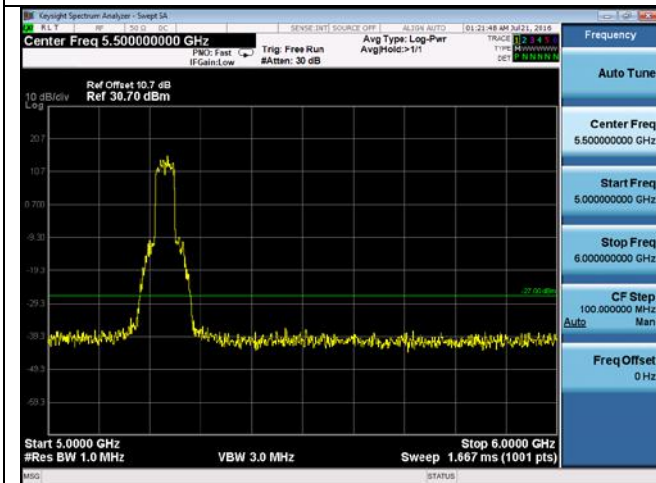
CUE-802.11n-40-5230M chain3(5GHz-6GHz)
