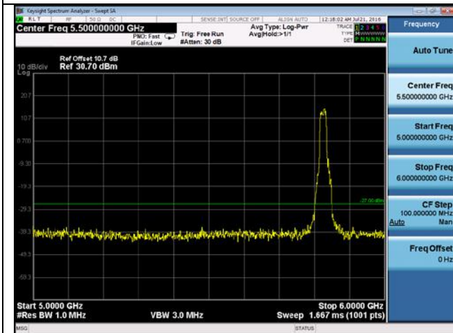
CUE-802.11a-5825M -chain 2(5GHz-6GHz)
