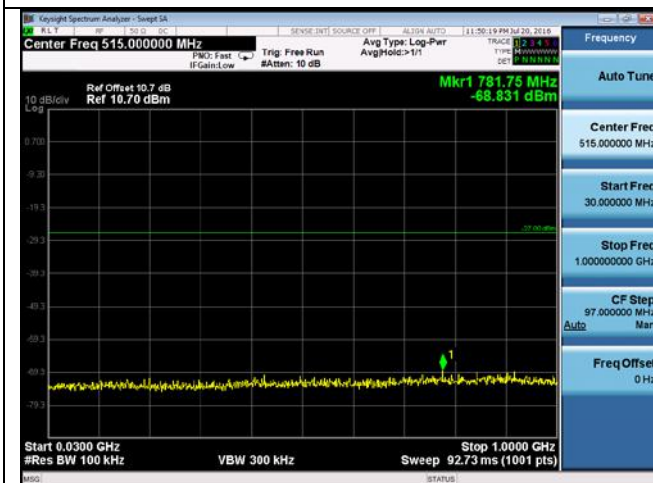
CUE-802.11n-20-5825M -chain 1(30MHz-1GHz)
