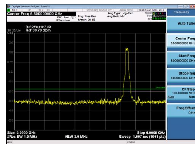
CUE-802.11n-20-5745M -chain3(5GHz-6GHz)
