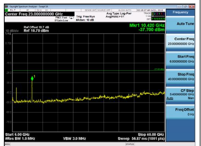
CUE-802.11ac-80-5210M chain 4 (6GHz-40GHz)
