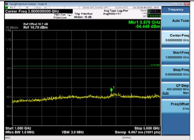
CUE-802.11a-5745M-chain4(1GHz-5GHz)
