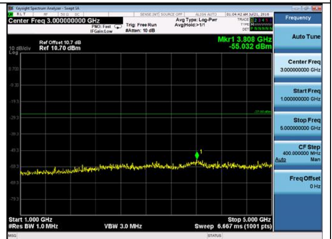
CUE-802.11a-5745M-chain3(1GHz-5GHz)
