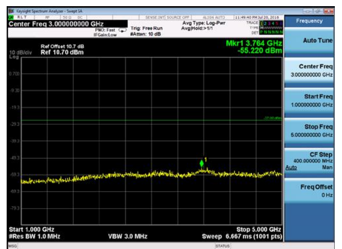
CUE-802.11n-20-5785M-chain1(1GHz-5GHz)
