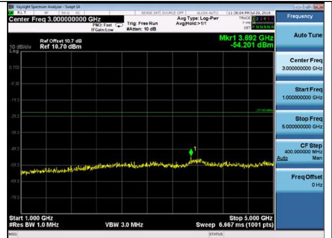
CUE-802.11a-5745M-chain1(1GHz-5GHz)
