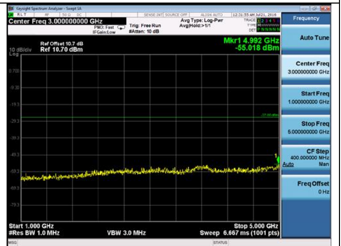
CUE-802.11n-40-5230M chain2(1GHz-5GHz)
