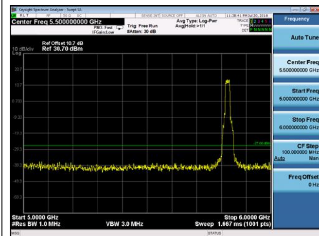
CUE-802.11a-5825M-chain 1(5GHz-6GHz)
