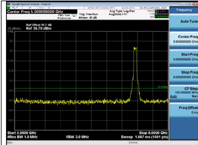
CUE-802.11a-5785M-chain 4(5GHz-6GHz)
