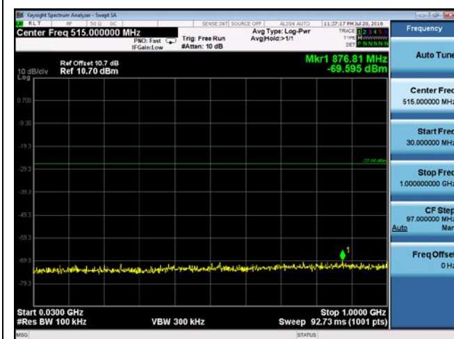
CUE-802.11a-5785M-chain1(30MHz-1GHz)
