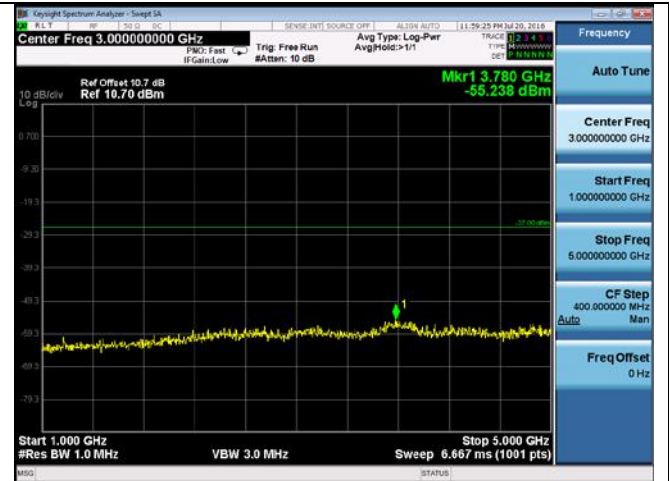
CUE-802.11n-40-5755M-chain1(1GHz-5GHz)
