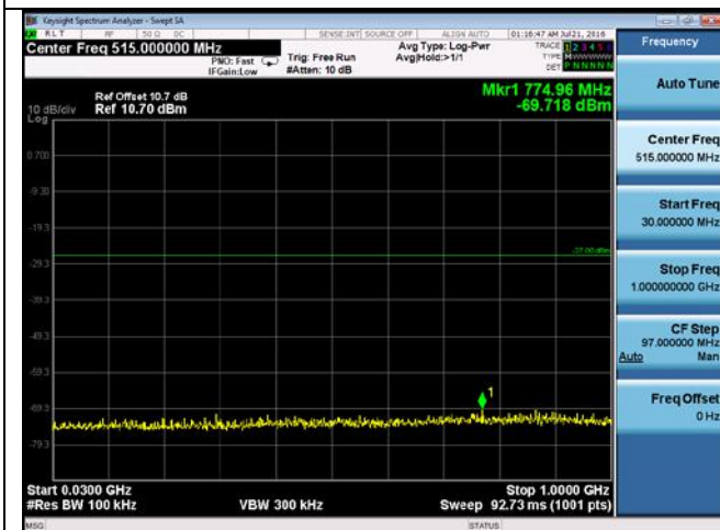
CUE-802.11n-20-5745M -chain3(30MHz-1GHz)
