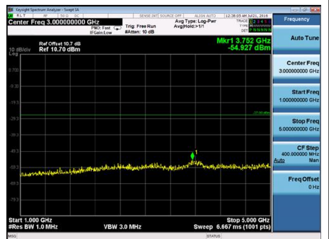
CUE-802.11n-40-5755M-chain2(1GHz-5GHz)
