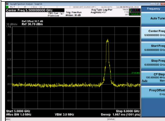
CUE-802.11n-20-5745M-chain1(5GHz-6GHz)
