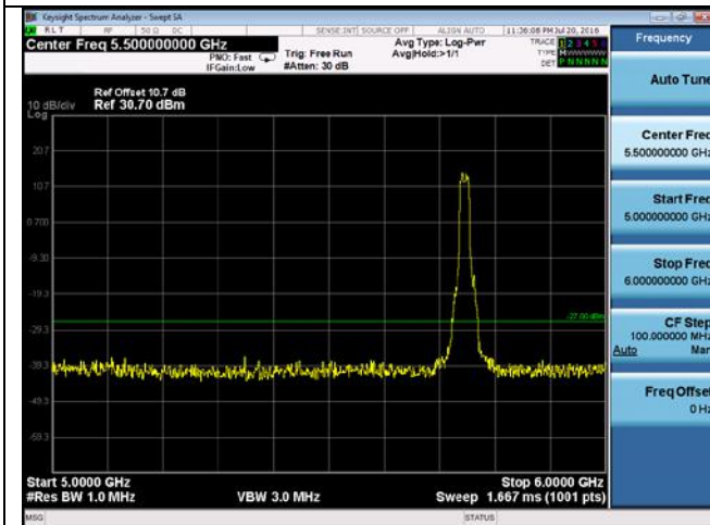
CUE-802.11a-5745M-chain1(5GHz-6GHz)
