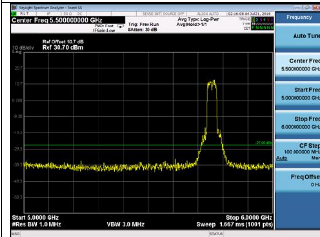
CUE-802.11n-40-5755M-chain4(5GHz-6GHz)
