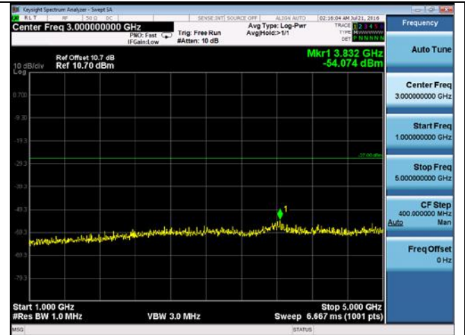
CUE-802.11n-40-5755M-chain4(1GHz-5GHz)
