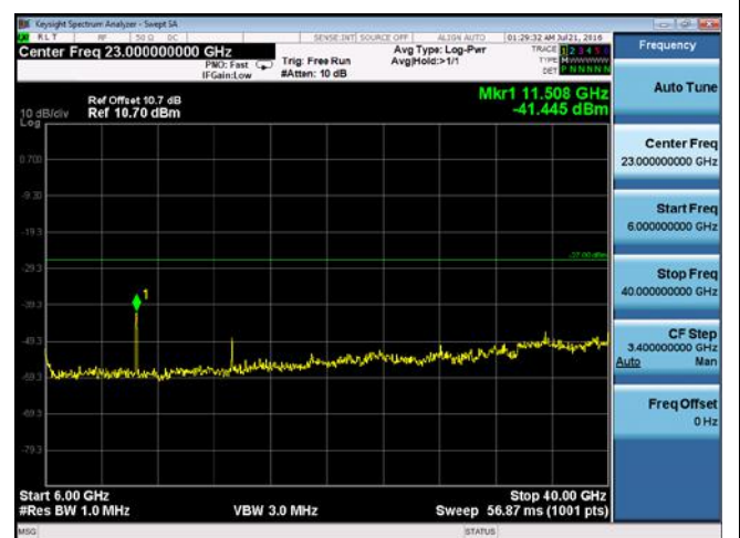
CUE-802.11n-40-5755M -chain3(6GHz-40GHz)
