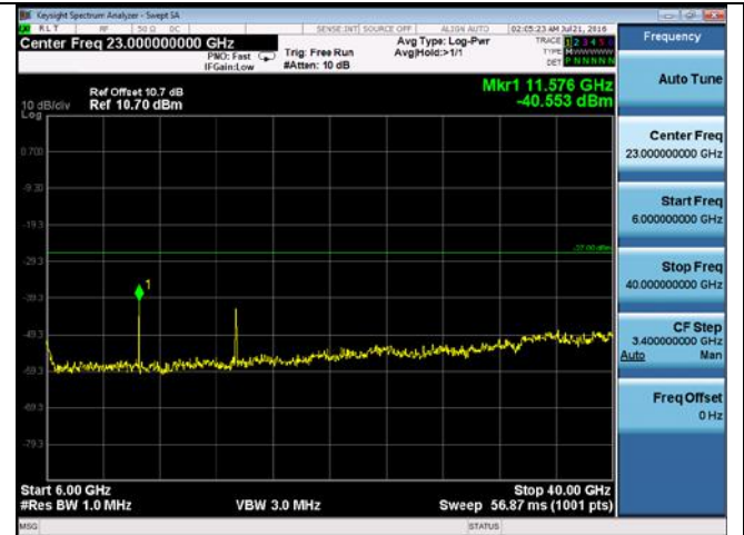
CUE-802.11n-20-5785M -chain 4(6GHz-40GHz)
