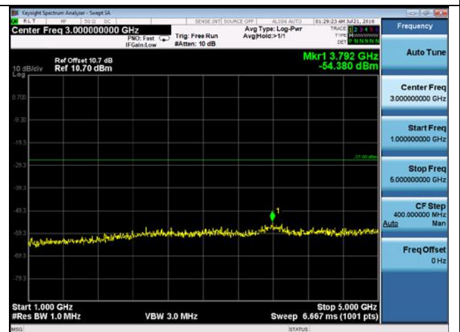
CUE-802.11n-40-5755M -chain3(1GHz-5GHz)
