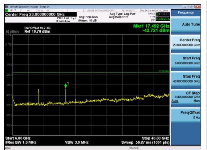
CUE-802.11a-5825M -chain 4(6GHz-40GHz)
