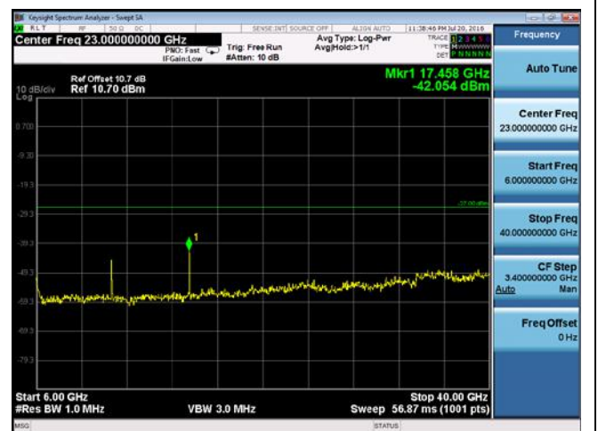
CUE-802.11a-5825M-chain 1(6GHz-40GHz)
