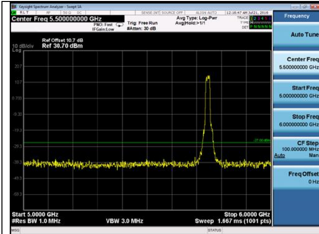
CUE-802.11a-5745M-chain2(5GHz-6GHz)
