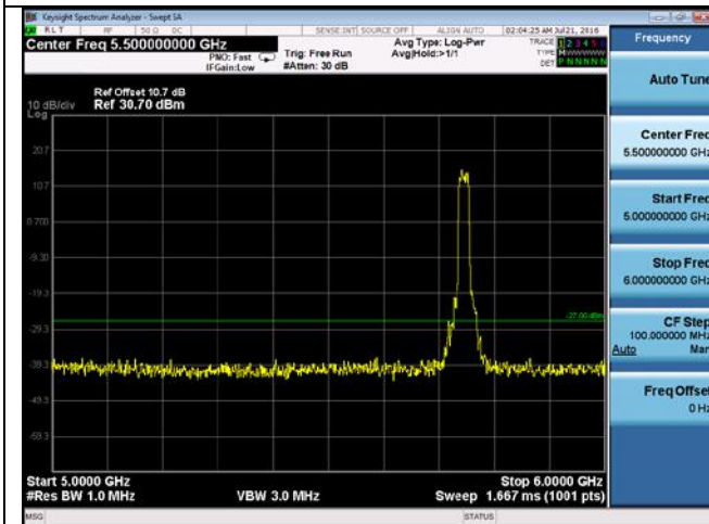
CUE-802.11n-20-5745M-chain4(5GHz-6GHz)
