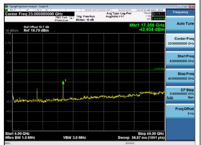
CUE-802.11a-5785M-chain2(6GHz-40GHz)
