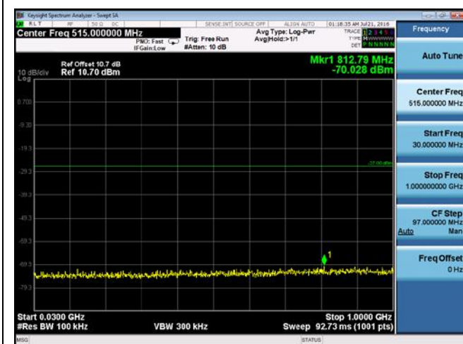
CUE-802.11n-20-5825M -chain 3(30MHz-1GHz)
