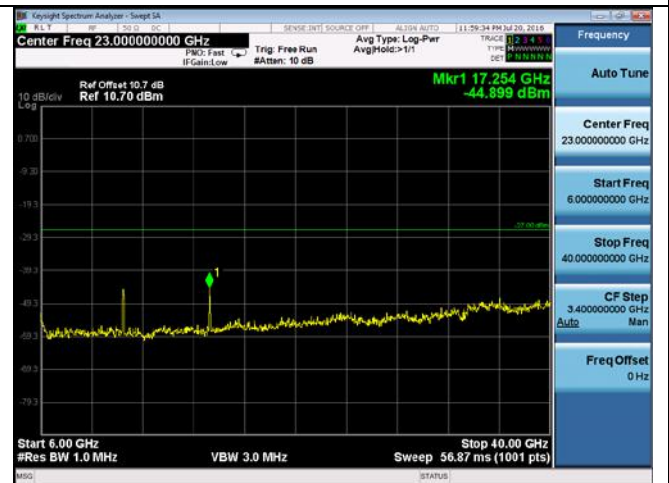
CUE-802.11n-40-5755M-chain1(6GHz-40GHz)
