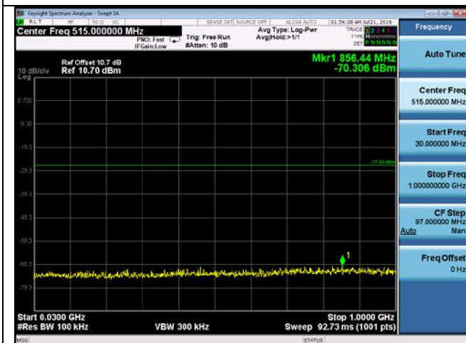
CUE-802.11a-5825M -chain 4(30MHz-1GHz)
