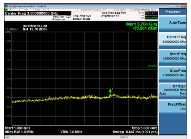
CUE-802.11a-5785M-chain1(1GHz-5GHz)
