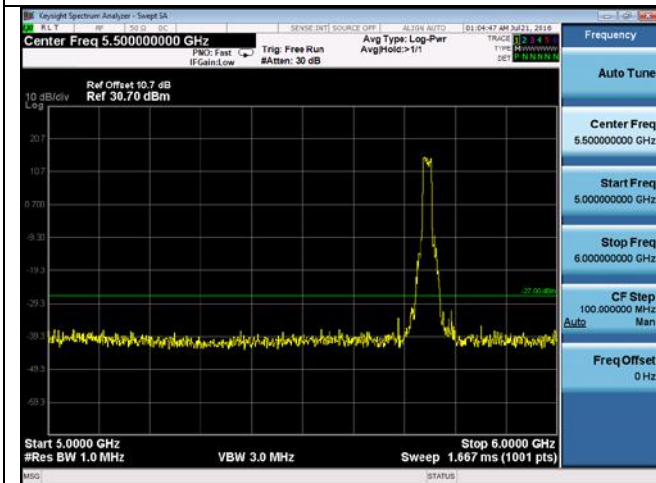
CUE-802.11a-5785M-chain3(5GHz-6GHz)
