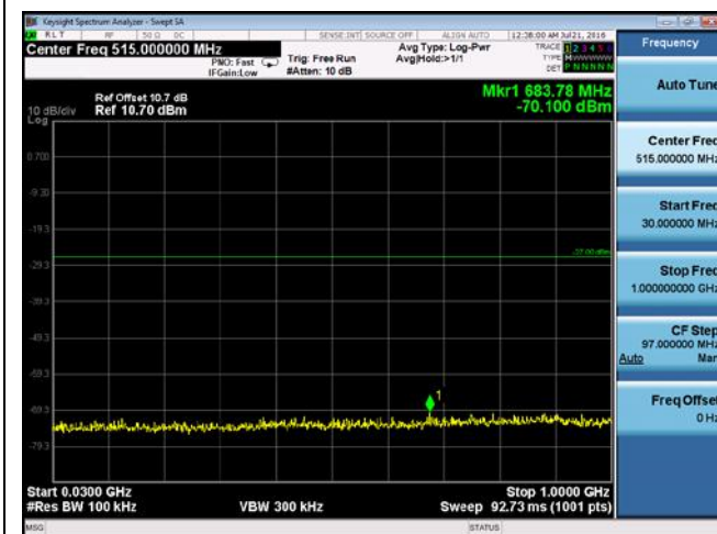
CUE-802.11n-40-5755M-chain2(30MHz-1GHz)
