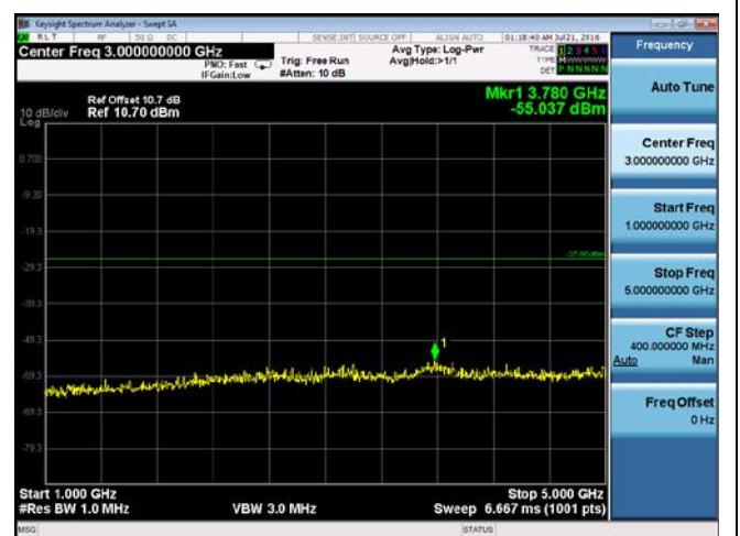
CUE-802.11n-20-5825M -chain 3(1GHz-5GHz)
