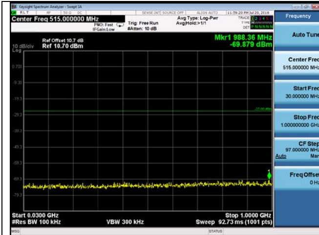
CUE-802.11n-40-5755M-chain1(30MHz-1GHz)
