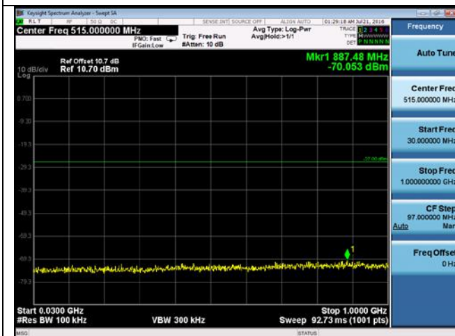
CUE-802.11n-40-5755M -chain3(30MHz-1GHz)
