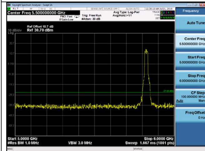
CUE-802.11n-20-5825M -chain 2(5GHz-6GHz)
