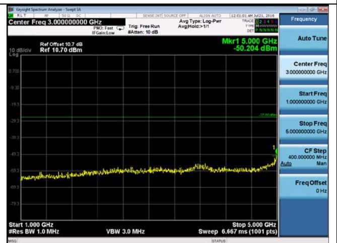
CUE-802.11ac-80-5210M-chain 1(1GHz-5GHz)
