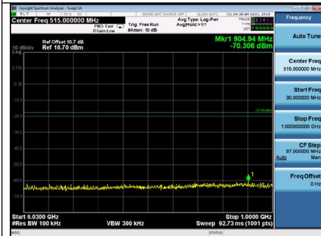
CUE-802.11a-5745M-chain3(30MHz-1GHz)
