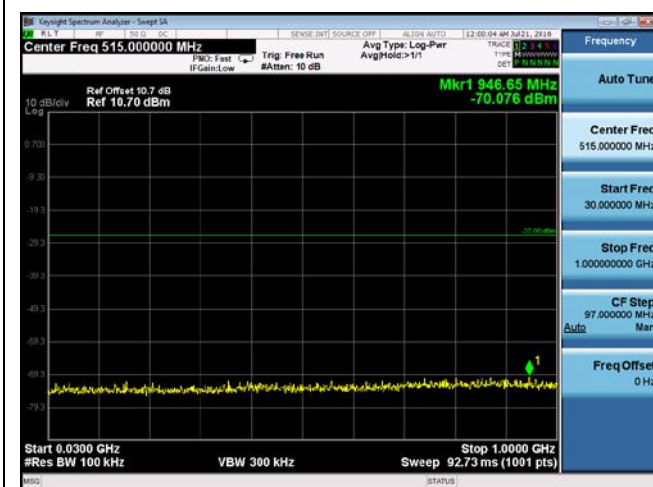
CUE-802.11n-40-5795M-chain1(30MHz-1GHz)
