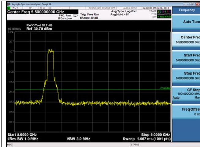
CUE-802.11n-40-5230M-chain 4(5GHz-6GHz)
