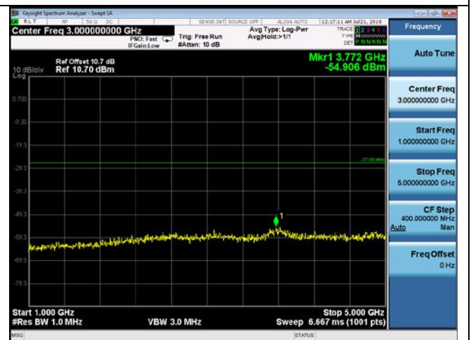
CUE-802.11a-5785M-chain2(1GHz-5GHz)
