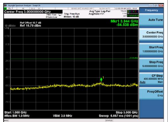
CUE-802.11n-40-5795M-chain1(1GHz-5GHz)
