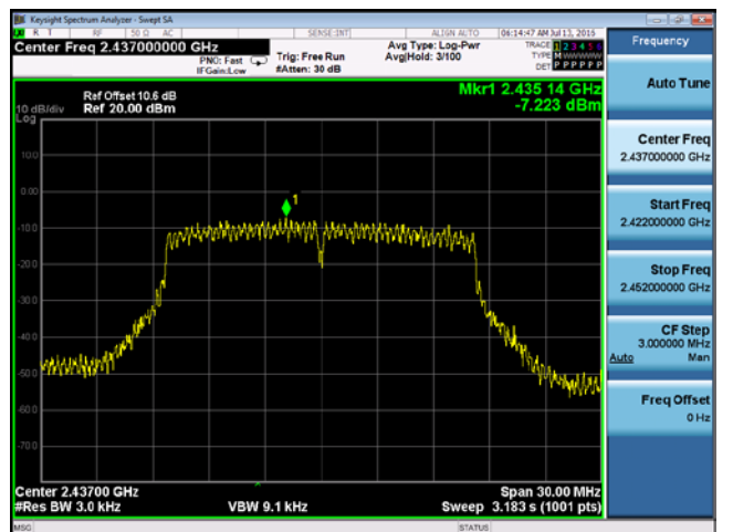
PSD-2.4G-802.11g Mid-chain2
