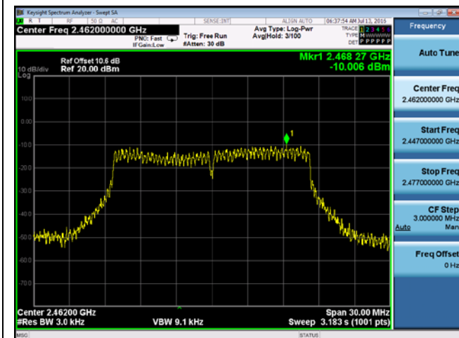
PSD-2.4G-802.11g High-chain3
