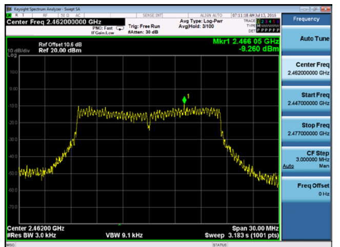
PSD-2.4G-802.11g High-chain4
