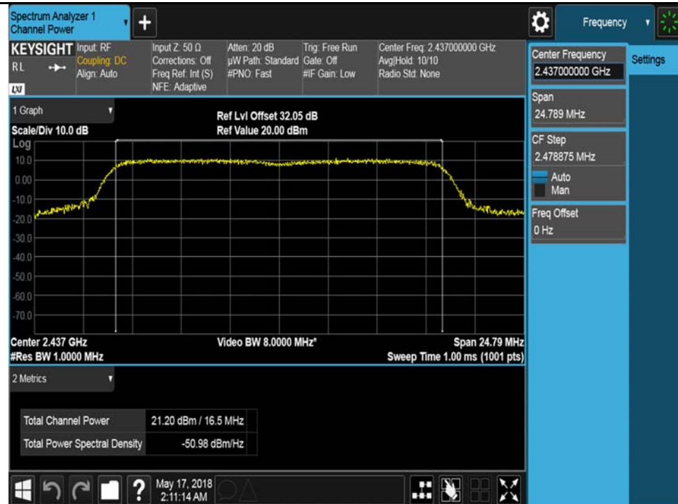
802.11g-2437MHz Chain 3
