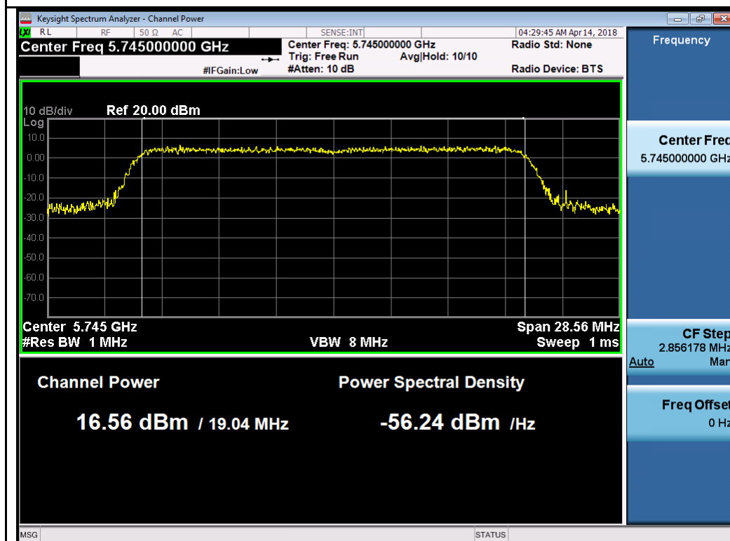
802.11ax20 5745M
