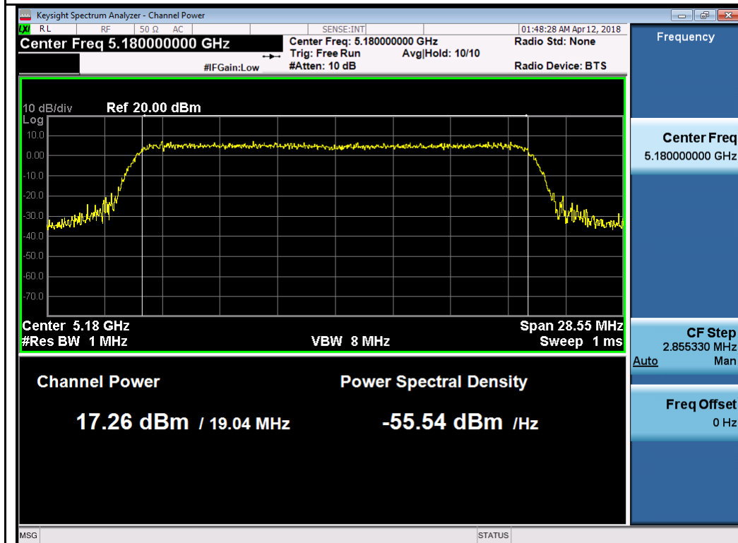
802.11ax20 5180M
