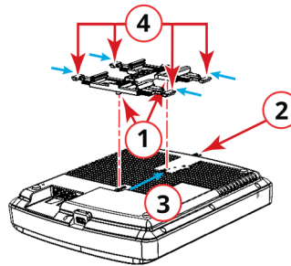
FIGURE 7 Attaching the T-bar Bracket to the AP
