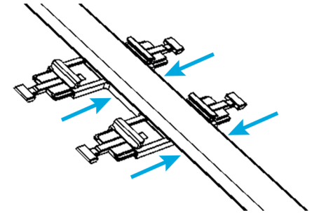
FIGURE 8 Attaching the T-bar Bracket to the T-bar
