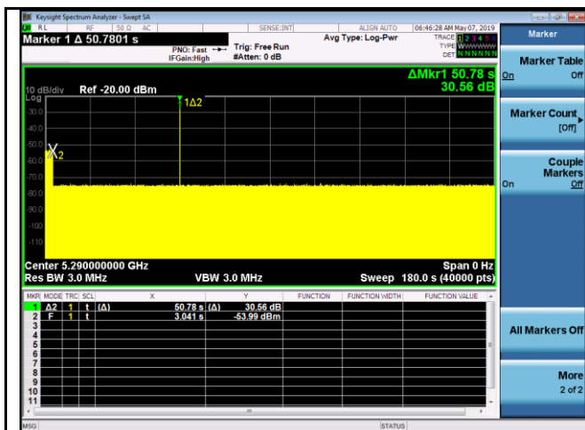
Radar at beginning of CAC – 802.11ax-80 – 5290MHz
