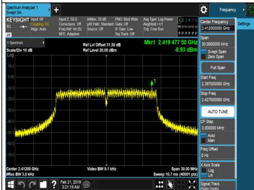
802.11g-2412MHz Chain 3
