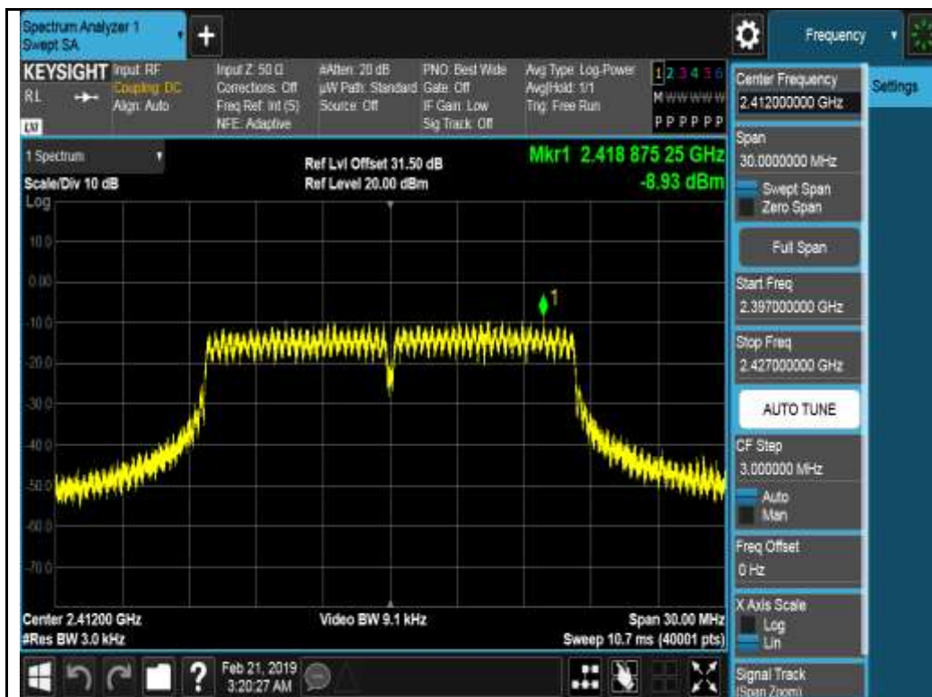
802.11g-2412MHz Chain 2
