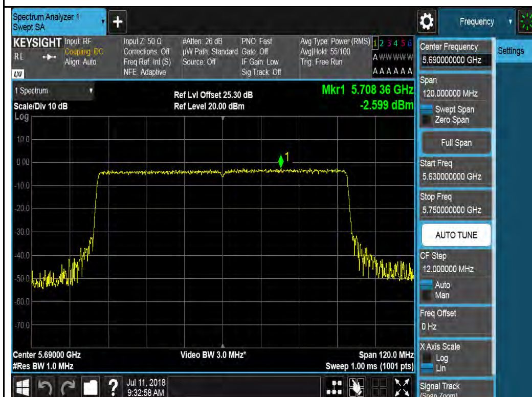
802.11ac-VHT80 5690M
