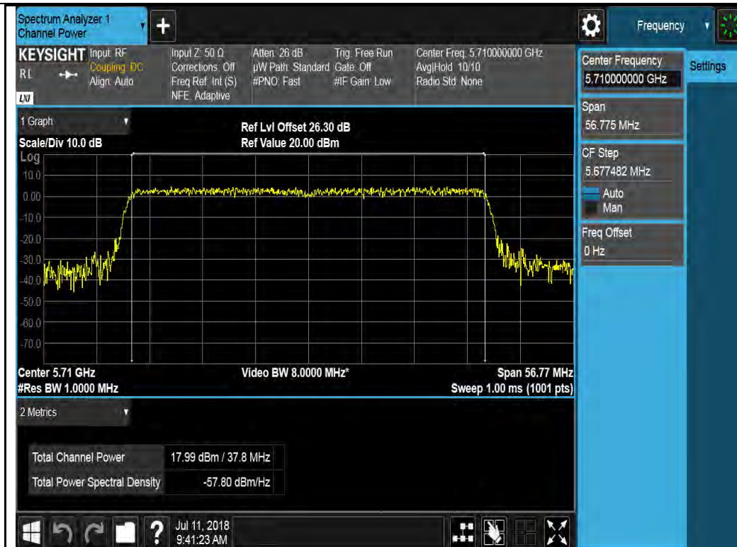
802.11n-HT40 5710M
