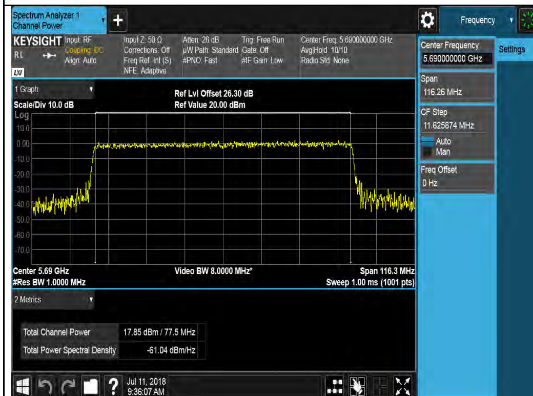
802.11ac-VHT80 5690M
