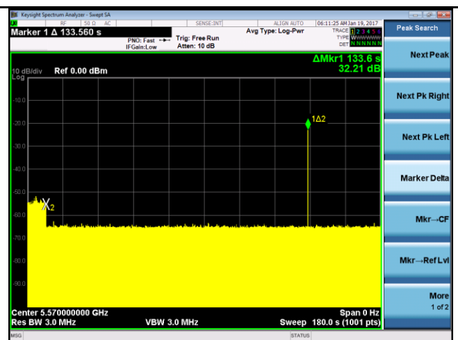
Radar at end of CAC – VHT160 – 5570MHz
