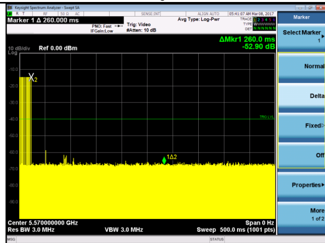
Channel Move Time& Closing Time - 802.11ac-5570MHz 260ms
