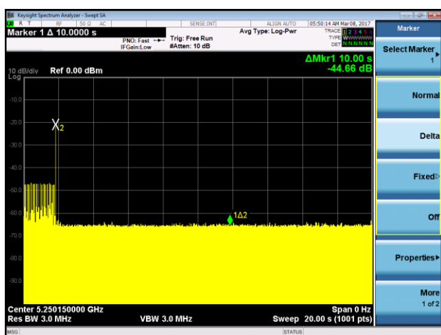
Channel Move Time& Closing Time - 802.11ac-5250MHz 10s
