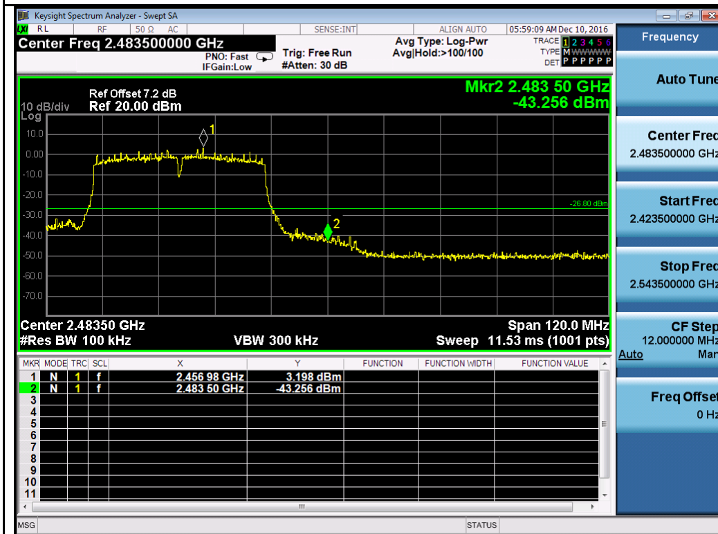
802.11n-HT40-2452MHz Chain 4
