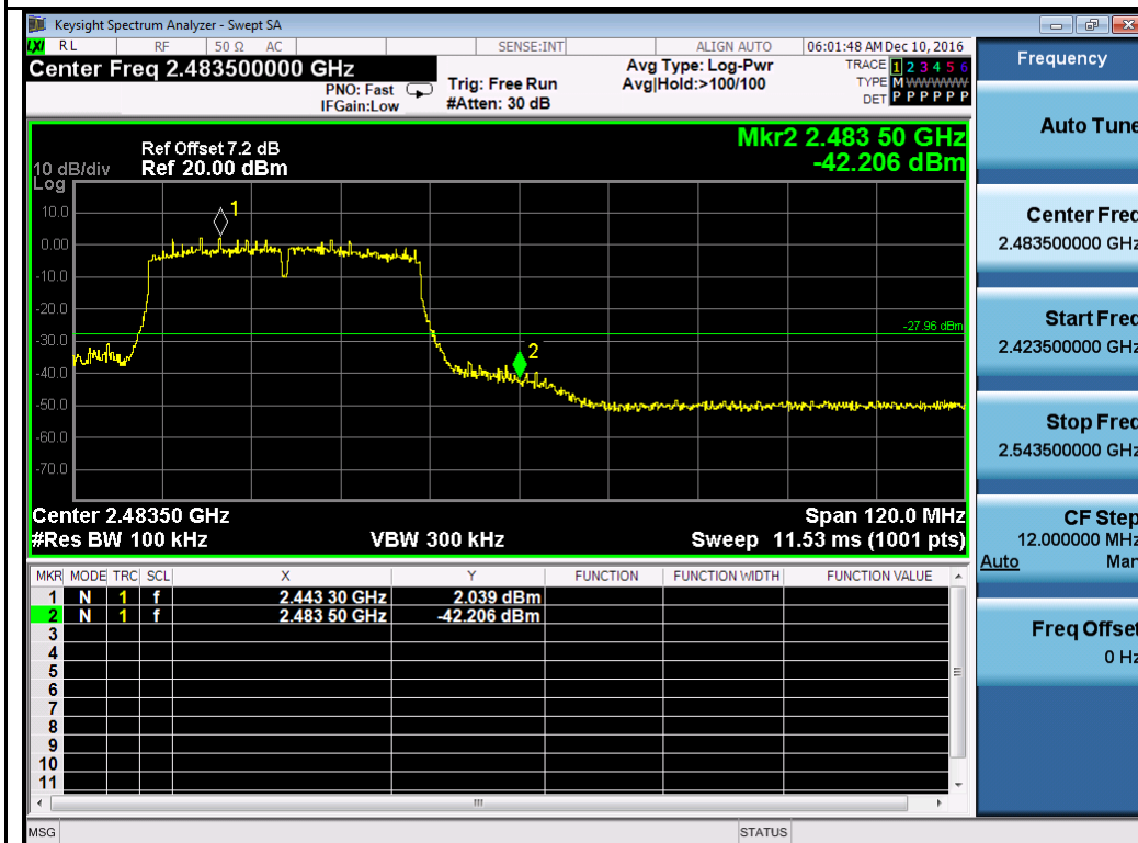
802.11n-HT40-2452MHz Chain 2
