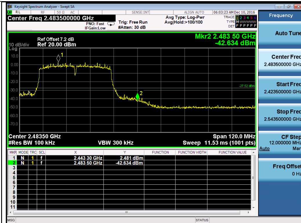
802.11n-HT40-2452MHz Chain 1
