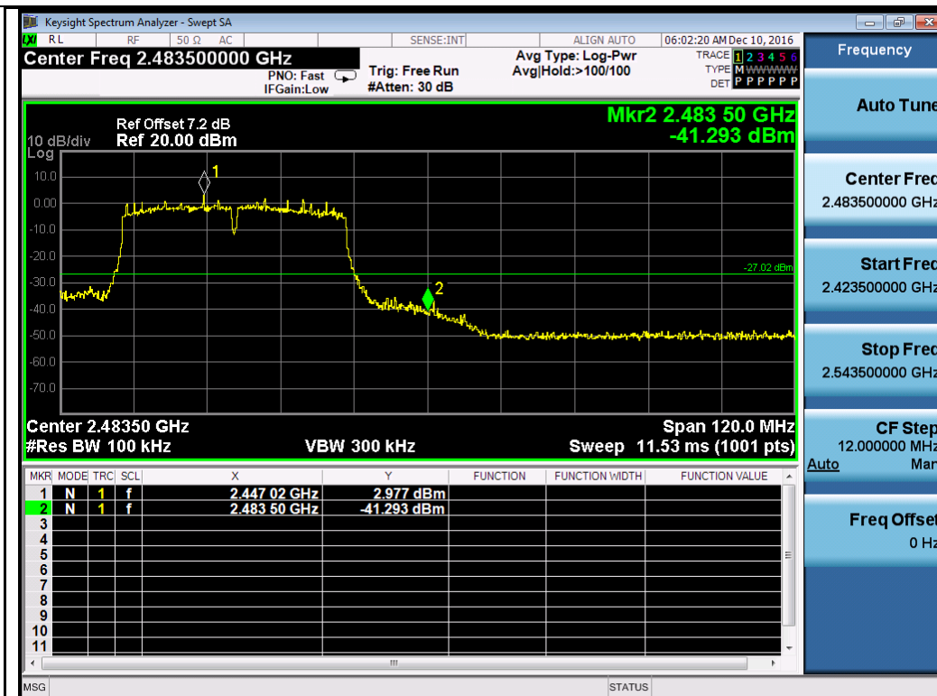
802.11n-HT40-2452MHz Chain 3
