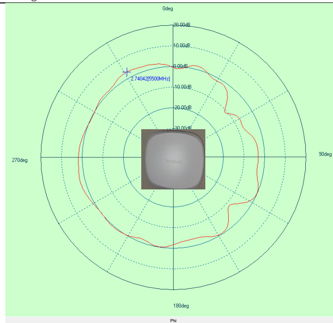
Antenna 3, dual band (2.4 and 5 GHz) horizontal Max gain 2.7 dBi at 5.5 GHz UNII-2 band
