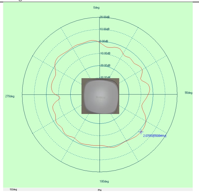
Antennas 4, 5/6 GHz vertical Max gain 2.1 dBi at 5.5 GHz UNII-2 band
