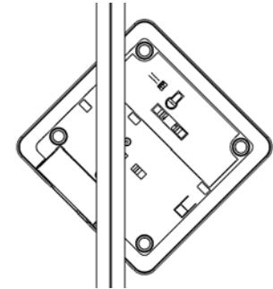
Figure 8. Attaching the integrated bracket to the T-bar
