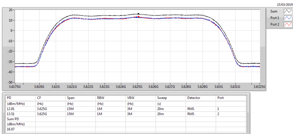
Band 48_LTE_10MHz_Nss1,QPSK_2TX 3625MHz_QPSK_RB 50,#RB 0
