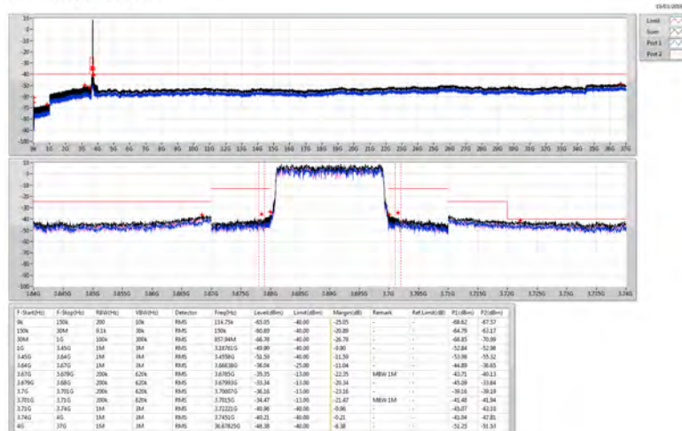
Band 48 LTE 20MHz Nss1,64QAM 2TX 3690MHz 64QAM RB 100, #RB 0
