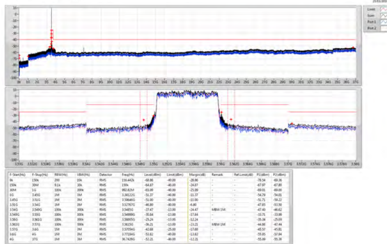
Band 48 LTE 10MHz Nss1.16QAM 2TX 3555MHz 16QAM RB 50, #RB 0
