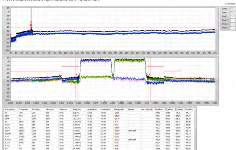
Band 48_LTE_20MHz+20MHz_Nss1,64QAM_4TX P#3560MHz.#3690MHz_64QAM_RB 100.#RB 0+RB 100.#RB 0
