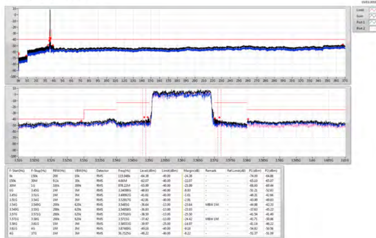
Band 48 LTE 20MHz Nss1,16QAM 2TX 3625MHz 16QAM_RB 100, #RB 0
