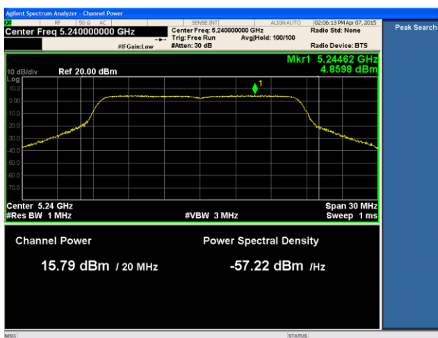
21dBi ANT-PSD-802.11a-5240M-chain1
