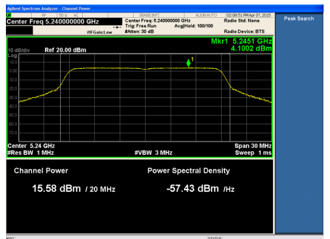
14dBi ANT-PSD-802.11n-HT20-5240M-chain2
