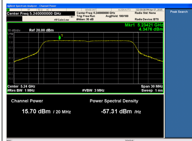
24dBi ANT-PSD-802.11n-HT20-5240M-chain1
