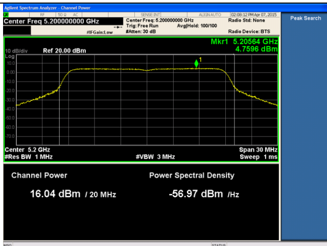
14dBi ANT-PSD-802.11n-HT20-5200M-chain1
