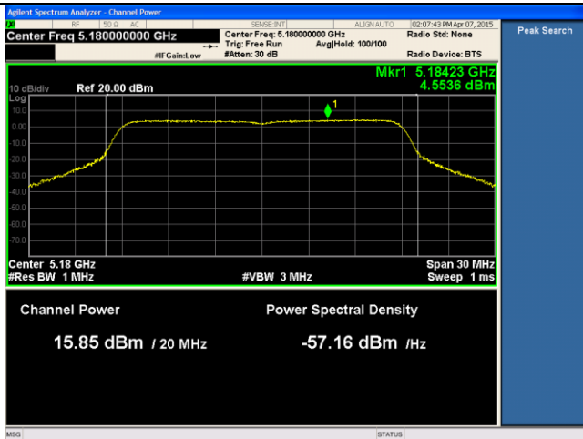
14dBi ANT-PSD-802.11n-HT20-5180M-chain1
