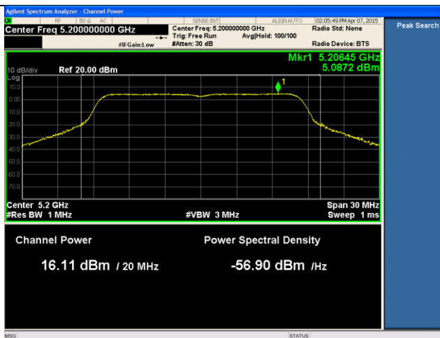
21dBi ANT-PSD-802.11a-5200M-chain1
