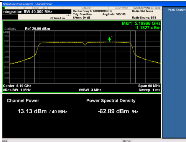
14dBi ANT-PSD-802.11n-HT40-5190M-chain1
