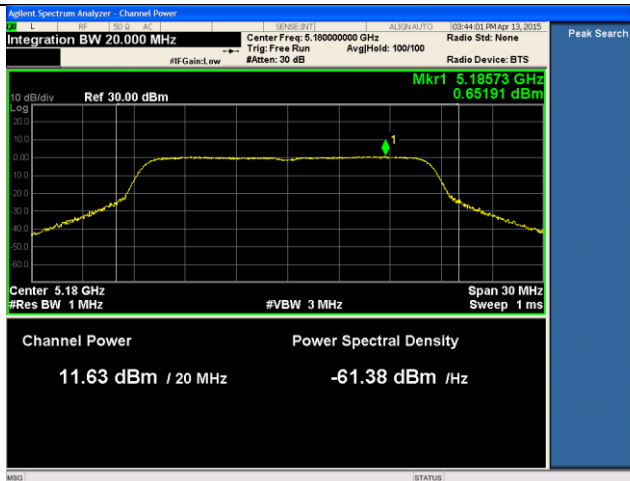
21dBi ANT-PSD-802.11a-5180M-chain1
