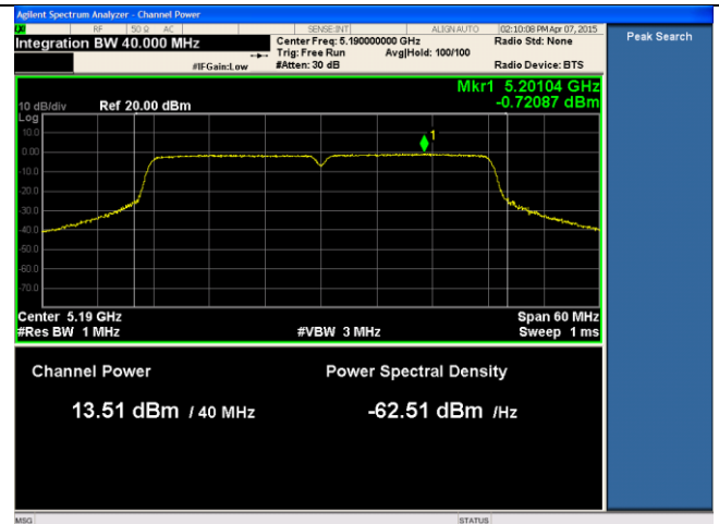
14dBi ANT-PSD-802.11n-HT40-5190M-chain2
