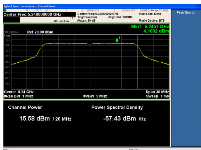
24dBi ANT-PSD-802.11n-HT20-5240M-chain2
