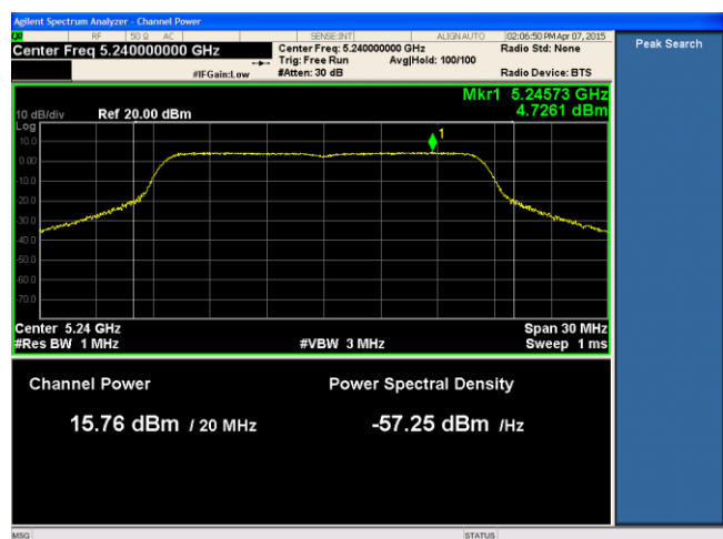
24dBi ANT-PSD-802.11a-5240M-chain2
