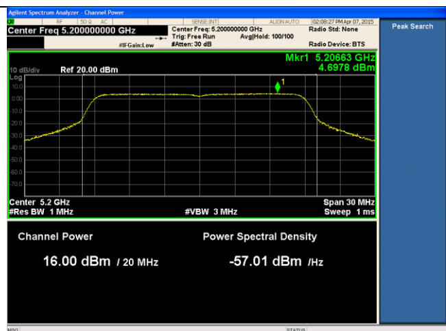
21dBi ANT-PSD-802.11n-HT20-5200M-chain2
