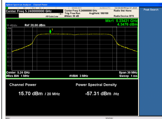
21dBi ANT-PSD-802.11n-HT20-5240M-chain1
