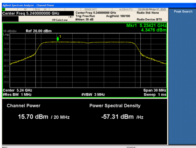
14dBi ANT-PSD-802.11n-HT20-5240M-chain1
