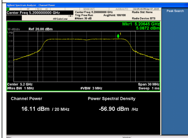
24dBi ANT-PSD-802.11a-5200M-chain1
