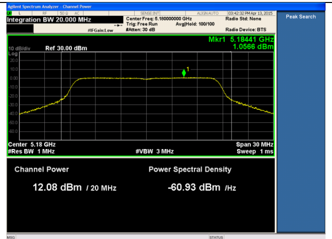
21dBi ANT-PSD-802.11a-5180M-chain2
