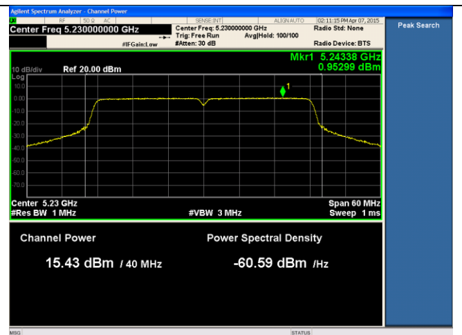
24dBi ANT-PSD-802.11n-HT40-5230M-chain2
