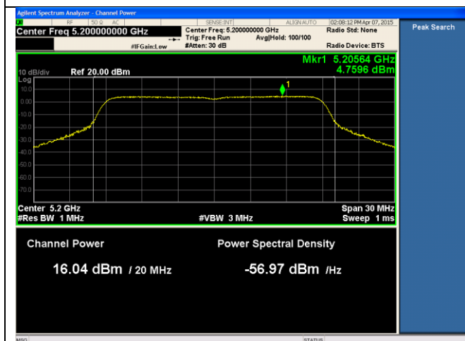
21dBi ANT-PSD-802.11n-HT20-5200M-chain1
