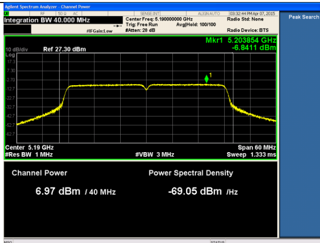
24dBi ANT-PSD-802.11n-HT40-5190M-chain1
