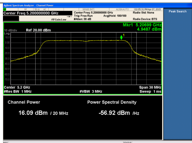
24dBi ANT-PSD-802.11a-5200M-chain2
