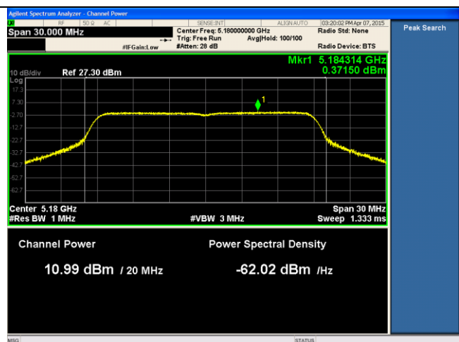
24dBi ANT-PSD-802.11n-HT20-5180M-chain2
