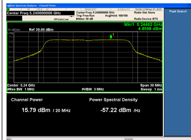
24dBi ANT-PSD-802.11a-5240M-chain1
