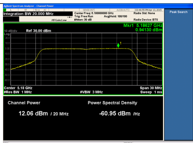
21dBi ANT-PSD-802.11n-HT20-5180M-chain2
