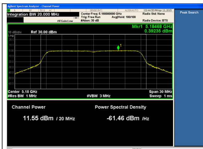
21dBi ANT-PSD-802.11n-HT20-5180M-chain1
