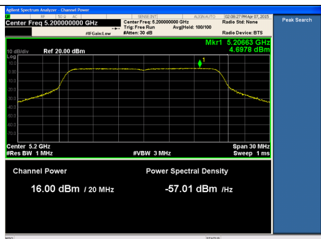
24dBi ANT-PSD-802.11n-HT20-5200M-chain2
