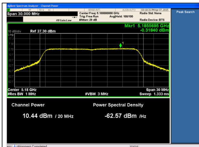
24dBi ANT-PSD-802.11n-HT20-5180M-chain1
