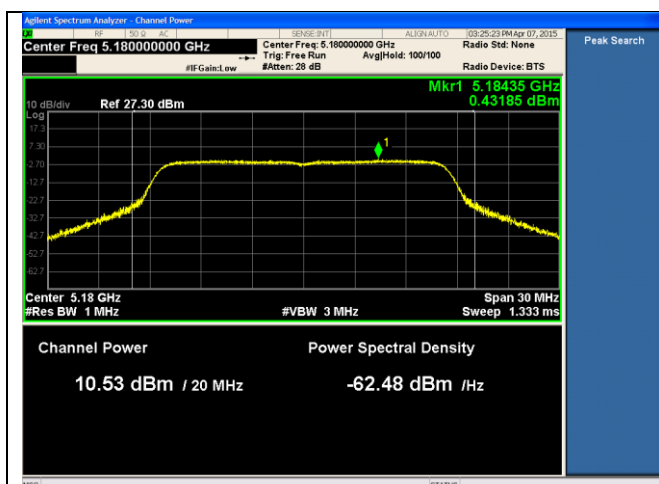
24dBi ANT-PSD-802.11a-5180M-chain1
