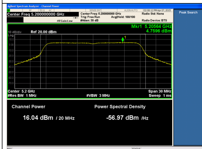
24dBi ANT-PSD-802.11n-HT20-5200M-chain1
