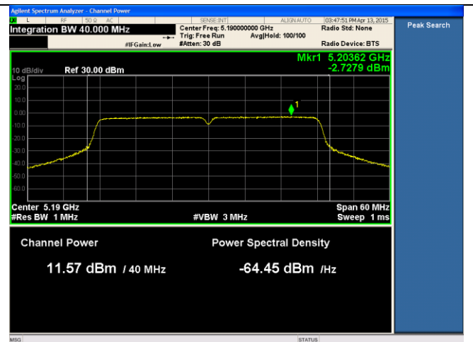
24dBi ANT-PSD-802.11n-HT40-5190M-chain2
