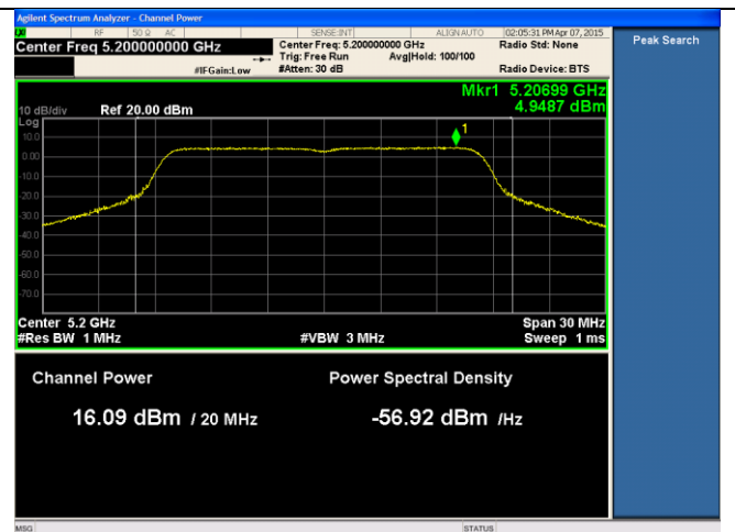
21dBi ANT-PSD-802.11a-5200M-chain2
