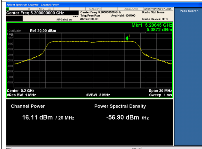
14dB ANT-PSD-802.11a-5200M-chain1
