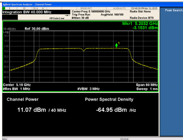
24dBi ANT-PSD-802.11n-HT40-5190M-chain1
