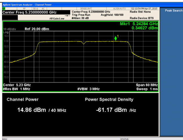
14dBi ANT-PSD-802.11n-HT40-5230M-chain1
