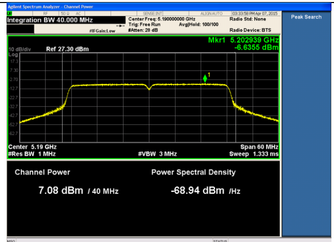
24dBi ANT-PSD-802.11n-HT40-5190M-chain2
