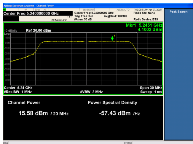
21dBi ANT-PSD-802.11n-HT20-5240M-chain2
