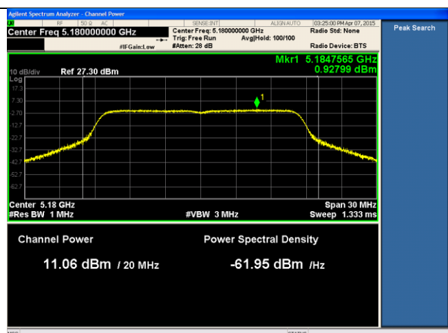
24dBi ANT-PSD-802.11a-5180M-chain2
