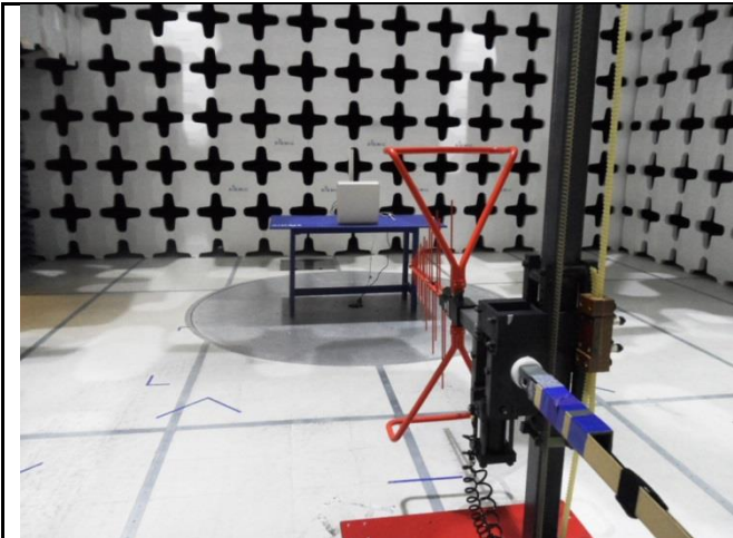
24dBi ANT Radiated Emissions (<1GHz) – Front View
