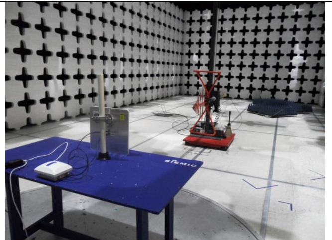
24dBi ANT Radiated Emissions (<1GHz) – Rear View
