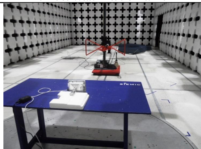
13dBi ANT Radiated Emissions (<1GHz) – Rear View
