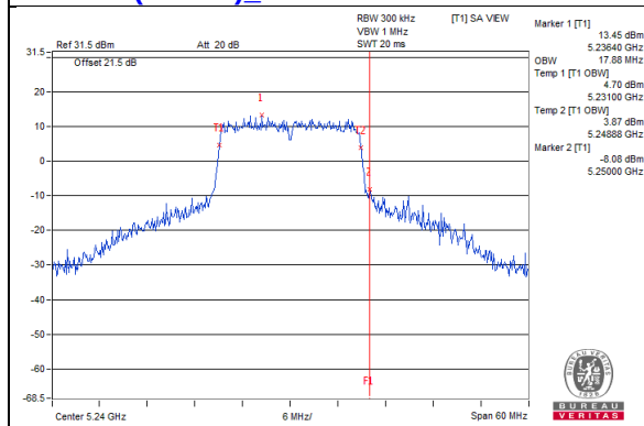
802.11ac(VHT20)_Chain0 / CH48
