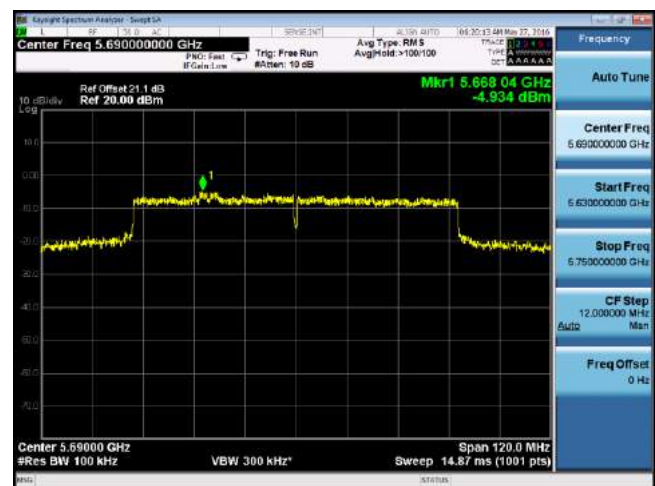
PSD-802.11ac-CROSSBAND-5690M-chain1
