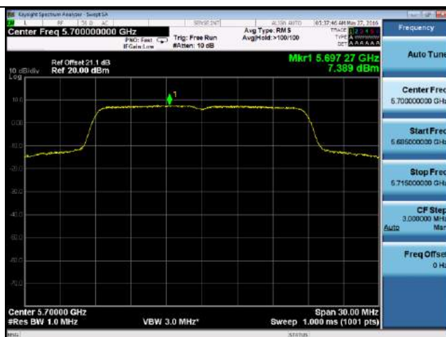
PSD-802.11n-20M-5700M-chain0
