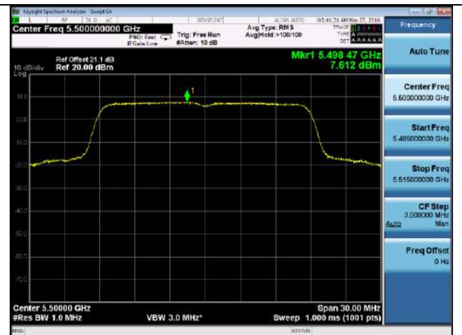
PSD-802.11n-20M-5500M-chain1
