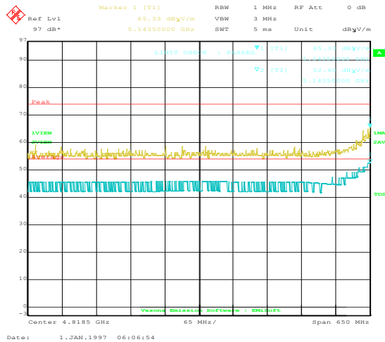
802.11ac-VHT80 5290M(4500-5150MHz)
