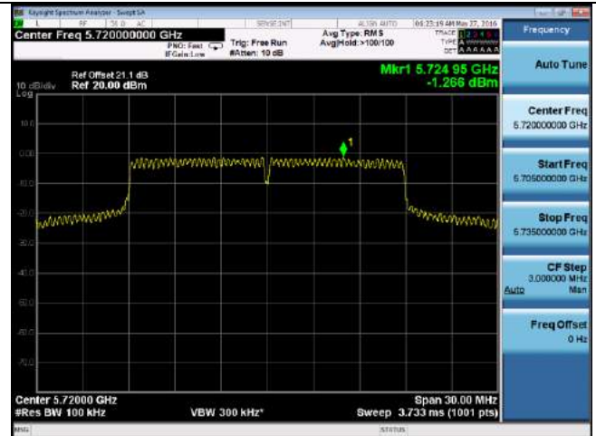
PSD-802.11n-20M-CROSSBAND-5720M-chain1
