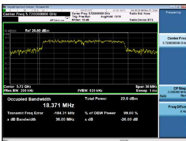
26dB BW -802.11a CROSSBAND 5720MHz
