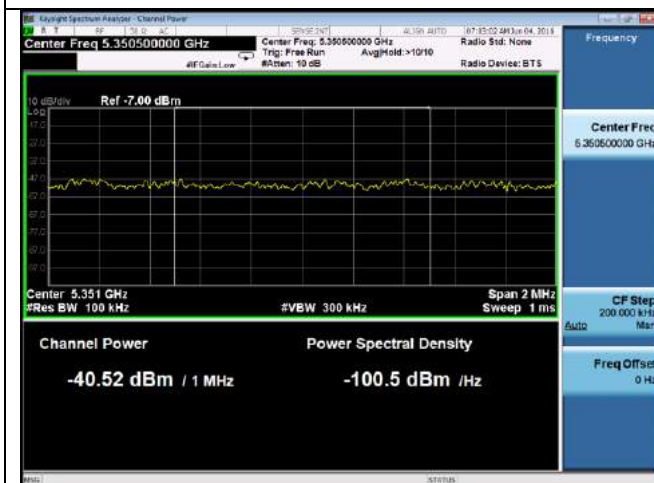
Band Edge -802.11n-20M -5320M-chain0
