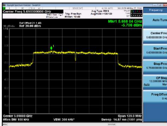
PSD-802.11ac-CROSSBAND-5690M-chain0
