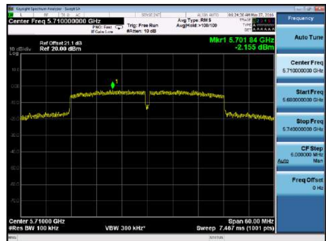
PSD-802.11n-40M-CROSSBAND-5710M-chain1
