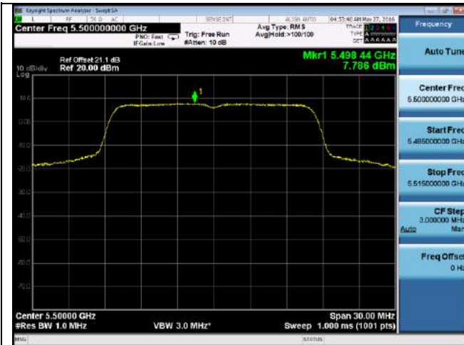
PSD-802.11a-5500M-chain0
