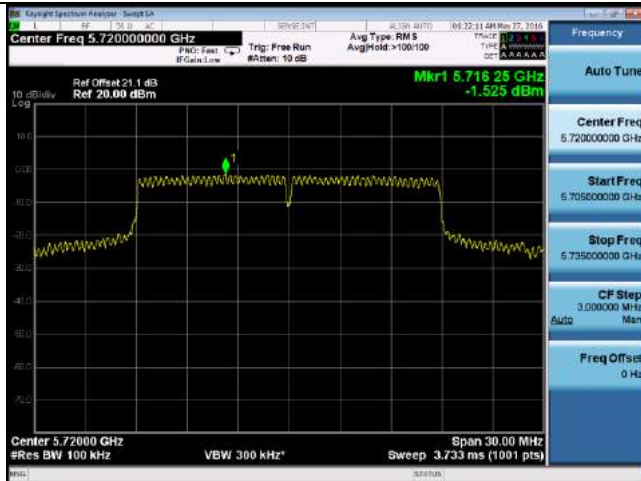
PSD-802.11n-20M-CROSSBAND-5720M-chain0
