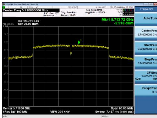
PSD-802.11n-40M-CROSSBAND-5710M-chain0
