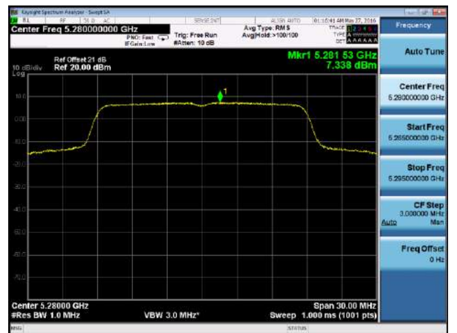
PSD-802.11n-20M-5280M-chain1
