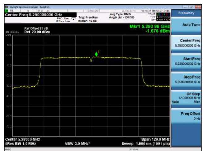
PSD-802.11ac-80M-5290M-chain1
