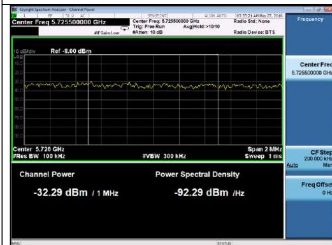
Band Edge -802.11a-5700M-chain0
