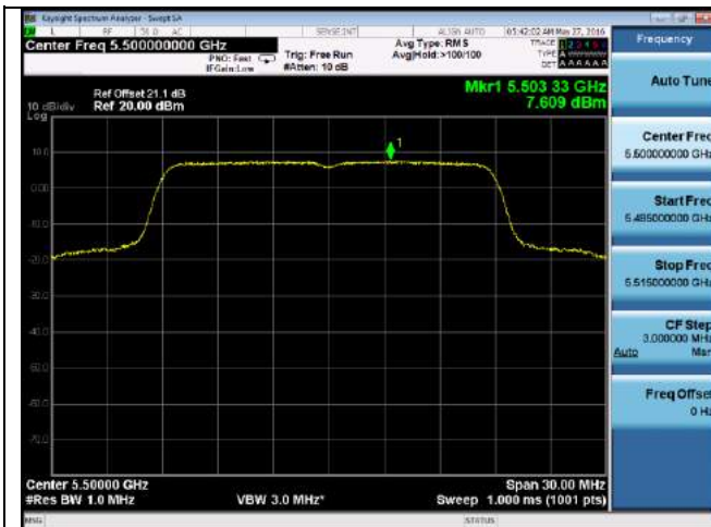
PSD-802.11n-20M-5500M-chain0
