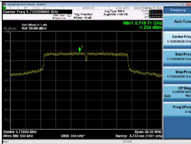
PSD-802.11a-CROSSBAND-5720M-chain0
