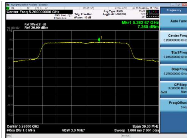
PSD-802.11n-20M-5260M-chain0
