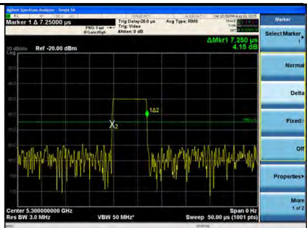
Radar Calibration - Type 3 (Single Burst)
