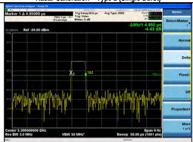
Radar Calibration - Type 2 (Single Burst)
