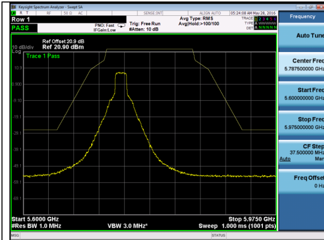
Emission Mask -802.11a-5745M-chain0
