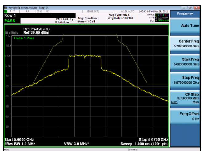
Emission Mask -802.11ac-80M-5775M-chain1
