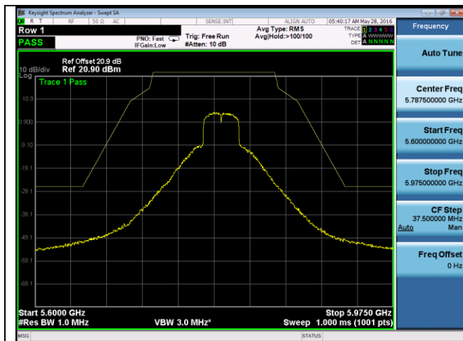
Emission Mask -802.11n-40M-5795M-chain0
