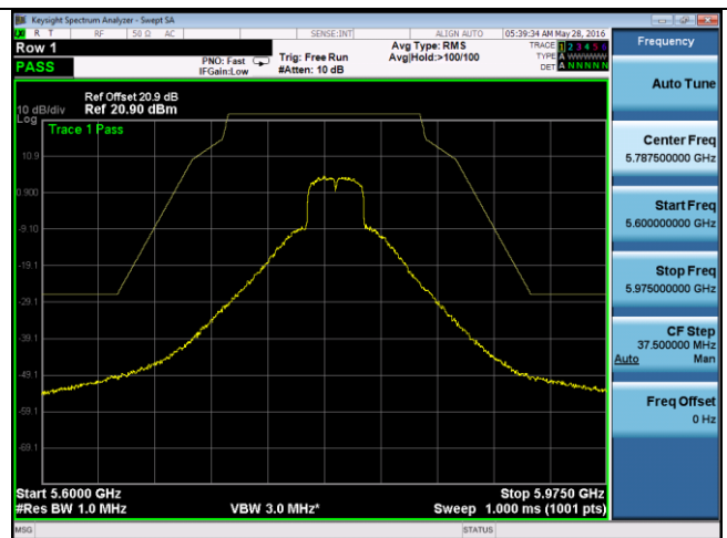
Emission Mask -802.11n-40M-5795M-chain1
