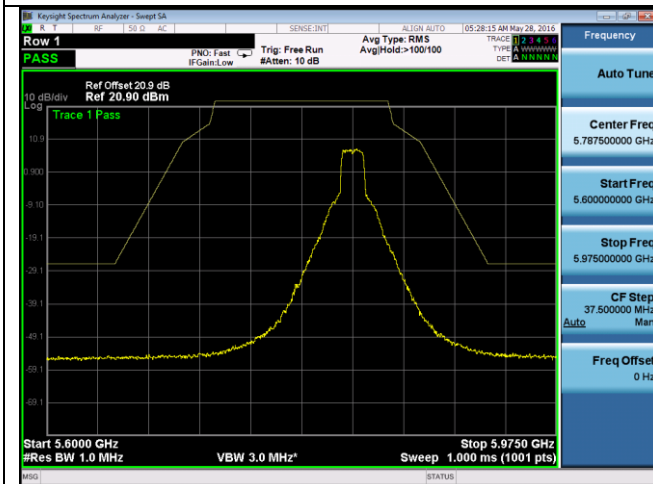
Emission Mask -802.11a-5785M-chain0
