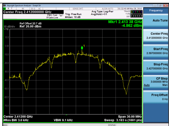
PSD-2.4G-802.11b Low-chain1
