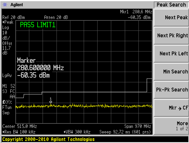
802.11n 40 mode, 5180 MHz, Chain J6 3
