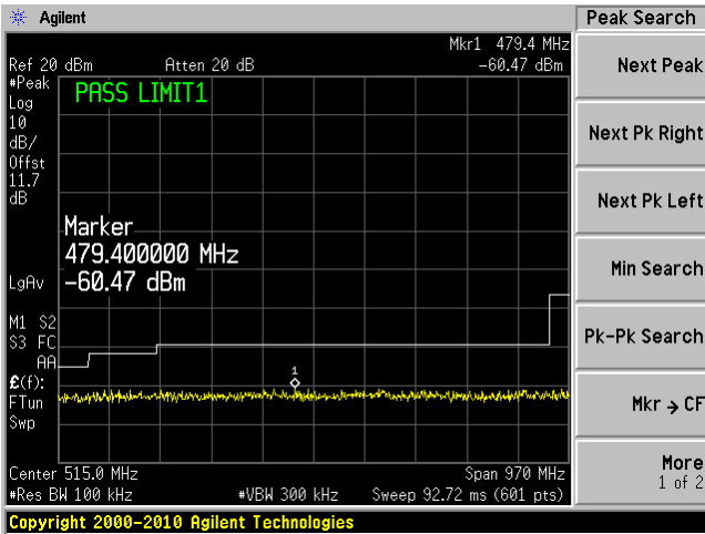
802.11n 40 mode, 5240 MHz, Chain J8 3
