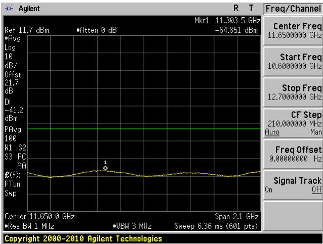
802.11n 20 mode, 5240 MHz, Chain J10 24
