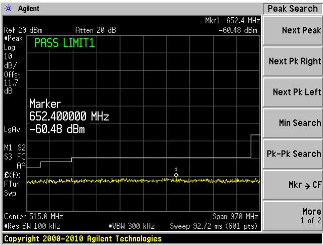
802.11n 40 mode, 5240 MHz, Chain J6 1
