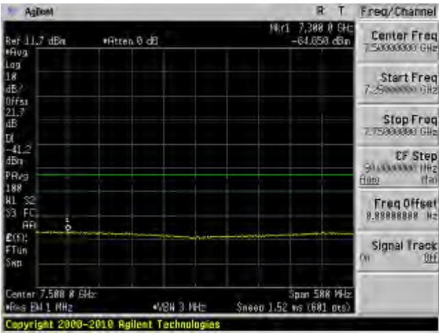
802.11a mode, 5240 MHz, Chain J8 18
