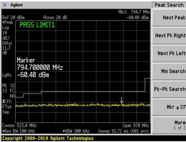
802.11n 40 mode, 5240 MHz, Chain J10 3
