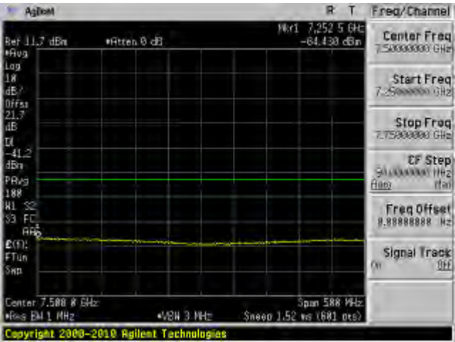
802.11n 20 mode, 5180 MHz, Chain J8 18
