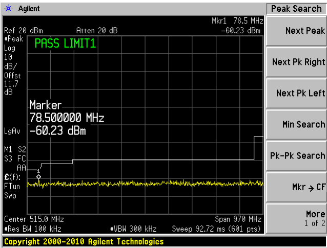
802.11n 20 mode, 5180 MHz, Chain J8 1
