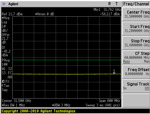
802.11n 20 mode, 5180 MHz, Chain J6 29
