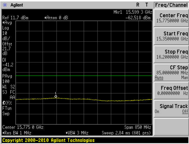
802.11n 40 mode, 5180 MHz, Chain J6 27
