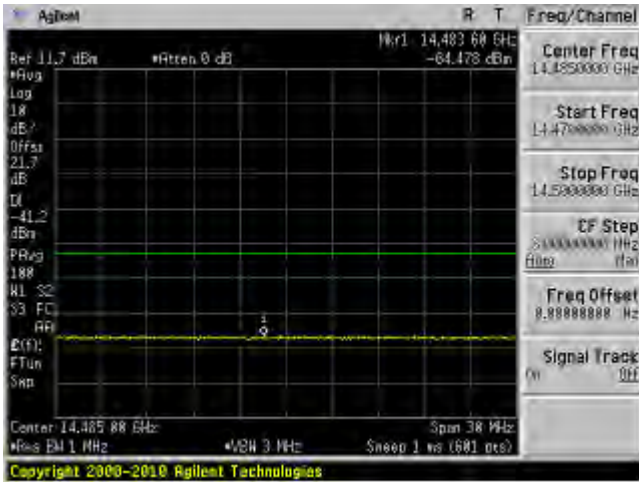
802.11n 40 mode, 5240 MHz, Chain J6 24
