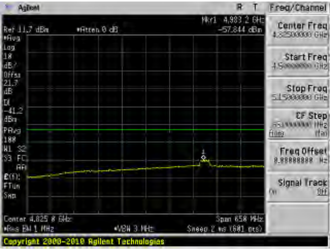
802.11n 20 mode, 5200 MHz, Chain J10 16
