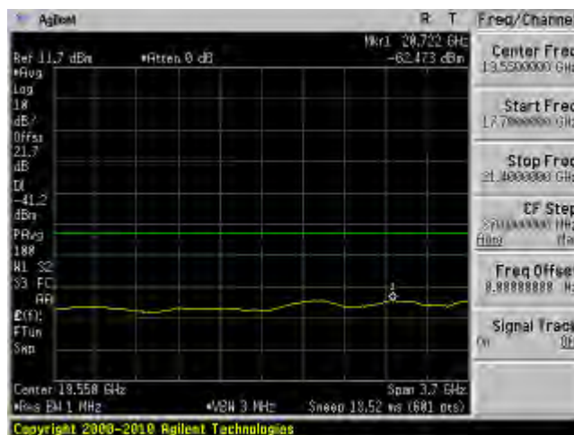
802.11a mode, 5240 MHz, Chain J8 26
