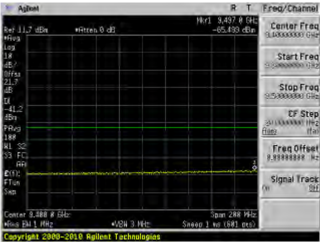
802.11a mode, 5240 MHz, Chain J8 23
