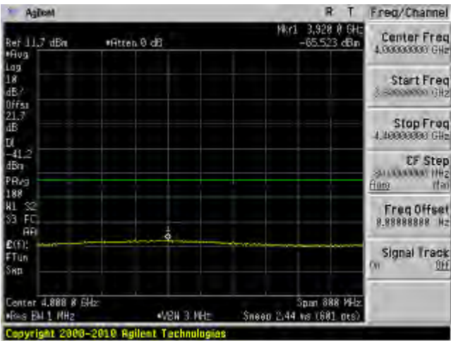
802.11a mode, 5240 MHz, Chain J8 15
