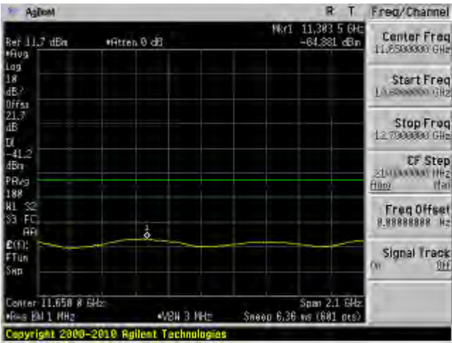
802.11n 40 mode, 5180 MHz, Chain J10 24
