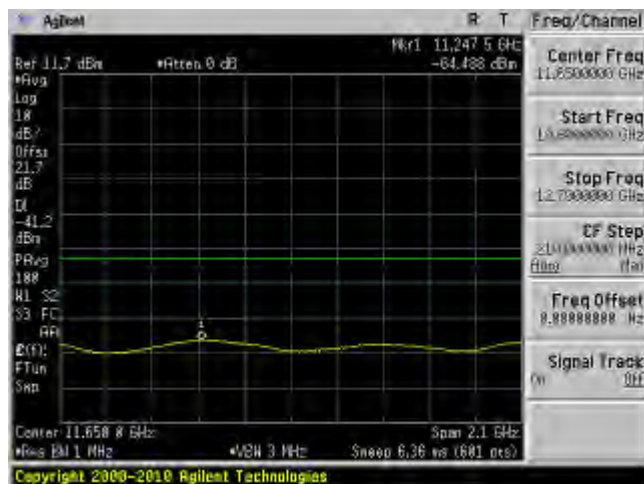
802.11a mode, 5240 MHz, Chain J10 24
