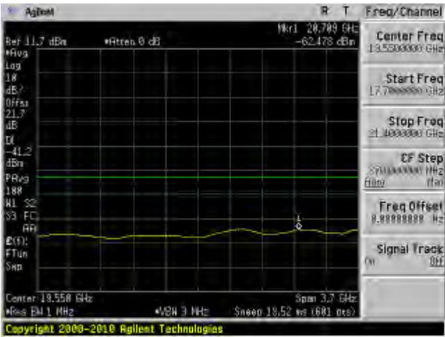
802.11a mode, 5240 MHz, Chain J10 28
