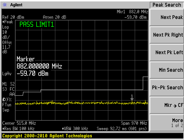
802.11a mode, 5240 MHz, Chain J6 3
