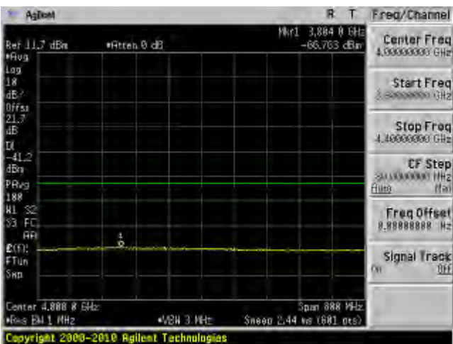
802.11n 40 mode, 5180 MHz, Chain J6 15
