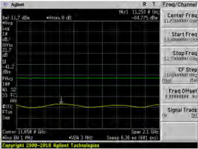
802.11n 20 mode, 5200 MHz, Chain J10 24
