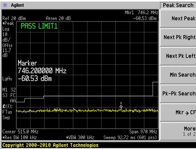
802.11n 20 mode, 5200 MHz,Chain J6 3
