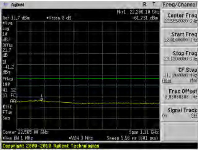
802.11n 40 mode, 5180 MHz, Chain J10 27
