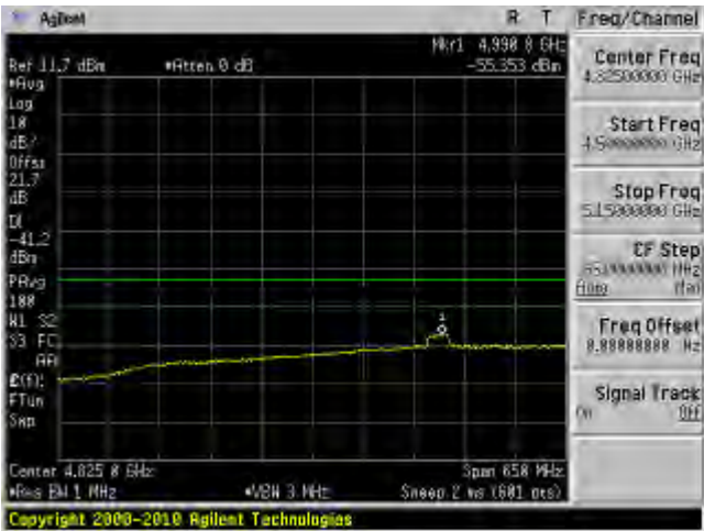
802.11a mode, 5240 MHz, Chain J10 16
