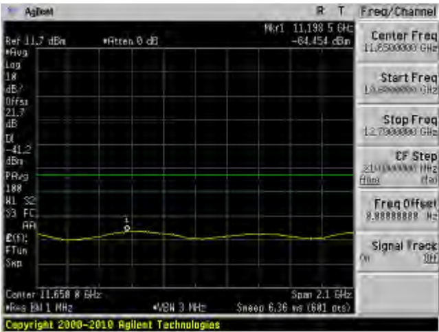
802.11a mode, 5240 MHz, Chain J8 24
