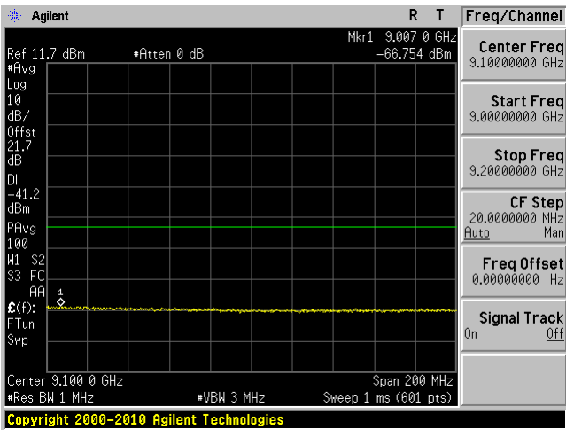
802.11a mode, 5240 MHz, Chain J8 20
