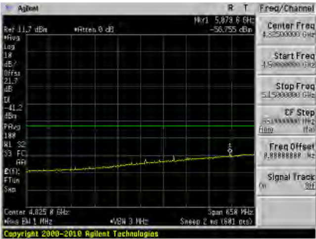
802.11a mode, 5200 MHz, Chain J8 16
