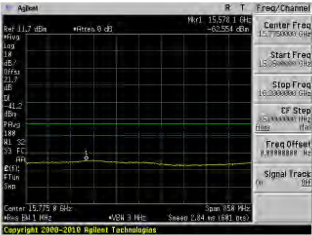
802.11n 20 mode, 5200 MHz, Chain J8 27
