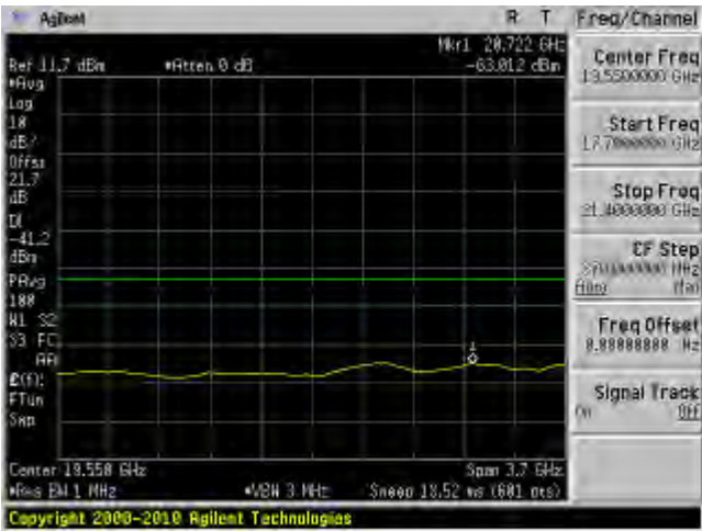
802.11n 20 mode, 5200 MHz, Chain J10 28
