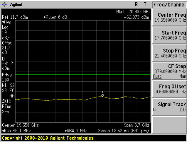
802.11n 40 mode, 5180 MHz, Chain J6 28
