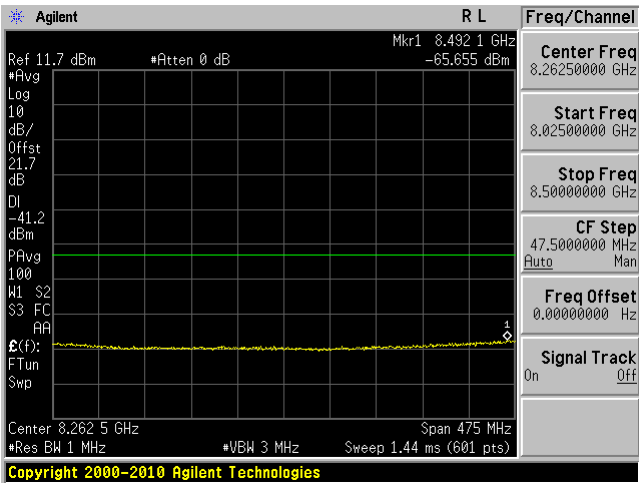
802.11n 20 mode, 5200 MHz, Chain J10 19
