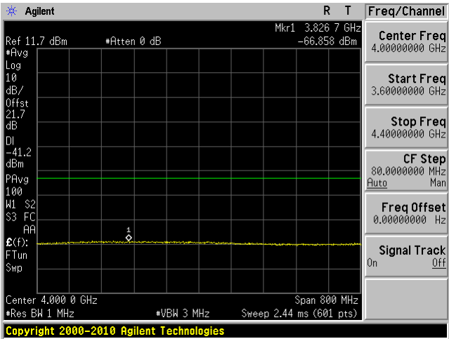
802.11n 20 mode, 5240 MHz, Chain J10 15
