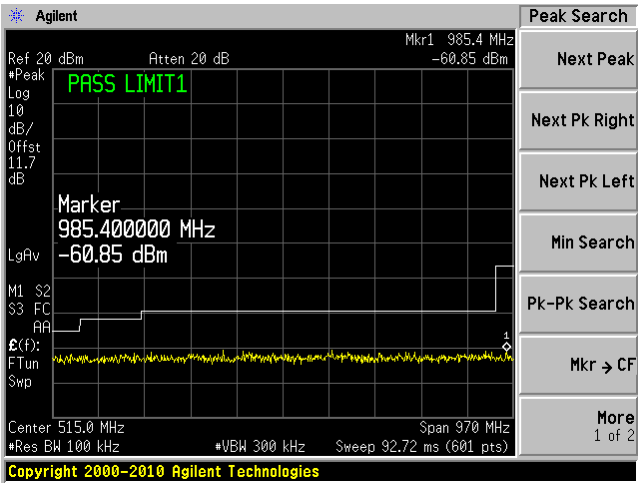
802.11n 20 mode, 5240 MHz, Chain J6 3
