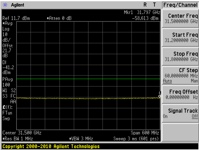
802.11n 20 mode, 5240 MHz, Chain J10 29
