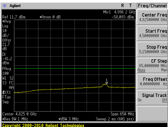
802.11n 20 mode, 5240 MHz, Chain J10 16
