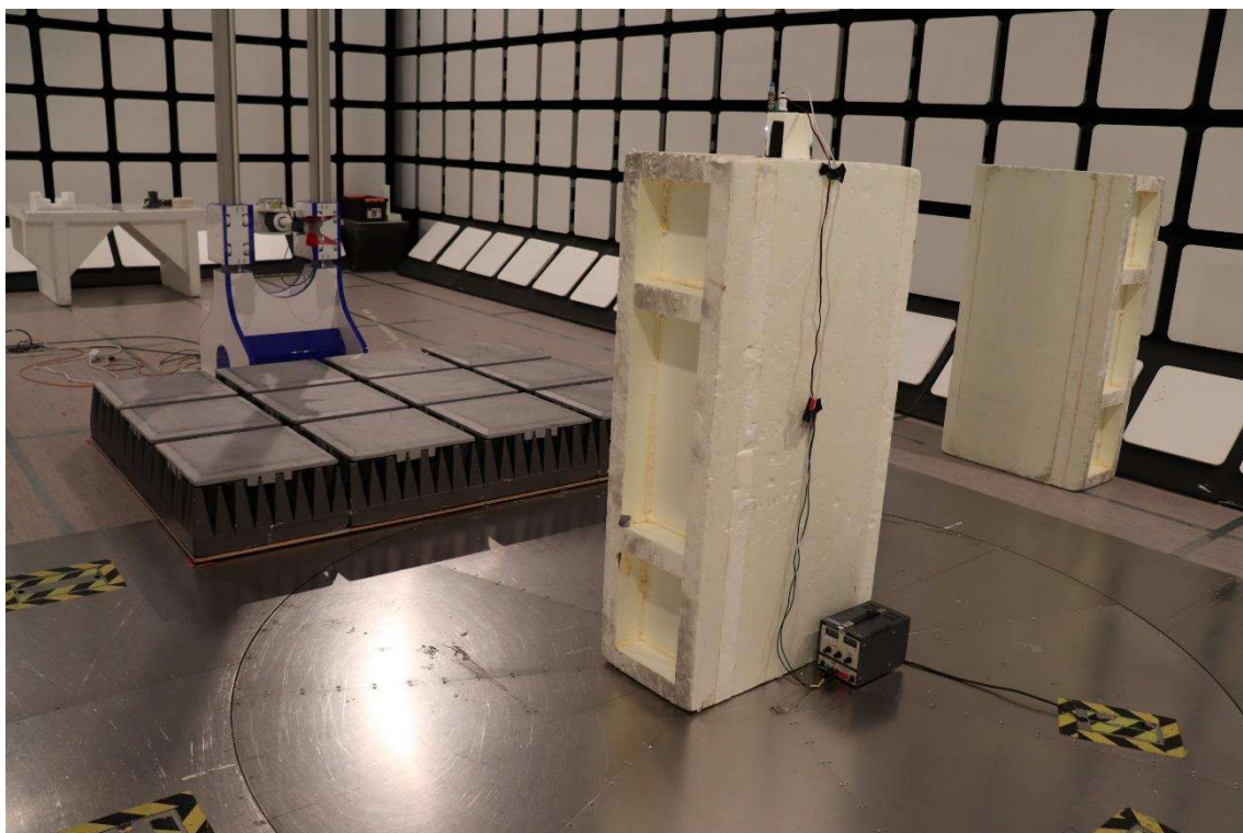
Photograph 3. Test Setup for Radiated Emissions 1 – 10 GHz
