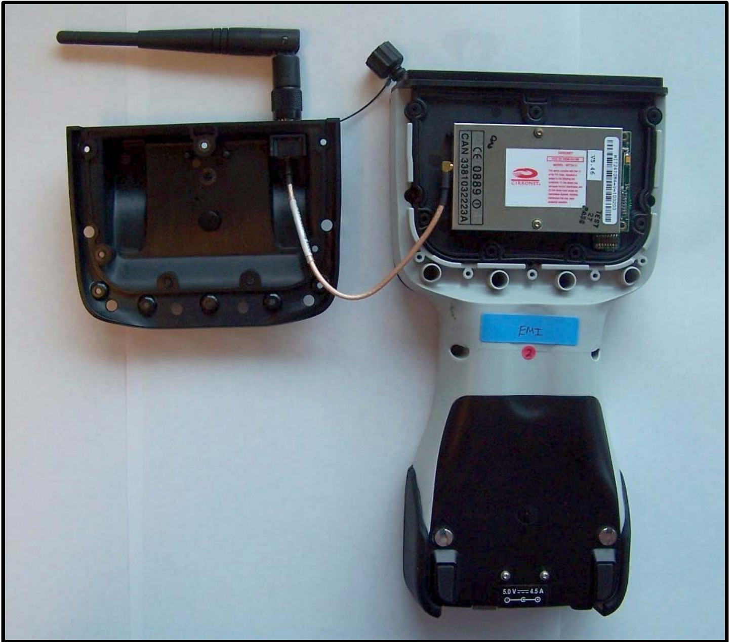
Cirronet Internal View
