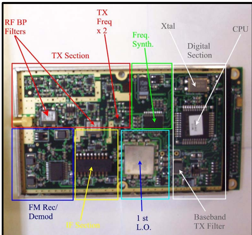
Cirronet Internal Close-up and Internal Block
