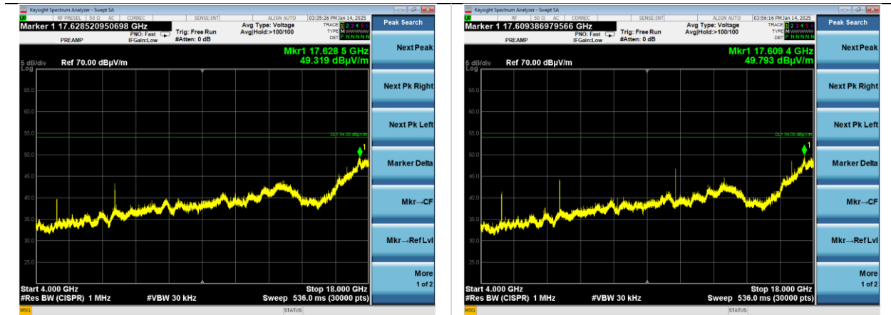
4-18 GHz Horizontal Polarity Ch 19 1M Power Index 20 | EUT Flat
