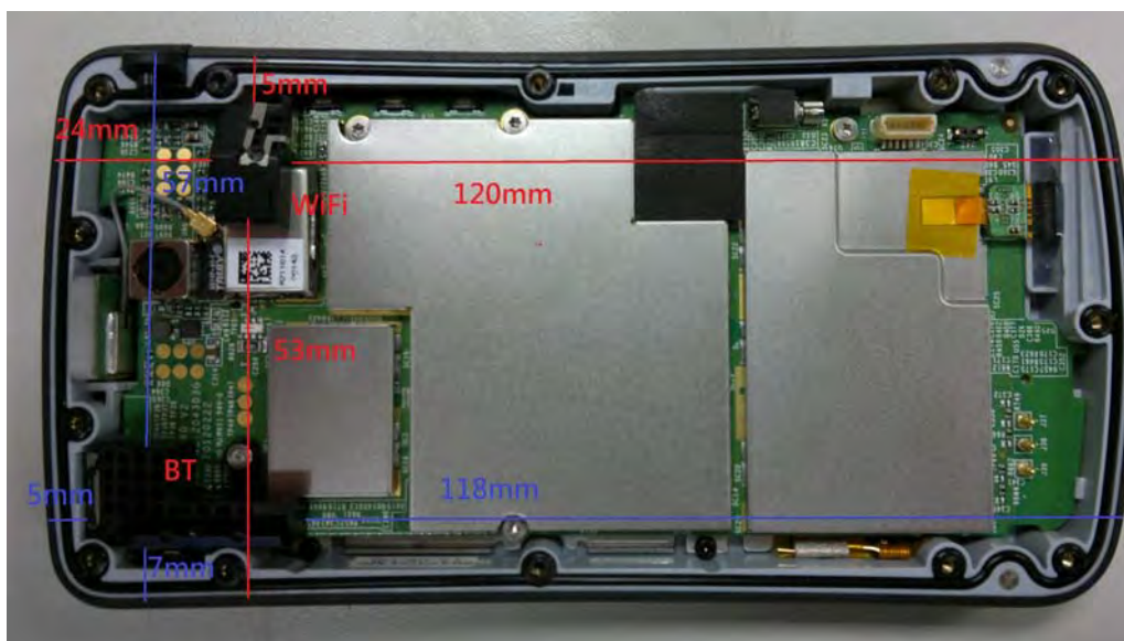
Fig.11 Antenna position of EUT
