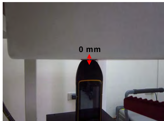
Fig.7 EUT top to flat phantom
