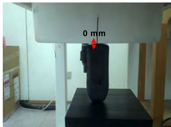
Fig.8 EUT bottom to flat phantom
