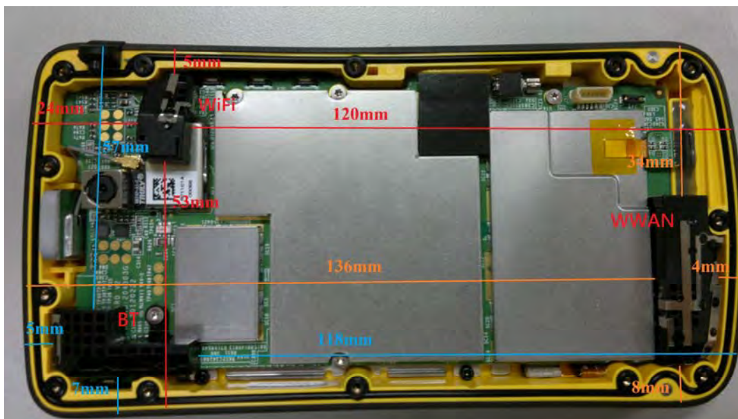
Fig.17 Antenna position of EUT
