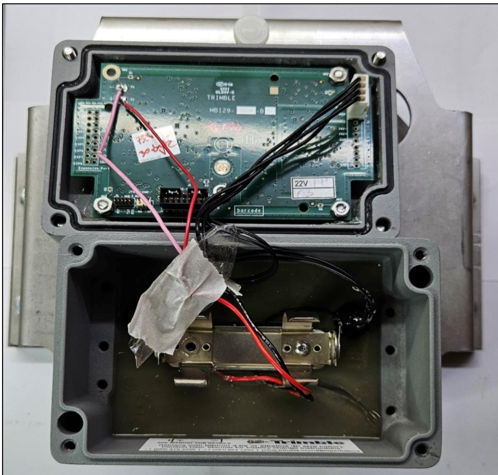
EUT Bottom View
