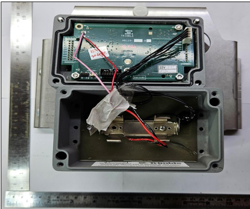
EUT Dimension View
