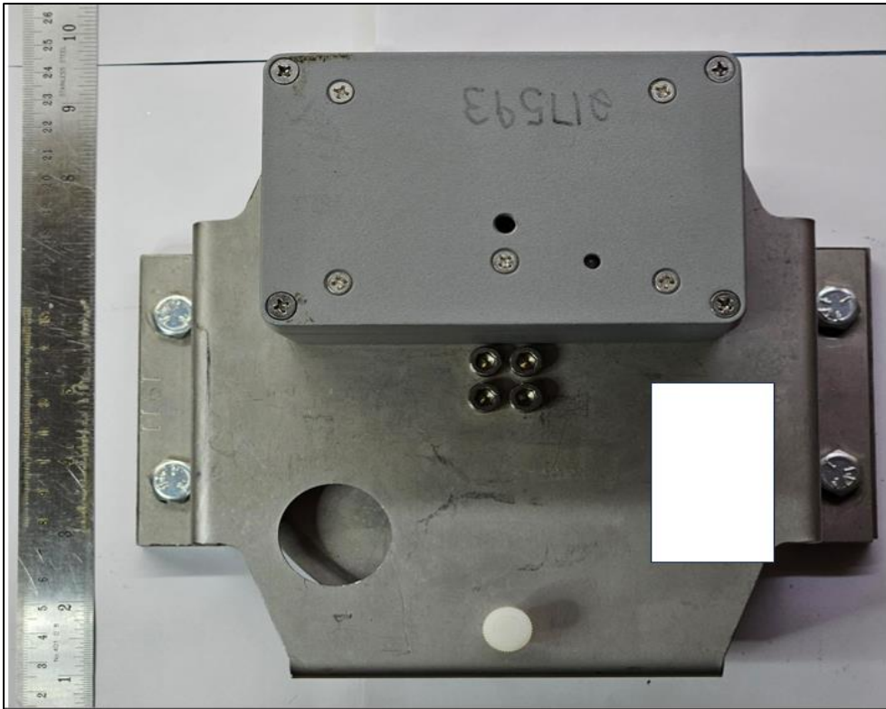
EUT Dimension View
