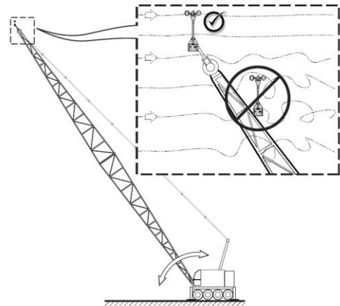
Figure 2, Wind Speed installation on crane boom
