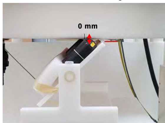
Fig.4 EUT Back side (WWAN) to flat phantom
