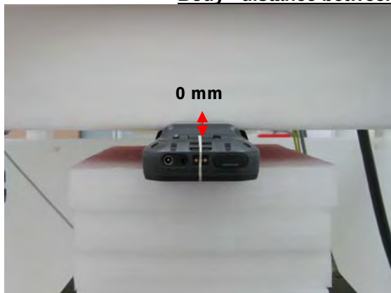
Fig.6 EUT Back side (WLAN Aux) to flat phantom
