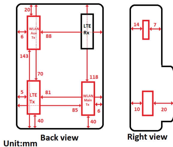
Fig.13 Antenna position of EUT (Back view & Right view )
