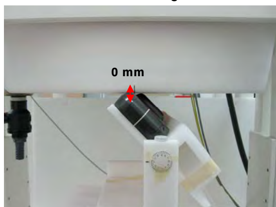
Fig.5 EUT Back side (WLAN Main) to flat phantom
