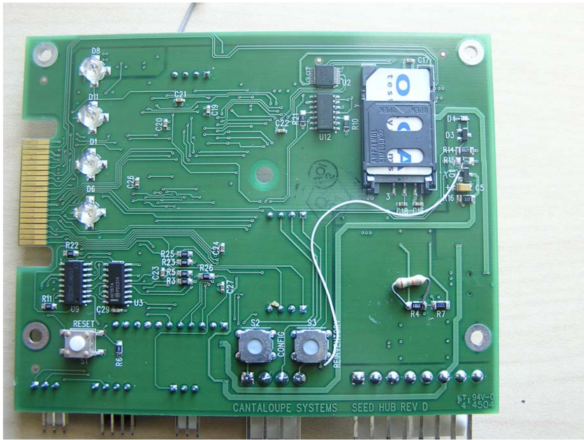
EUT – Internal Bottom View
