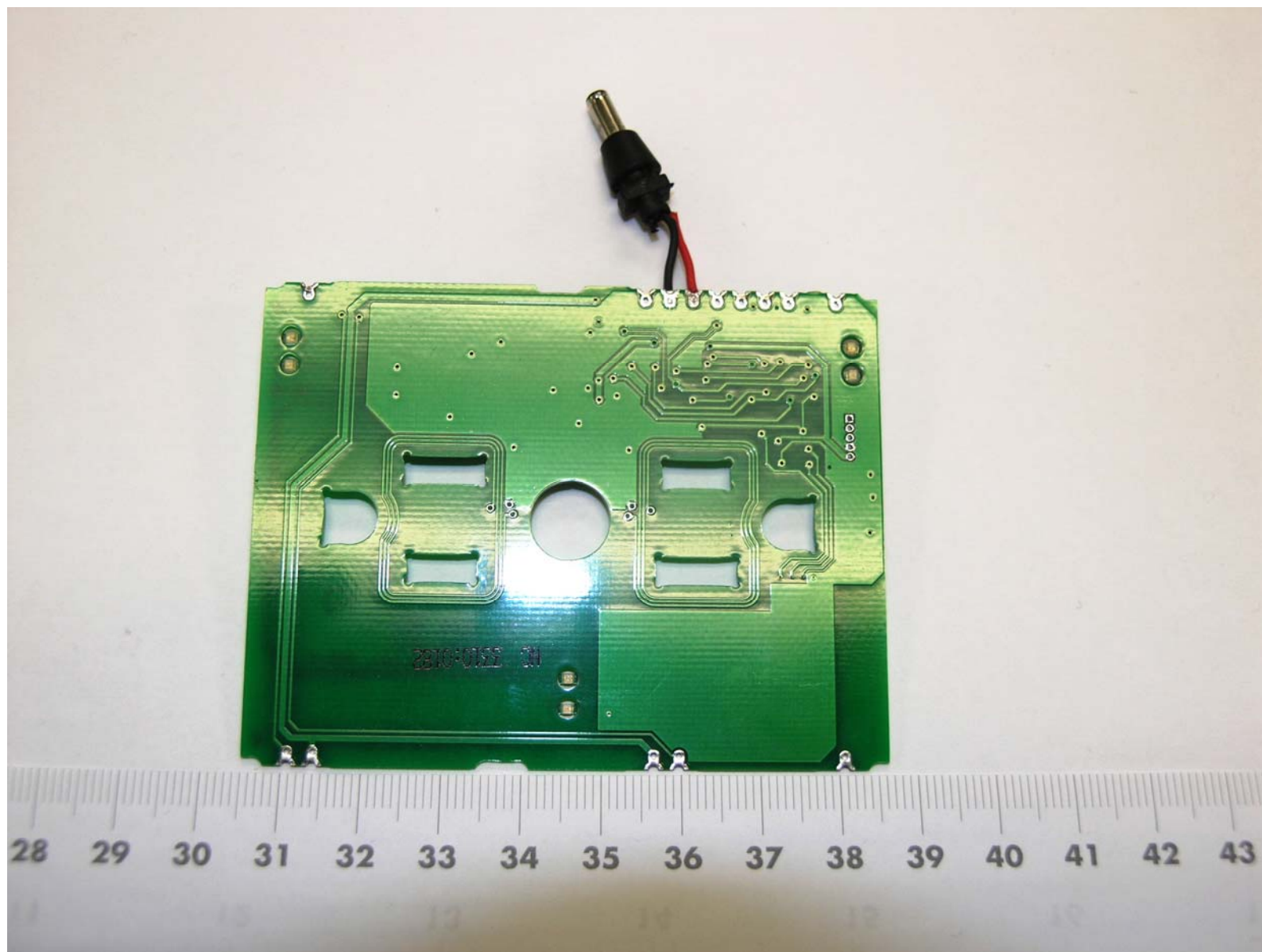
OFI, Inc. (subsidiary of 2D2C Inc.) SafePlug Outlet Control Board, Model 3064 FCC ID: S9C-3064 IC: 5850A-3064
